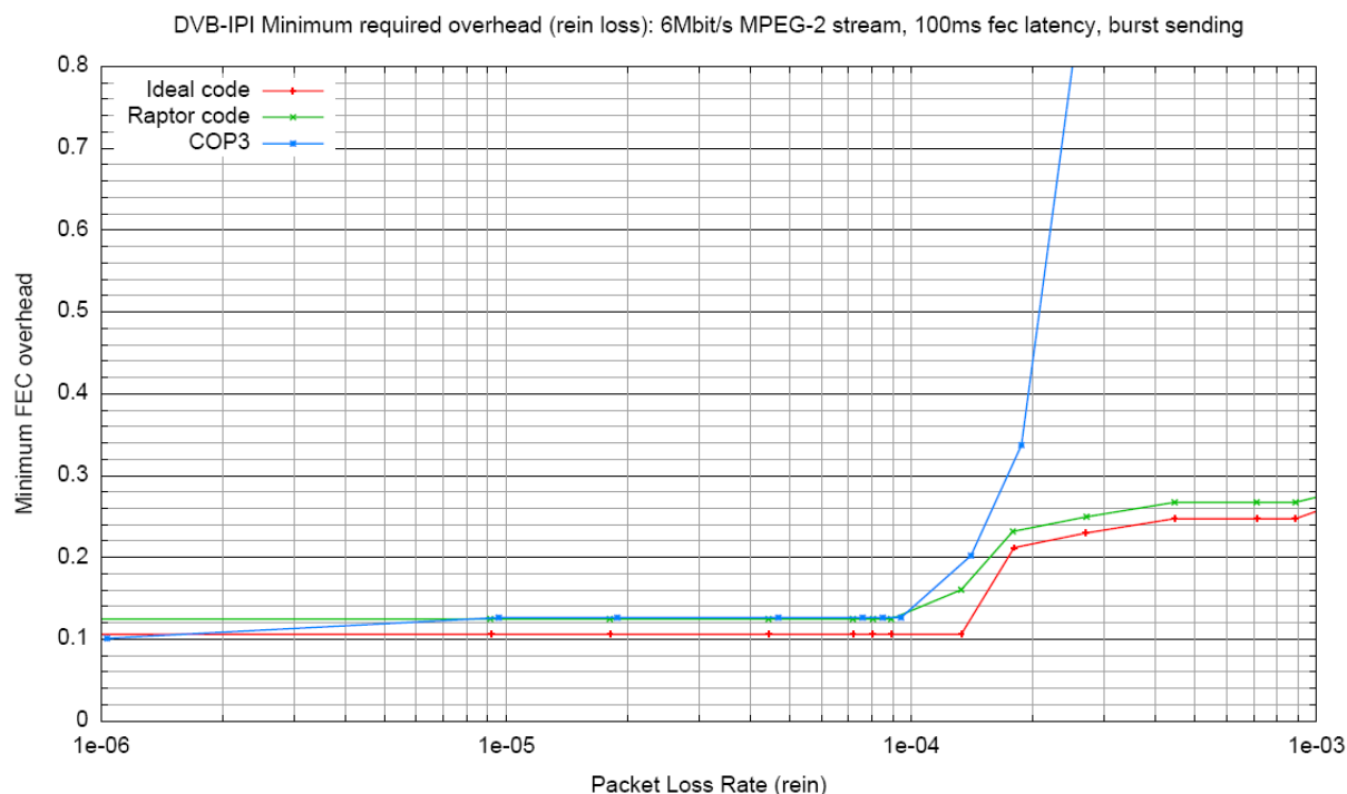
Figure 9.3.3.2.4: 6 Mbit/s MPEG-2 Transport Stream, 100 ms latency (live content), REIN loss, burst sending
