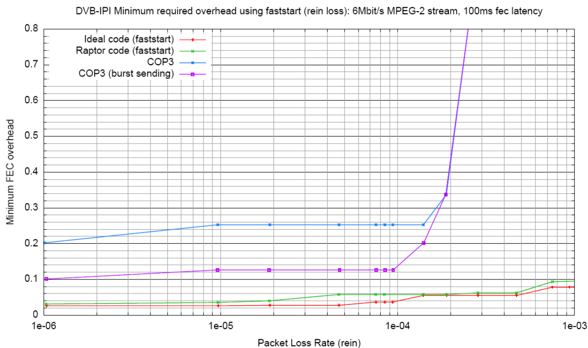
Figure 9.3.3.1.4: 6 Mbit/s MPEG-2 Transport Stream, 100 ms latency (stored/buffered content), REIN
