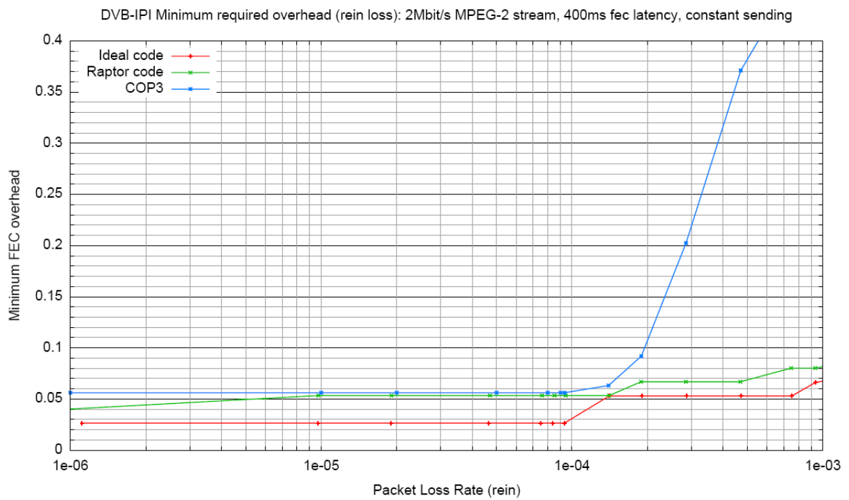
Figure 9.3.2.1.3: 2 Mbit/s MPEG-2 Transport Stream, 400 ms latency, REIN, constant sending
