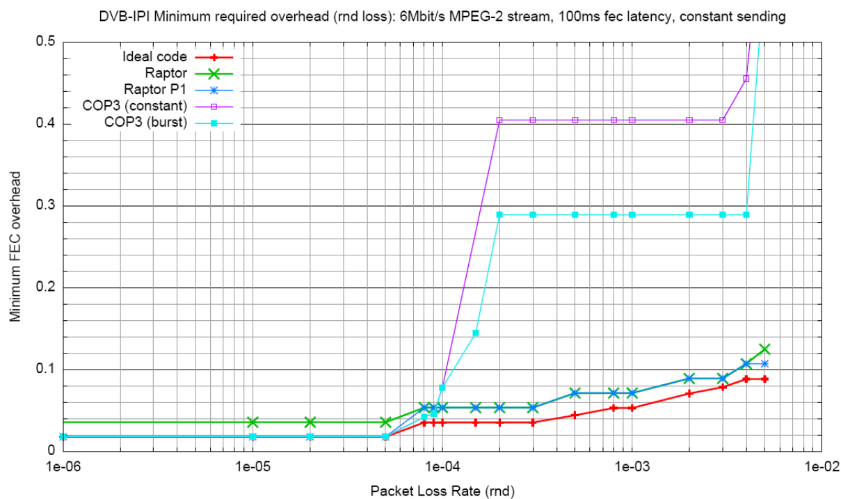
Figure 12.1.6: 6 Mbit/s MPEG-2 Transport Stream, 100 ms latency, Random Loss, constant sending
