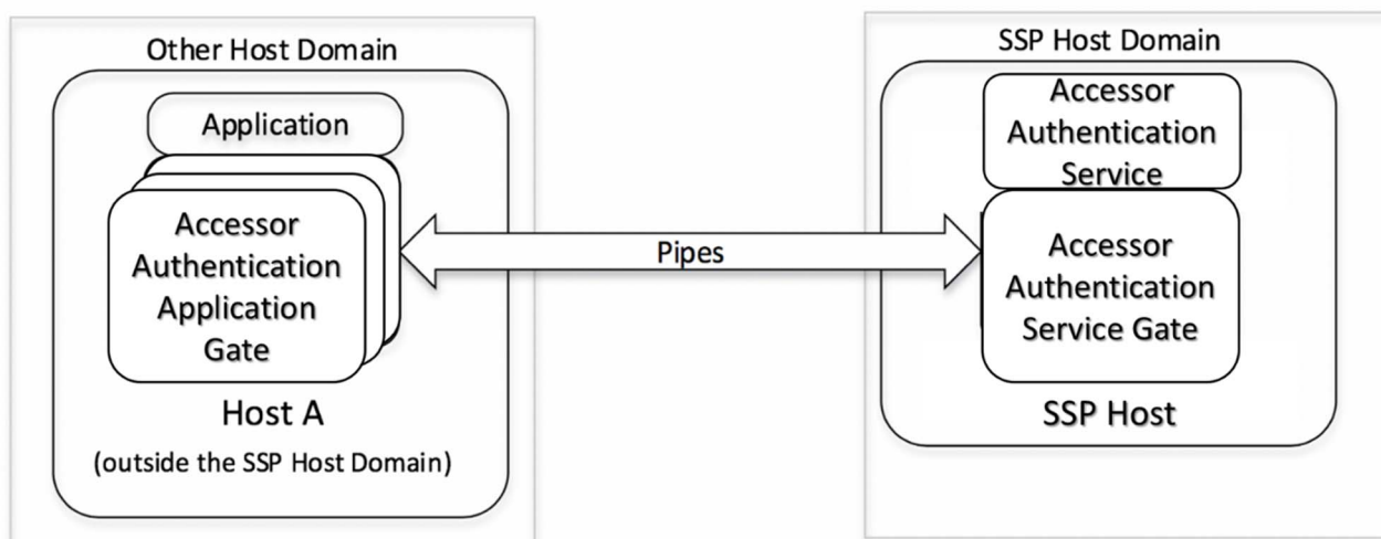
Figure 10.11: Accessor authentication service platform
