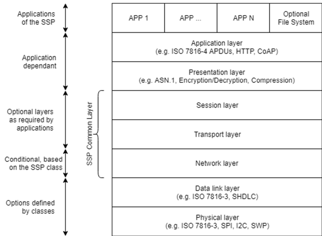
Figure 5.3: SSP protocol stack
