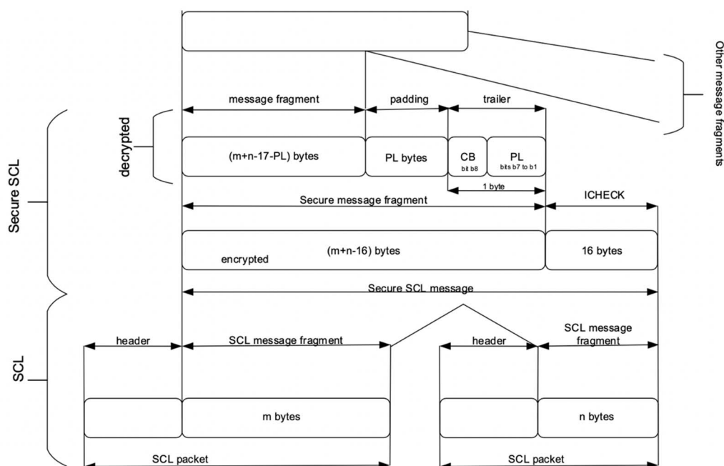
Figure 9.2: Structure of SCL message
