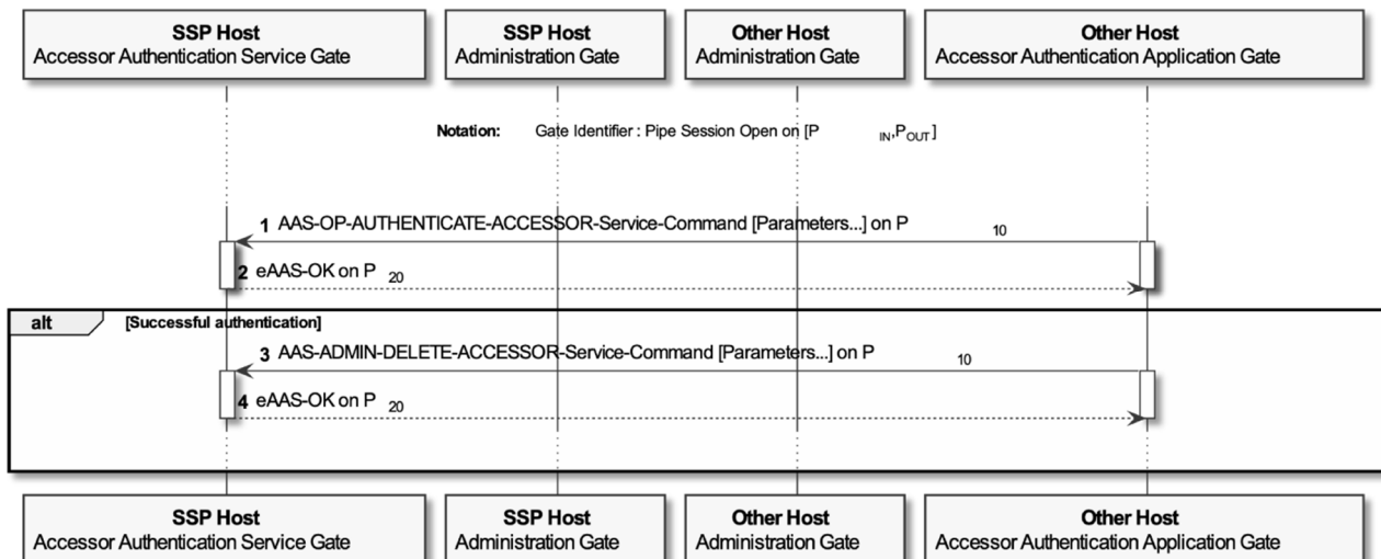
Figure J.2: Accessor deletion
