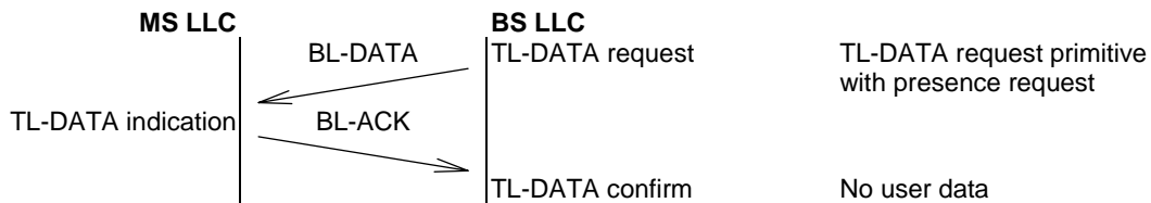
Figure 22.12: Basic link data transfer with presence indication
