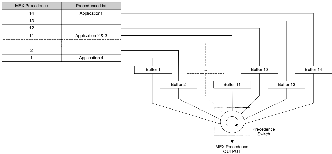
Figure 30.4: MEX Precedence
