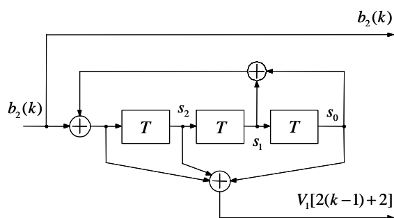
Figure 8.4: RSC encoder
