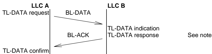
Figure 22.3: Basic link PDU exchange with acknowledgement carrying a layer 3 message
