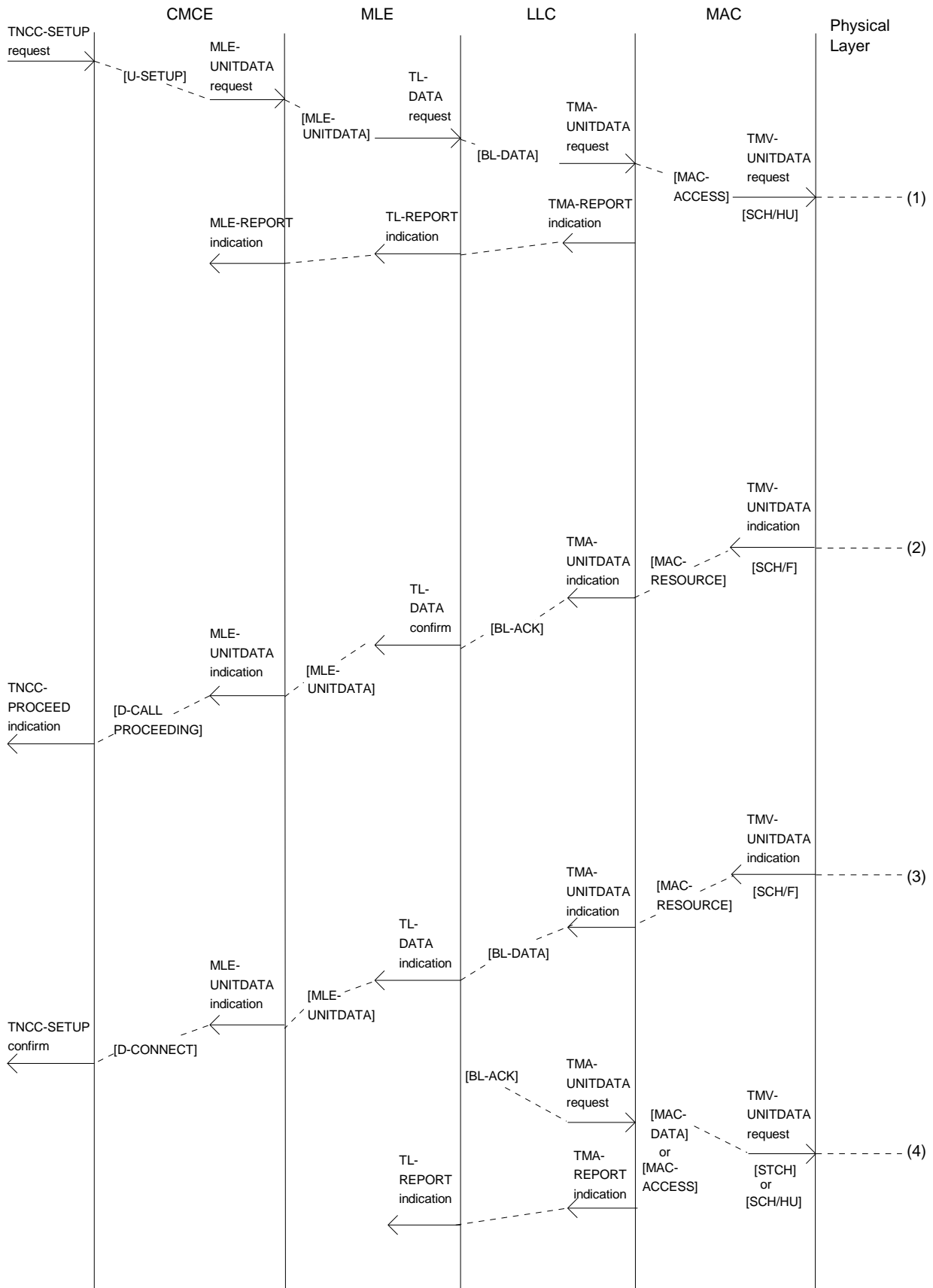
Figure 19.15: Primitives and PDUs on the calling MS air interface on a CA cell for an individual call with direct set-up signalling - Calling MS side
