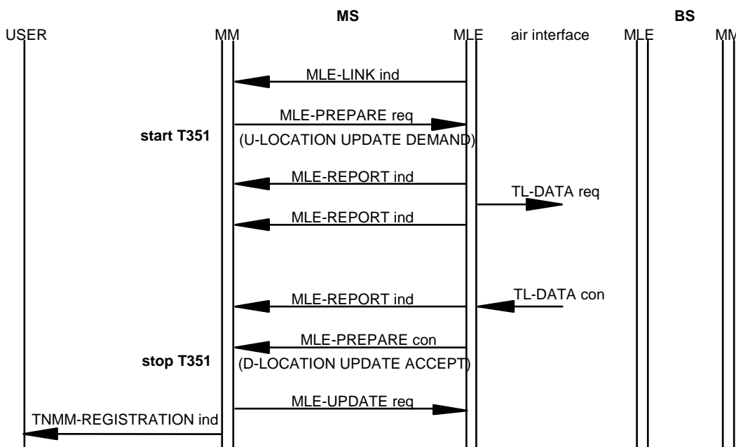
Figure 16.4: MLE initiated forward registration
