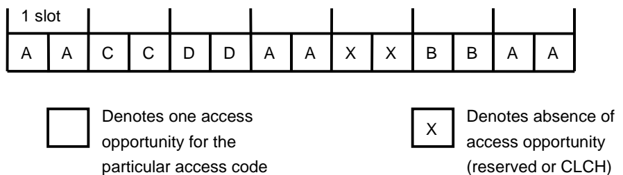
Figure 23.10: Example of subslot structure on assigned SCCH
