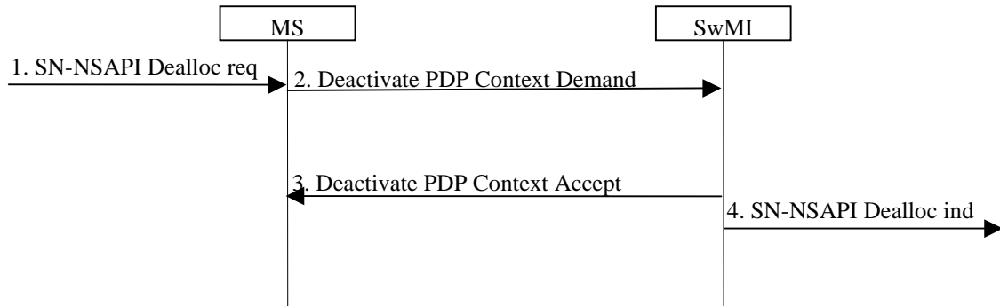
Figure 28.19: PDP context deactivation procedure
