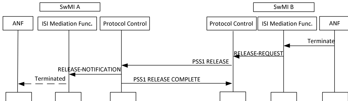
Figure 5.12: Termination of a Call Independent Connection
