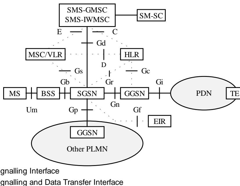
Figure 2: Configuration of a PLMN supporting GPRS
