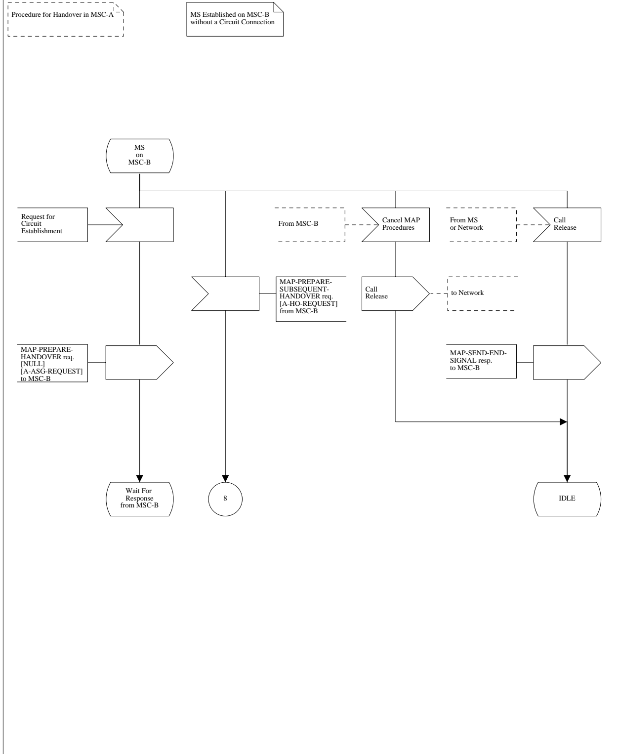
Figure 13 (Sheet 21 of 26): Handover control procedure in MSC-A
