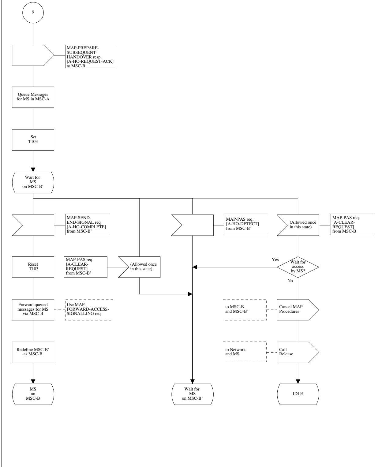
Figure 13 (Sheet 25 of 26): Handover control procedure in MSC-A
