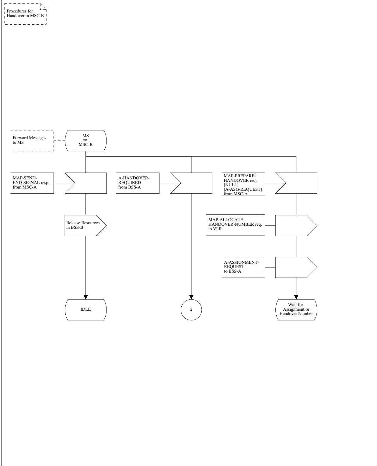
Figure 14 (Sheet 14 of 18): Handover control procedure in MSC-B
