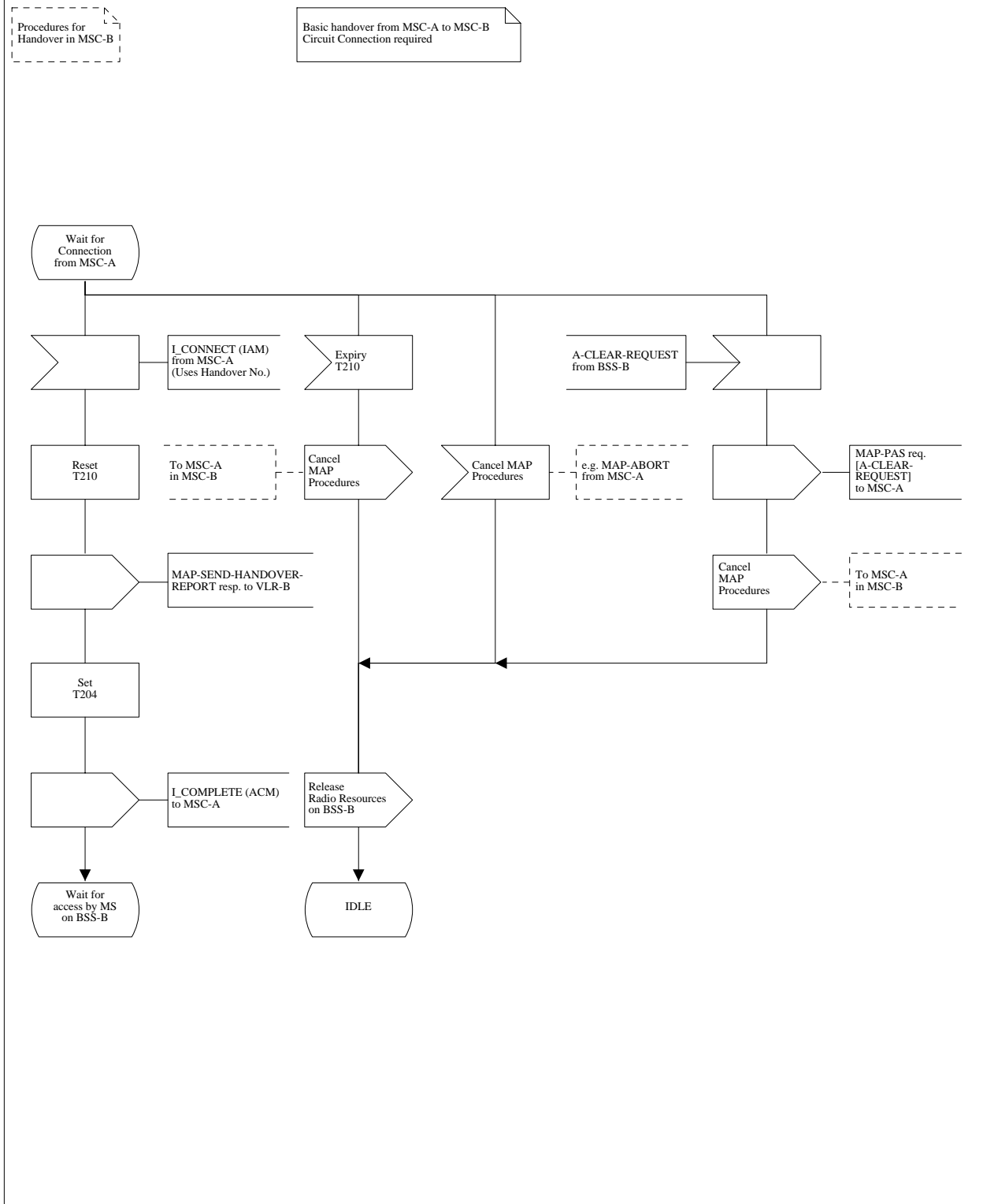
Figure 14 (Sheet 4 of 18): Handover control procedure in MSC-B
