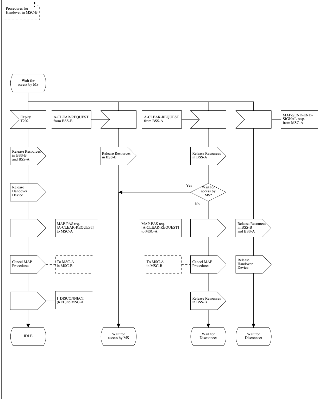
Figure 14 (Sheet 10 of 18): Handover control procedure in MSC-B
