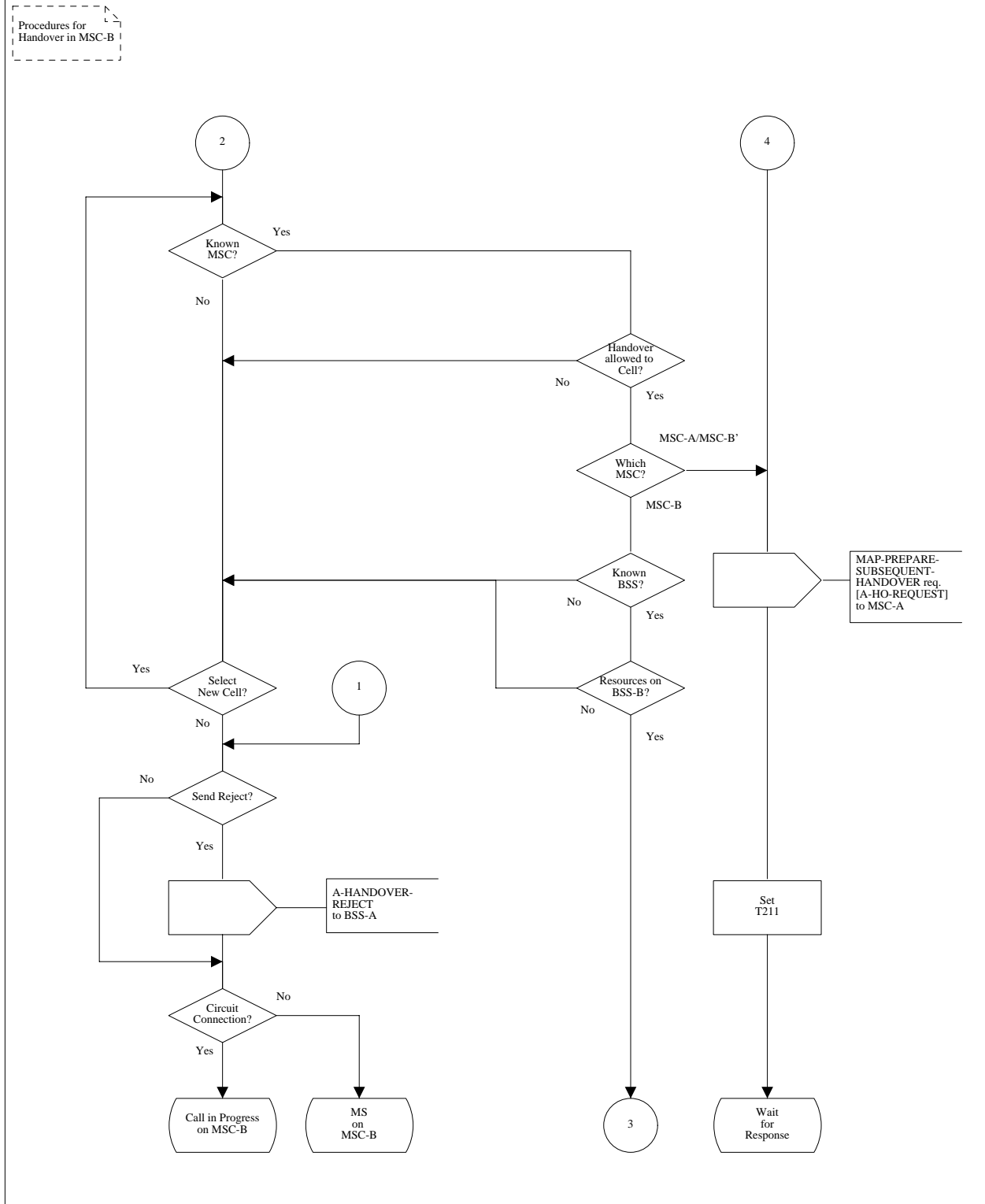
Figure 14 (Sheet 7 of 18): Handover control procedure in MSC-B
