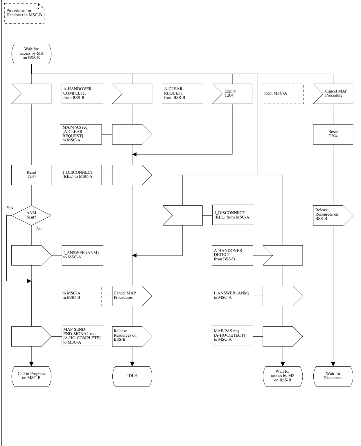
Figure 14 (Sheet 5 of 18): Handover control procedure in MSC-B
