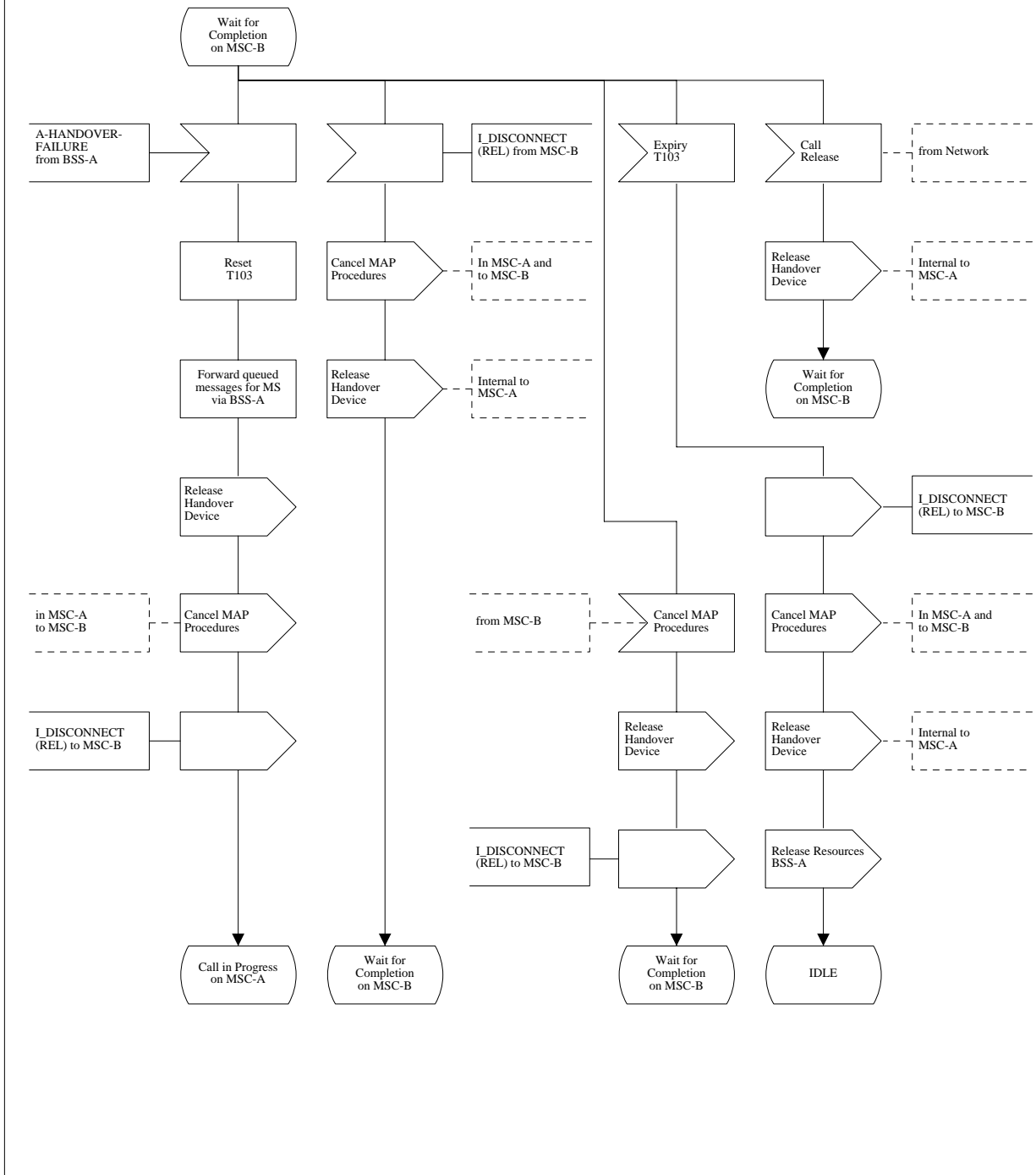
Figure 13 (Sheet 9 of 26): Handover control procedure in MSC-A
