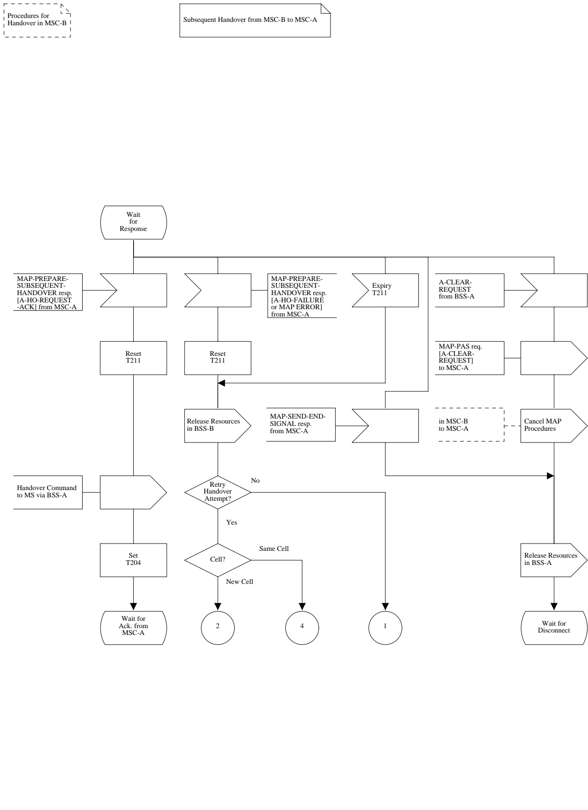
Figure 14 (Sheet 11 of 18): Handover control procedure in MSC-B
