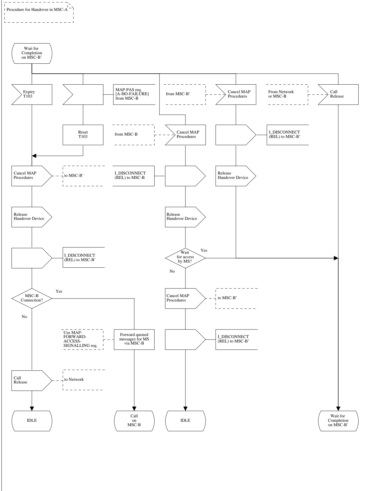
Figure 13 (Sheet 18 of 26): Handover control procedure in MSC-A
