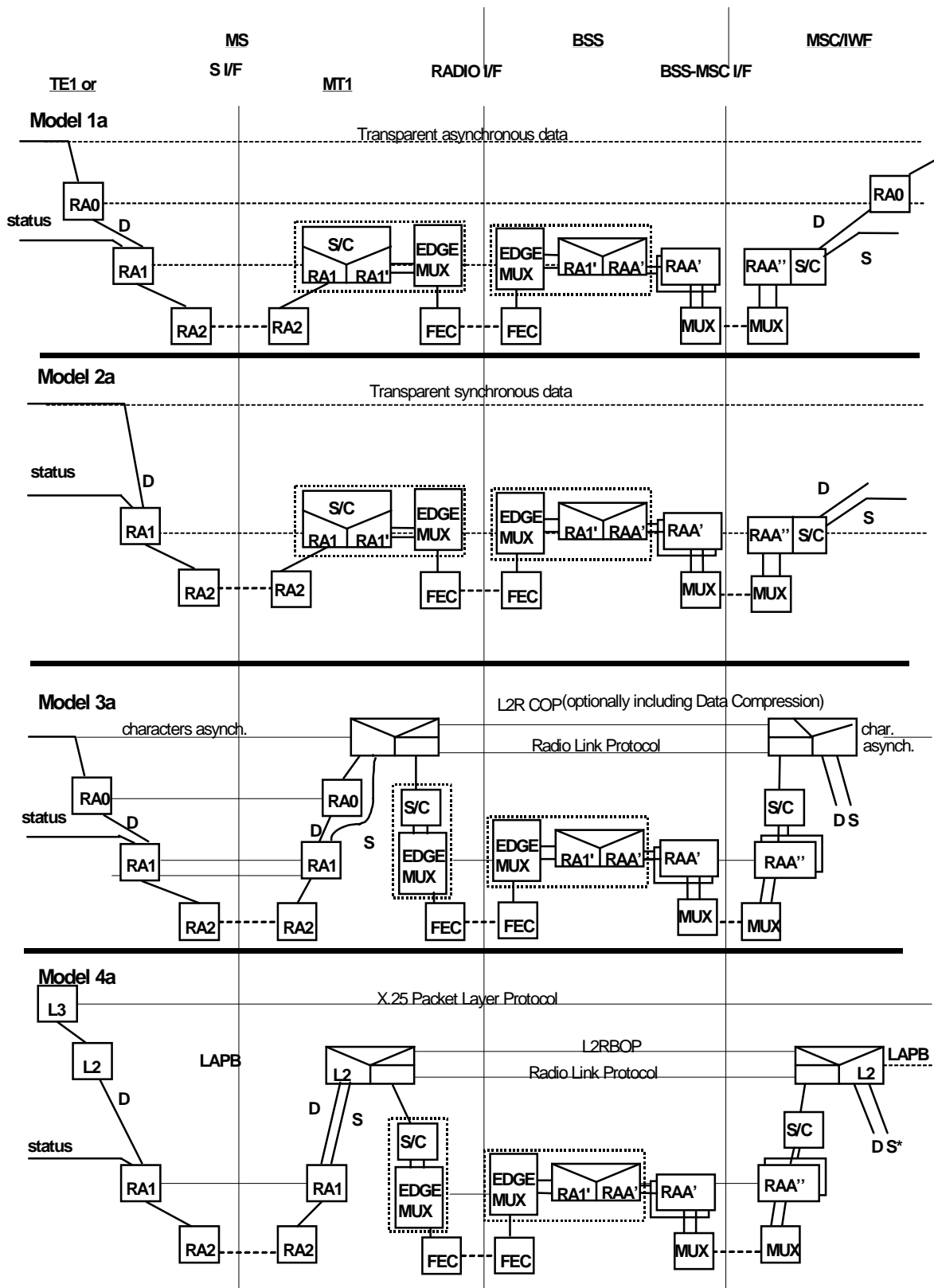
Figure 8 : Information transfer protocol models for GSM PLMN connections using EDGE channels
