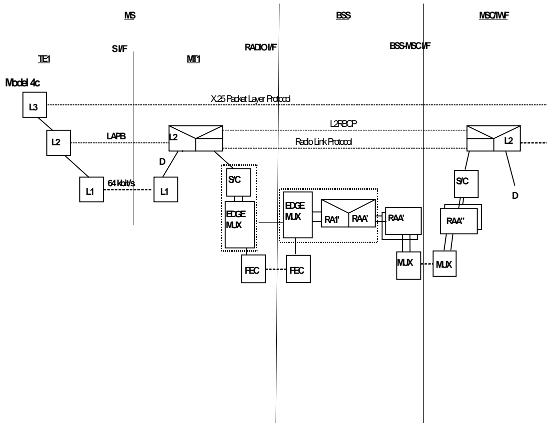
Figure 8 (concluded) : Information transfer protocol models for GSM PLMN connections using EDGE channels
