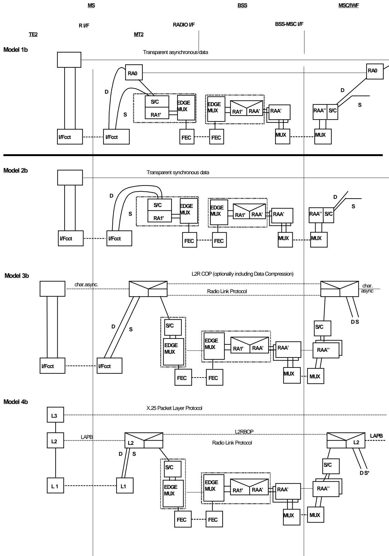
Figure 8 (continued) : Information transfer protocol models for GSM PLMN connections using EDGE channels
