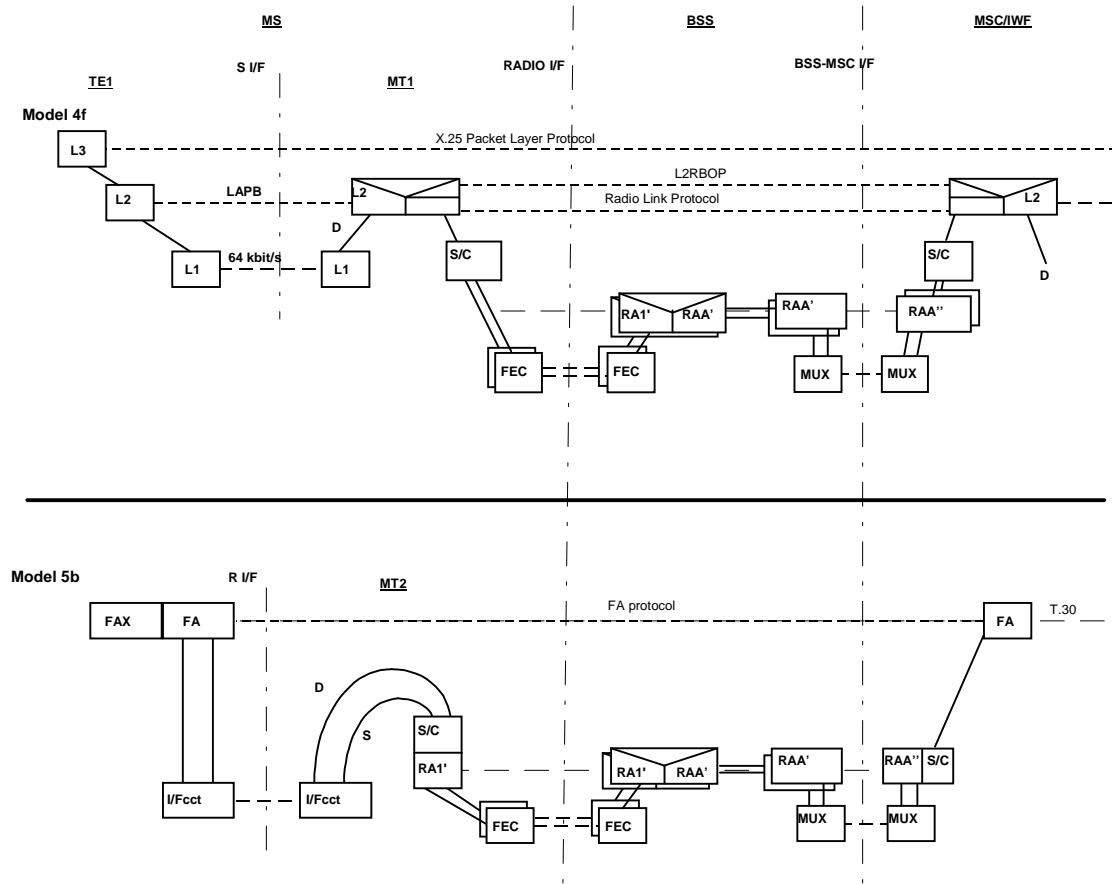
Figure 7 (continued) : Information transfer protocol models for GSM PLMN connections using 14.4 channels
