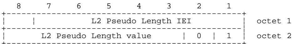
FIGURE 10.37/3GPP TS 04.08 L2 Pseudo Length information element
