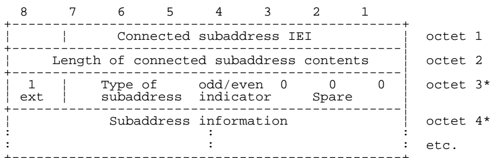
Figure 10.81/3GPP TS 04.08
