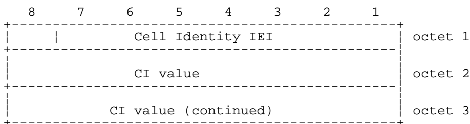
FIGURE 10.2/3GPP TS 04.08 Cell Identity information element
