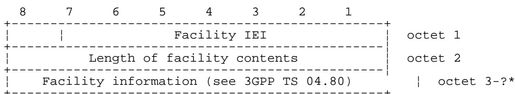
Figure 10.82/3GPP TS 04.08
