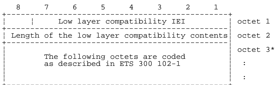
FIGURE 10.85/3GPP TS 04.08 Low layer compatibility information element
