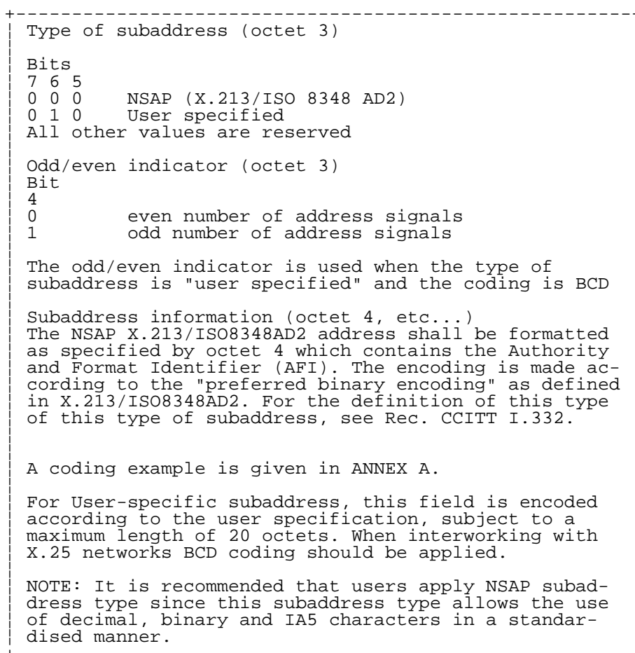
FIGURE 10.76/3GPP TS 04.08 Calling party subaddress
