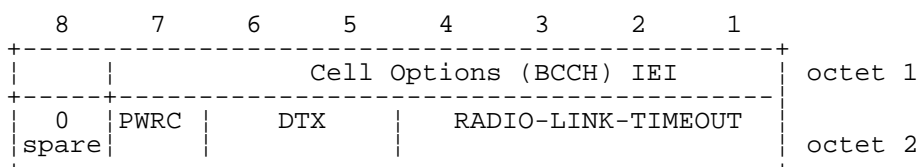
FIGURE 10.17/3GPP TS 04.08 Cell Options (BCCH) information element
