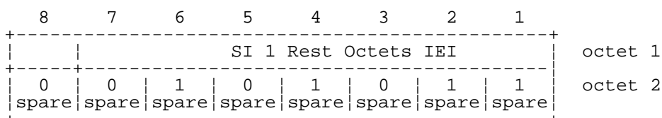
FIGURE 10.50/3GPP TS 04.08 SI 1 Rest Octets information element
