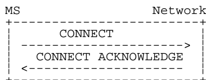
Figure 5.7/3GPP TS 04.08
