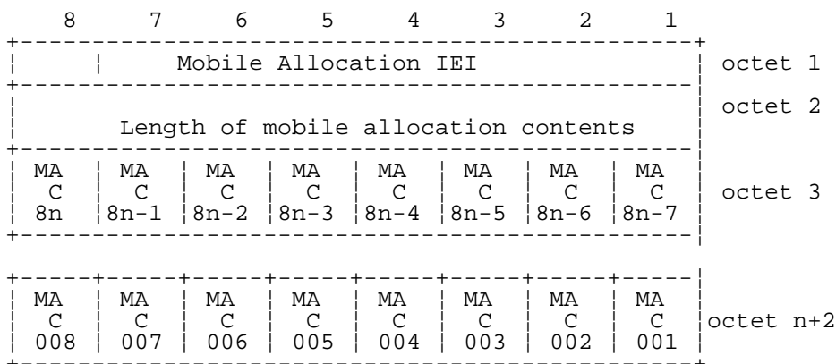
FIGURE 10.39/3GPP TS 04.08 Mobile Allocation information element.
