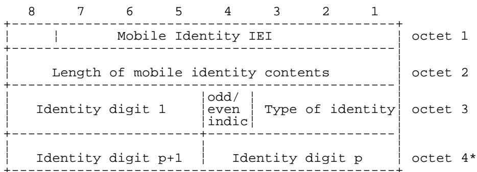
FIGURE 10.5/3GPP TS 04.08 Mobile Identity information element
