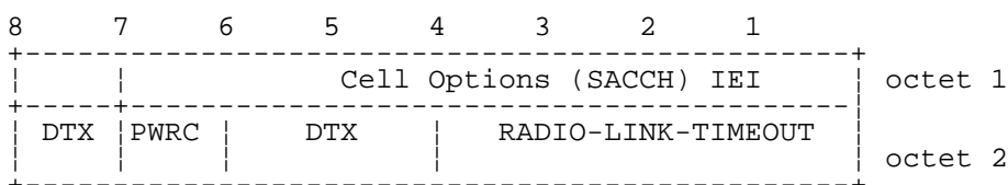
FIGURE 10.17a/3GPP TS 04.08 Cell Options (SACCH) information element
