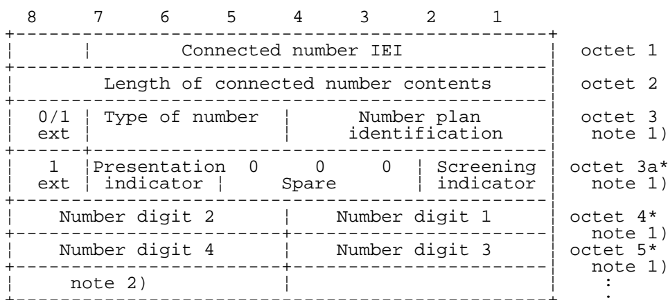
Figure 10.80/3GPP TS 04.08
