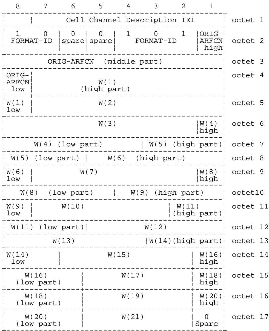
FIGURE 10.13/3GPP TS 04.08 Cell Channel Description information element, range 256 format
