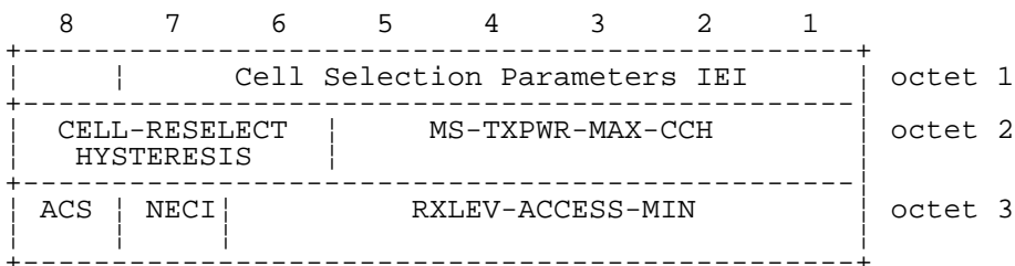
FIGURE 10.18/3GPP TS 04.08 Cell Selection Parameters information element
