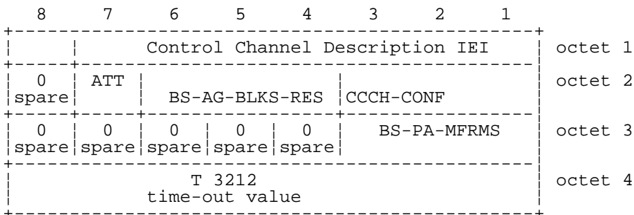
FIGURE 10.25/3GPP TS 04.08 Control Channel Description information element
