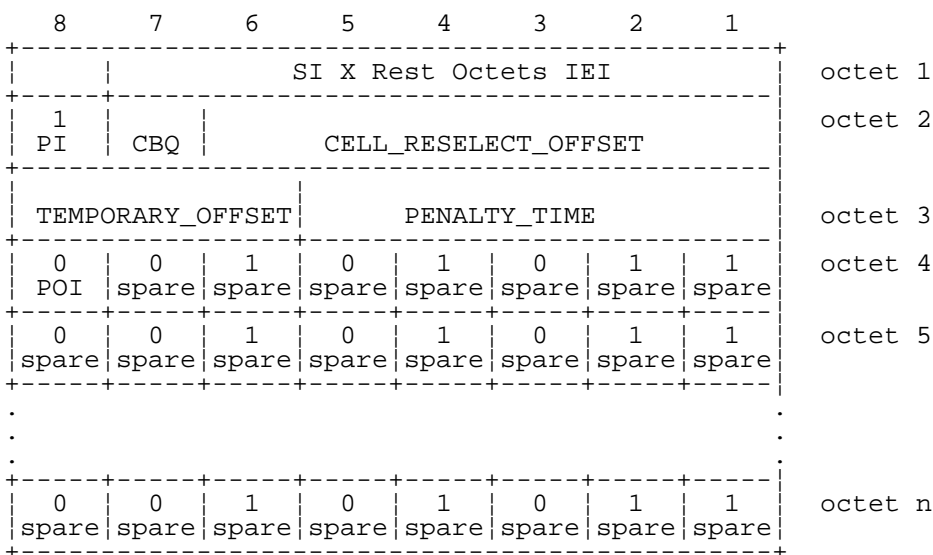
FIGURE 10.54a/3GPP TS 04.08 SI X Rest Octets information element (X = 4, 7, or 8), for PI=1 & POI=0
