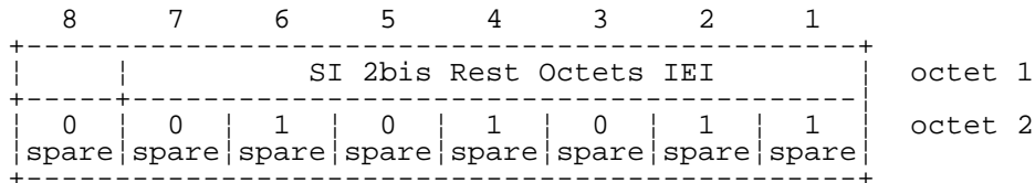
FIGURE 10.51/3GPP TS 04.08 SI 2bis Rest Octets information element
