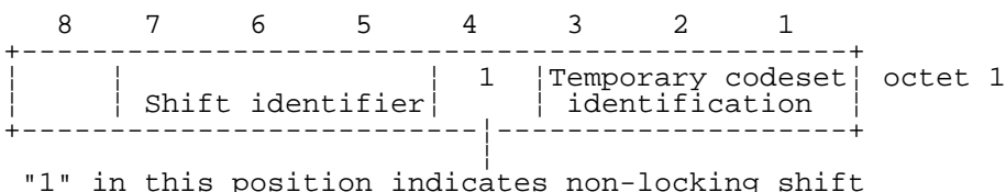
FIGURE 10.69/3GPP TS 04.08 Non-locking shift element
