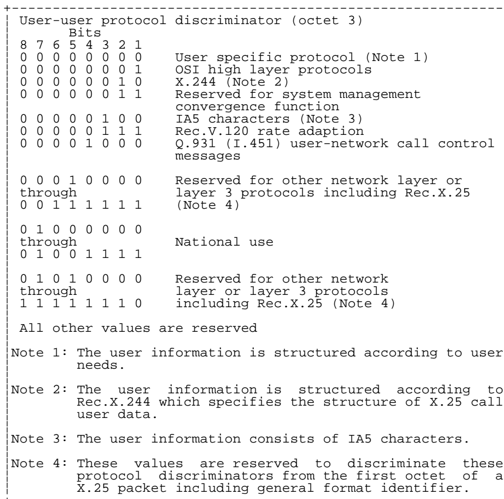
FIGURE 10.92/3GPP TS 04.08 User-user information element
