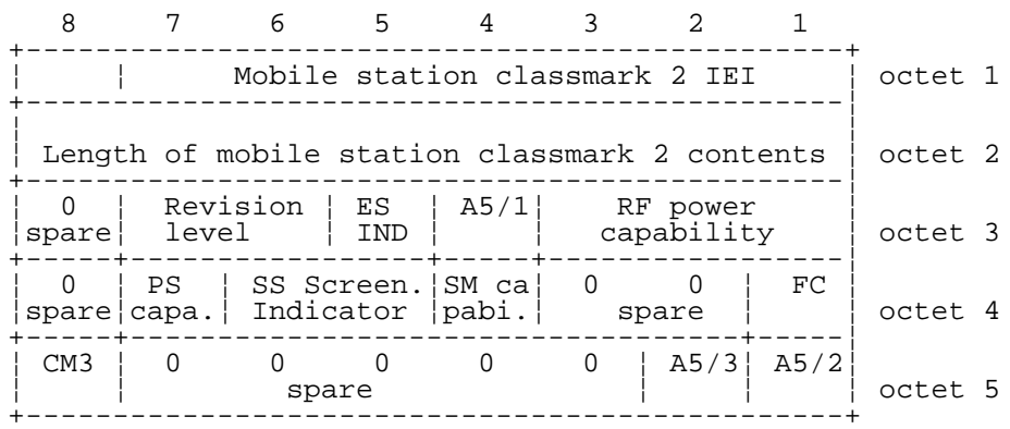
FIGURE 10.7/3GPP TS 04.08 Mobile Station Classmark 2 information element
