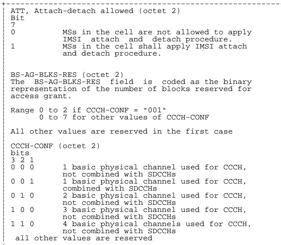
FIGURE 10.25/3GPP TS 04.08 Control Channel Description information element
