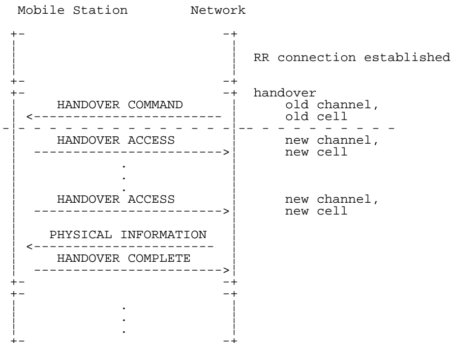
Figure 7.15/3GPP TS 04.08 Handover to a non-synchronized cell, successful case
