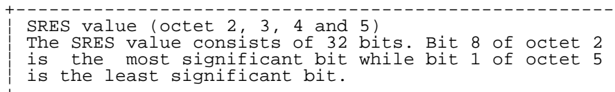
FIGURE 10.62/3GPP TS 04.08 Authentication Parameter SRES information element
