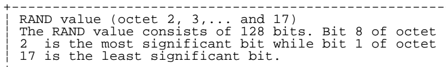
FIGURE 10.61/3GPP TS 04.08 Authentication Parameter RAND information element
