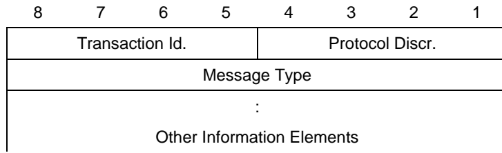
Figure 8.1/GSM 04.11
