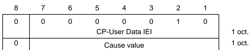
Figure 8.3/GSM 04.11: CP-Cause element layout
