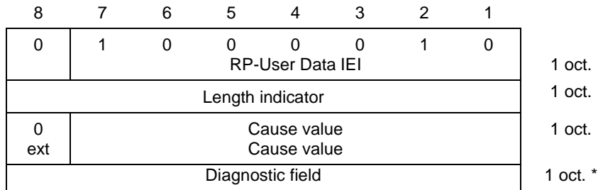
Figure 8.8/GSM 04.11: RP-Cause element layout
