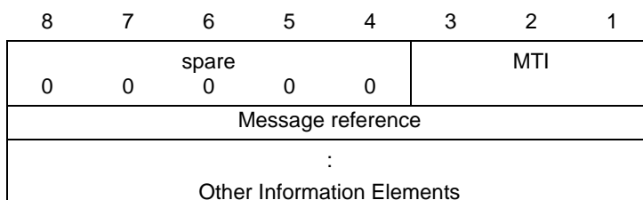
Figure 8.4/GSM 04.11
