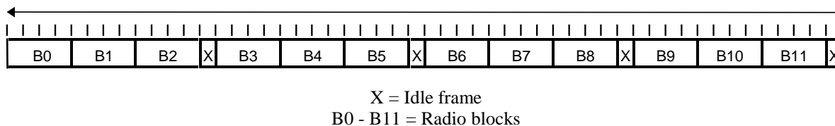
Figure 2a: 52- multiframe for PDCHs
