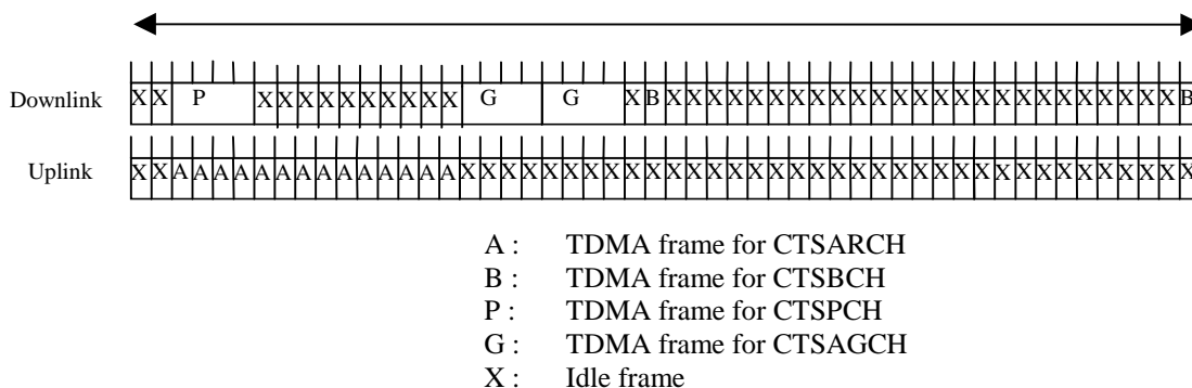
Figure 2b: 52-multiframe for CTS
