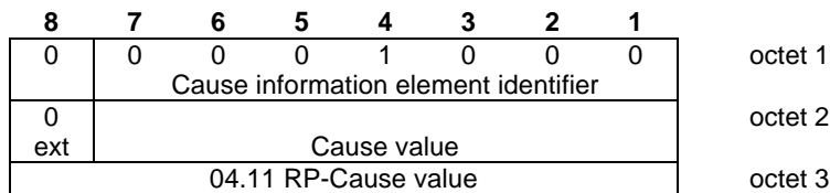
Figure 2.5.10/GSM 07.05: Cause information element
