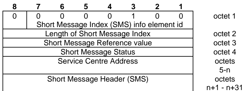
Figure 2.5.6/GSM 07.05: Short Message Index (SMS) information element
