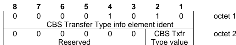
Figure 2.5.12/GSM 07.05: CBS Transfer Type information element
