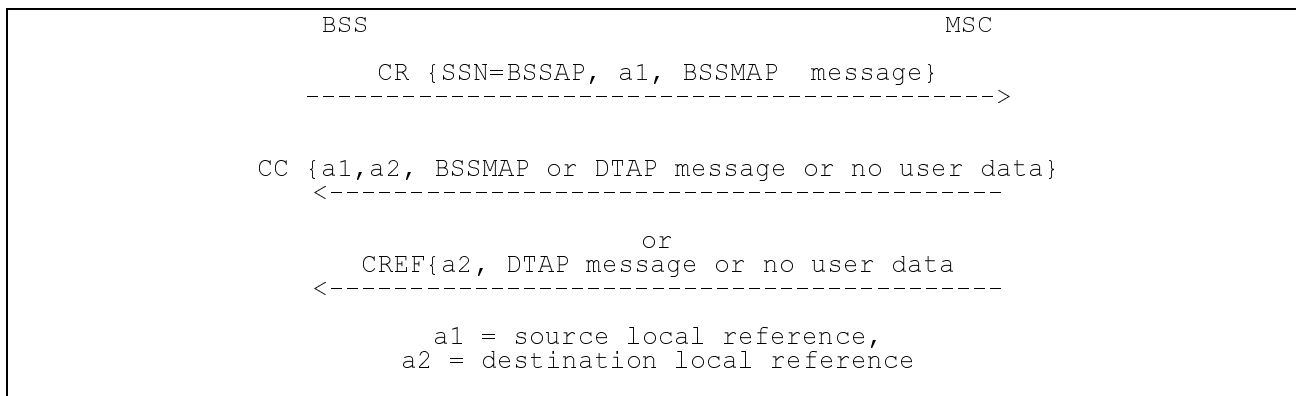
Figure 1/08.06 Set-up of SCCP connections on the first BSS/MS interface
