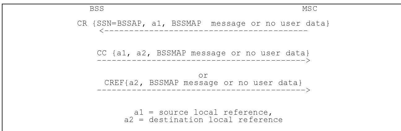
Figure 2/08.06 Set-up of SCCP connections on a new BSS/MS (handover) interface or for a voice group or broadcast call initiation
