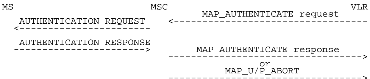
Figure 2: Authentication operation
