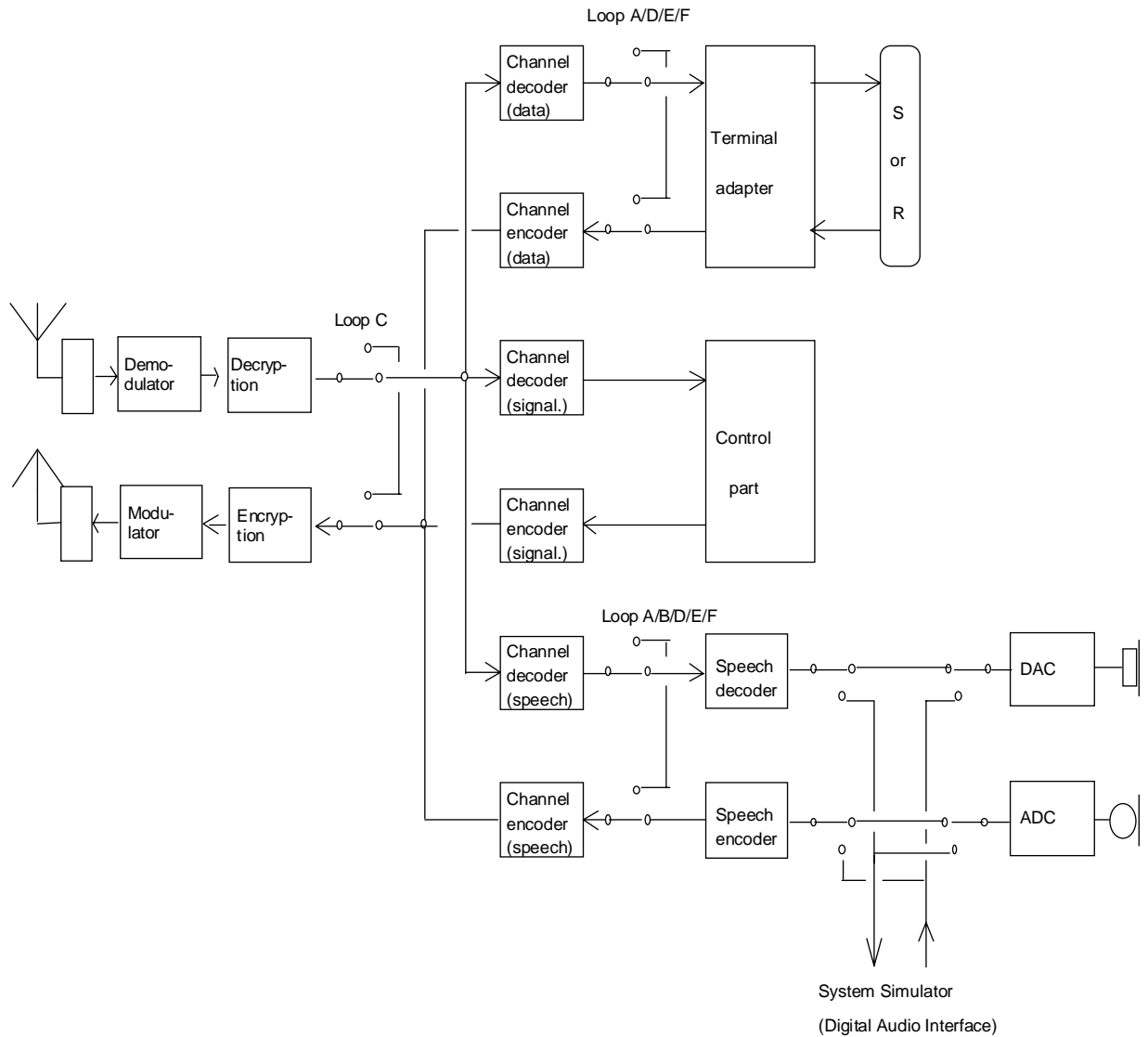
Figure 36-1: Test loops in the MS
