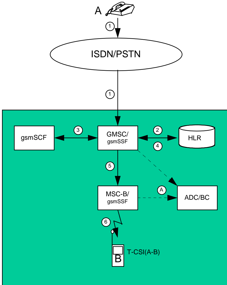
Figure B.11: Incoming call handled by CAMEL without redirection
