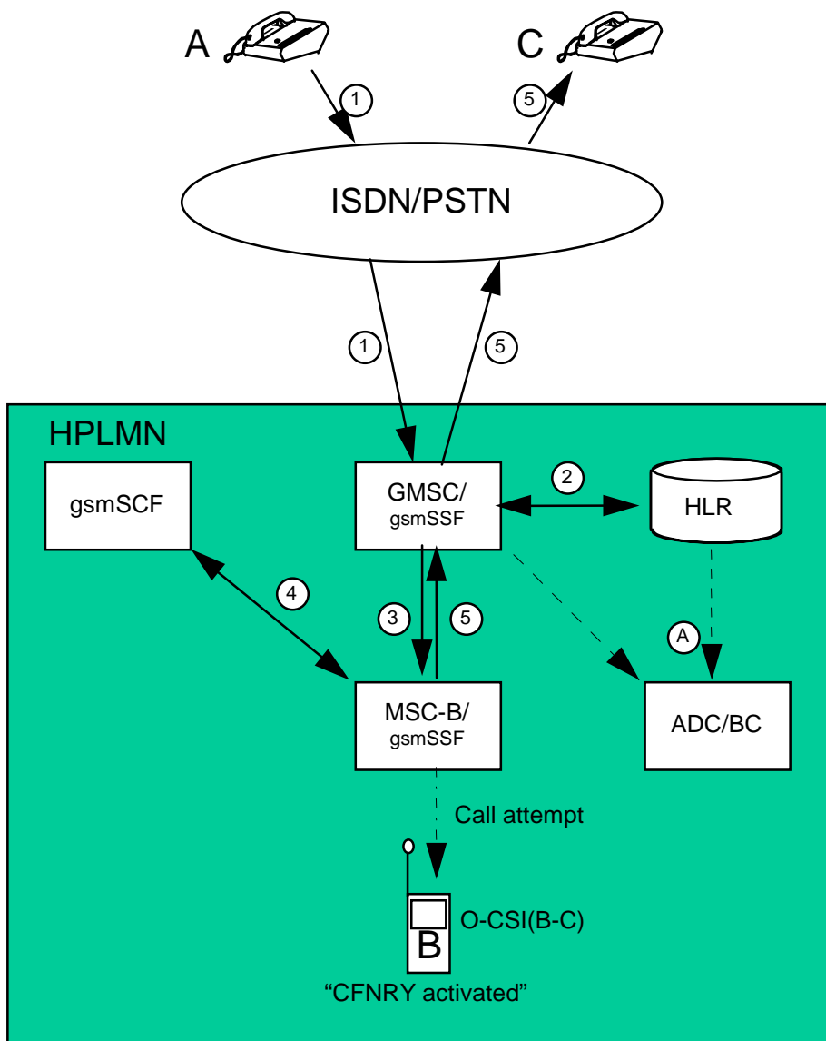
Figure B.4.17: Late forwarded call controlled by CAMEL
