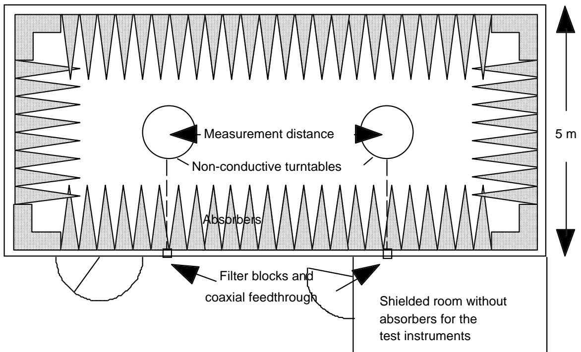
Figure A.3: Example of construction of an anechoic shielded chamber
