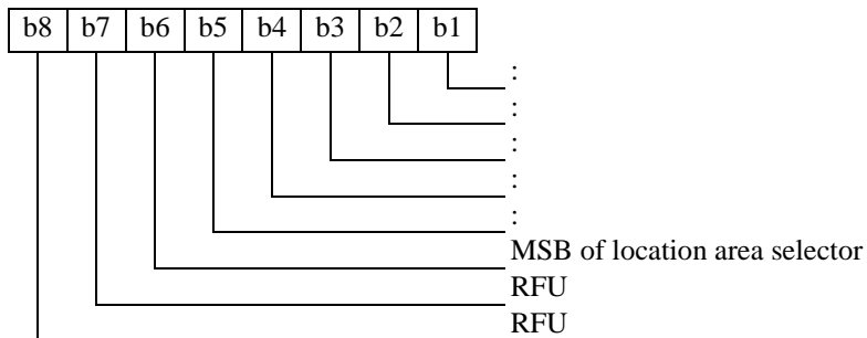
Figure 14: Location area selector
