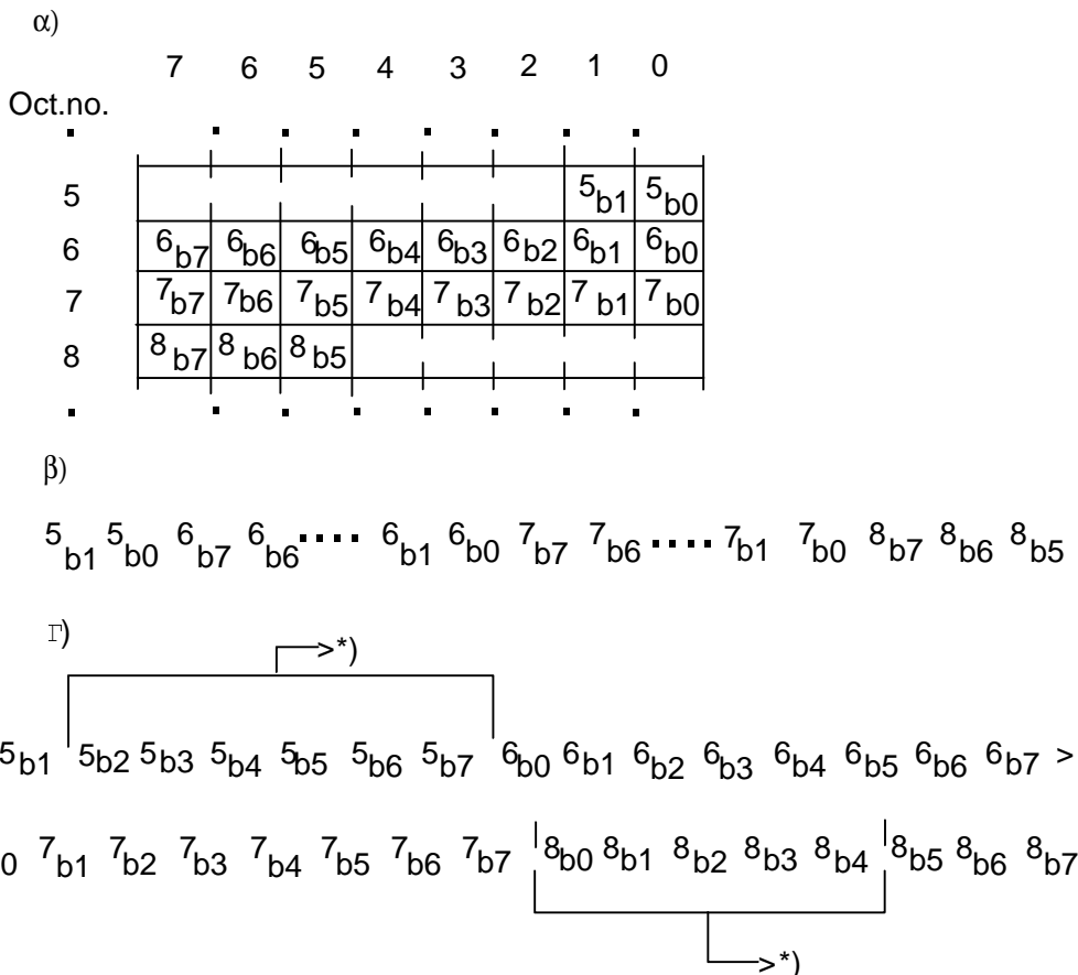
Figure 03.40/8: 21 bits from the octets 5, 6, 7, and 8 in a short message α) will represent an integer as shown in β), and will be transmitted in an order as shown in Γ)
