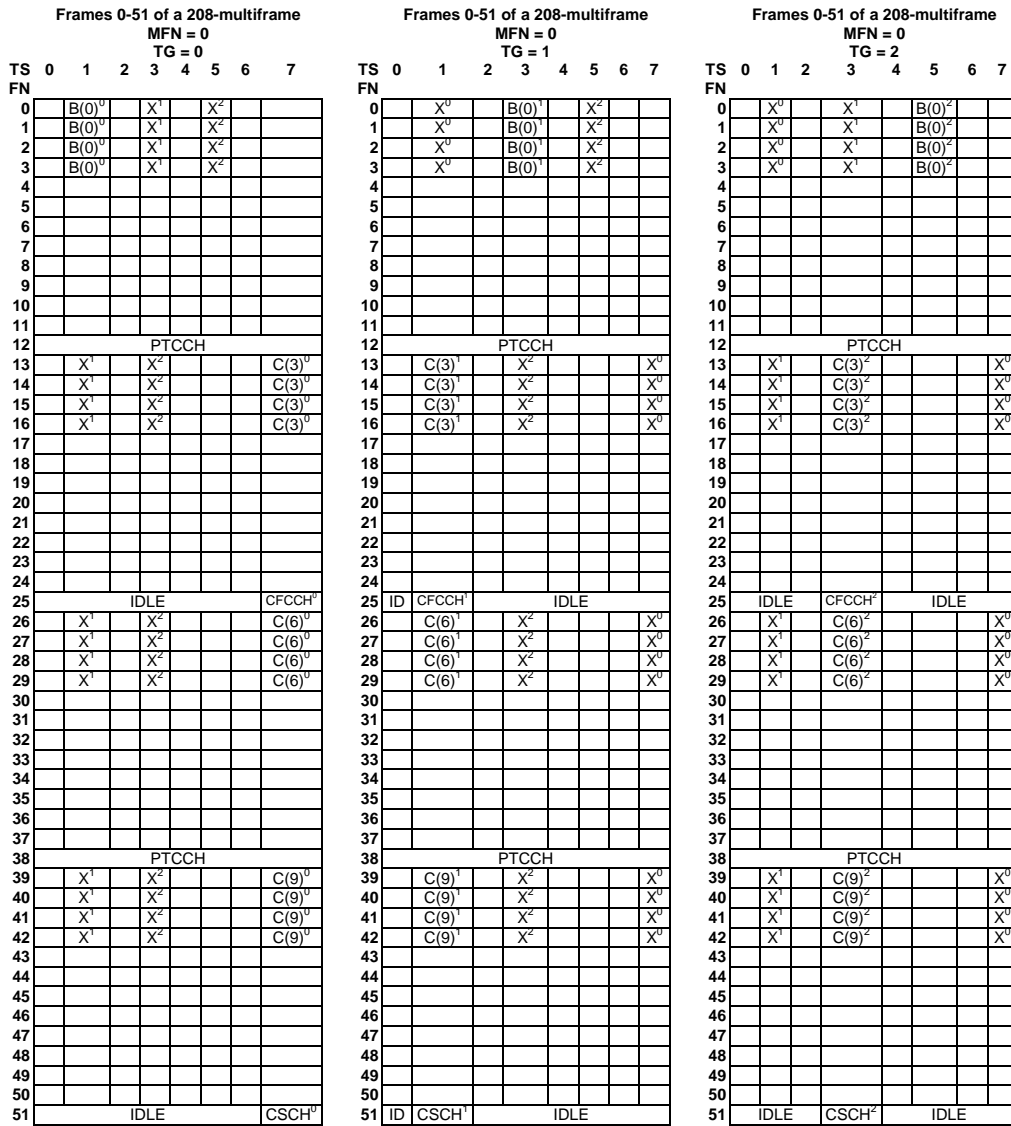
Figure D.2: COMPACT downlink 52-multiframe structure using 3 time groups for nominal cells (based on an assignment of 1 CPBCCCH and 3 CPCCCHs with NIB_CCCH_0 = NIB_CCCH_1 = NIB_CCCH_2 = 4, NIB_CCCH_3 = 0). NIB_CCCHs not broadcast for serving cell time group
