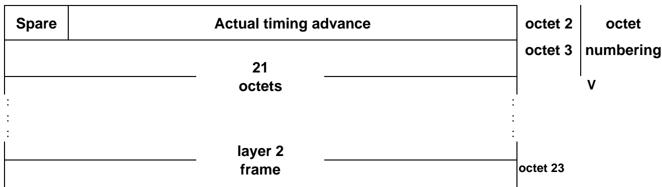
Figure 7.2: SACCH uplink block format
