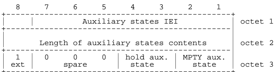
Figure 10.5.87/3GPP TS 04.08: Auxiliary states information element
