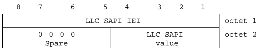
Figure 10.5.141/3GPP TS 04.08: LLC service access point identifier information element
