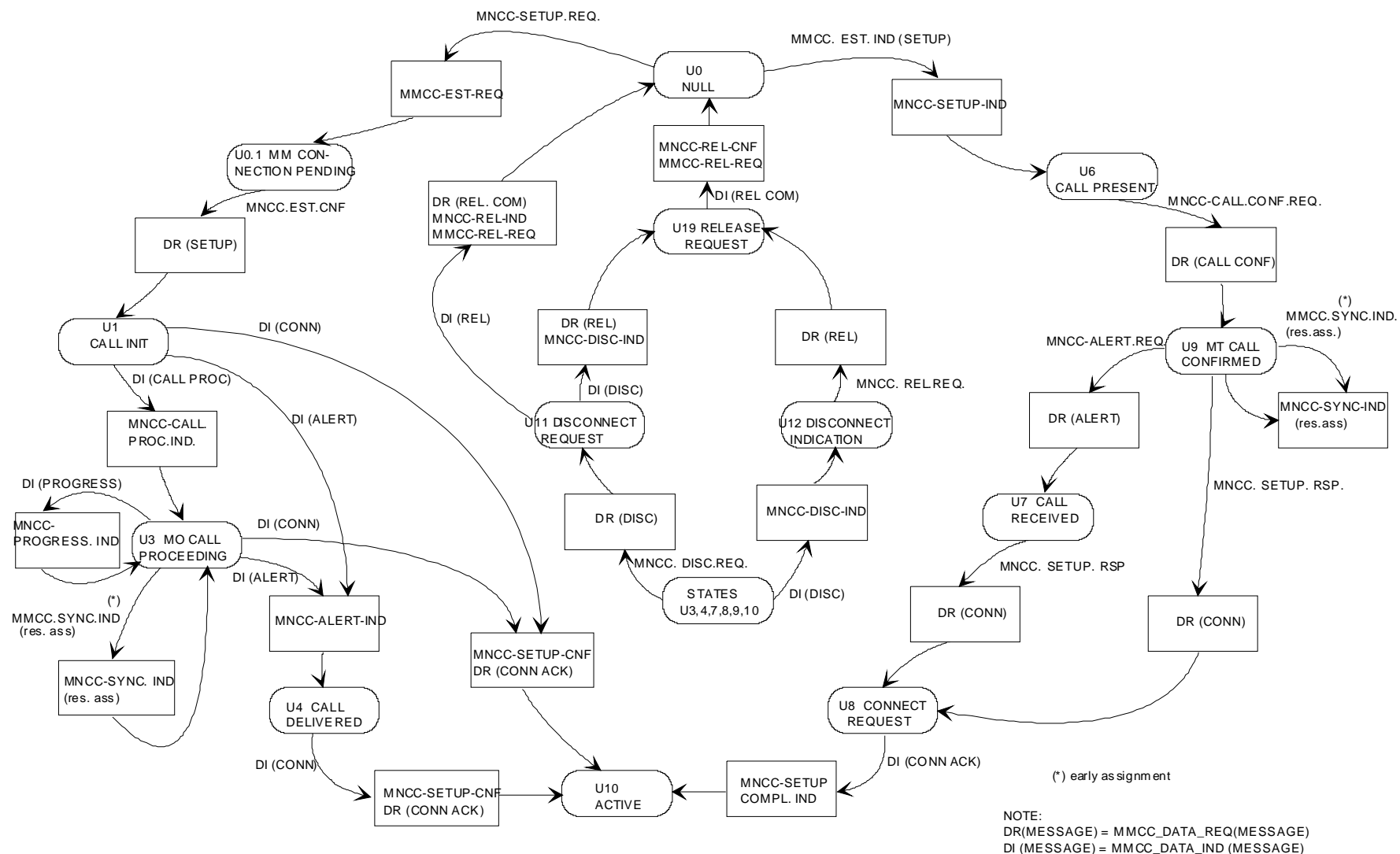
Figure 5.1a/3GPP TS 04.08: Overview call control protocol/MS side
