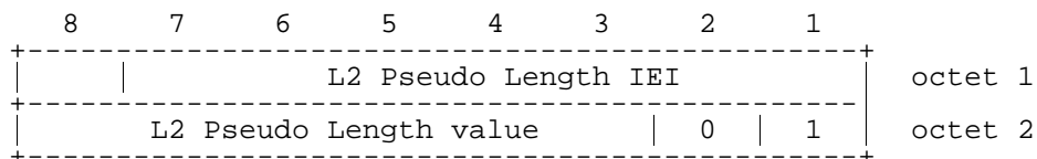
Figure 10.5.46/3GPP TS 04.08: L2 Pseudo Length information element
