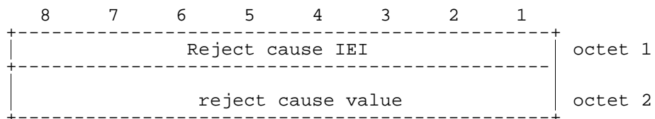
Figure 10.5.81/3GPP TS 04.08: Reject Cause information element
