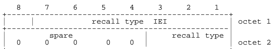
Figure 10.5.108/3GPP TS 04.08: Recall type information element
