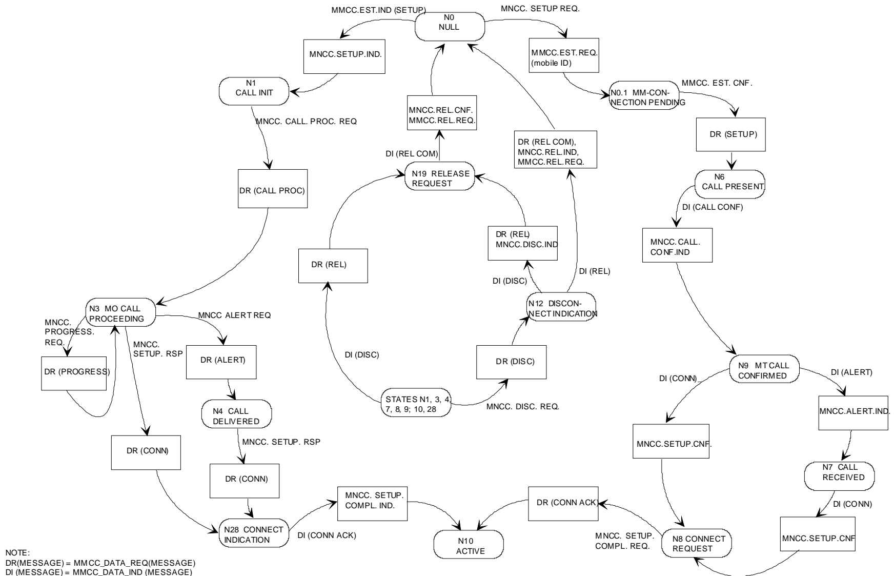
Figure 5.1b/3GPP TS 04.08: Overview call control protocol/Network side
