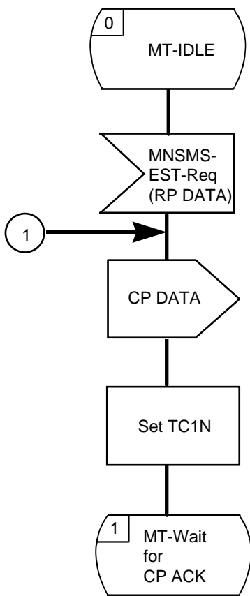
MT-SMC-GP entity on Network-side for GPRS SDL-22
