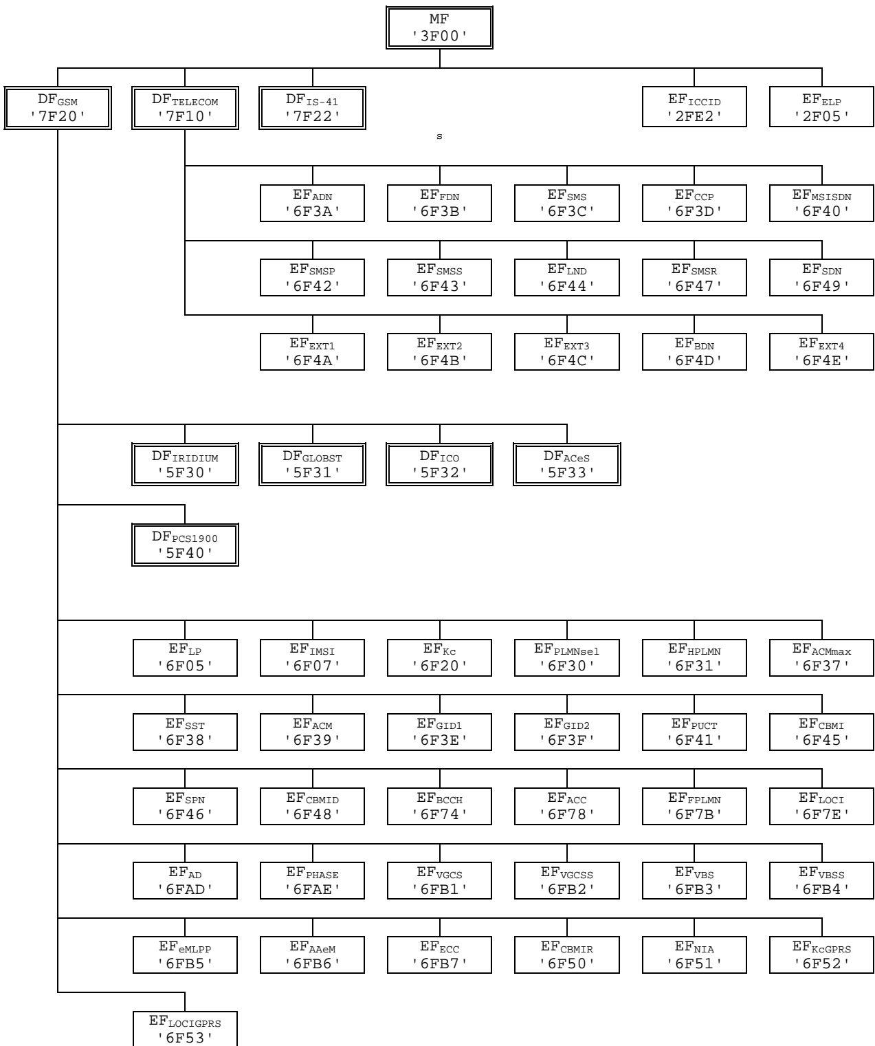
Figure 8: File identifiers and directory structures of GSM
