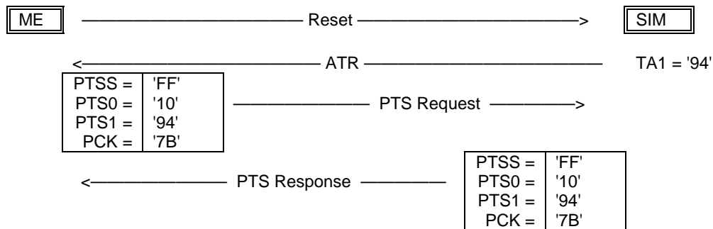
Figure 2: PTS procedure requesting enhanced speed values (F=512, D=8, see subclause 5.8.3)
