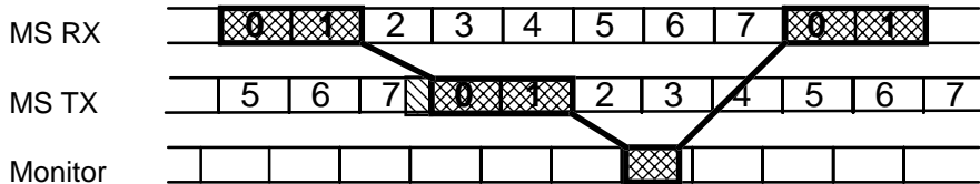
Figure 2: Double slot operation in the air interface
