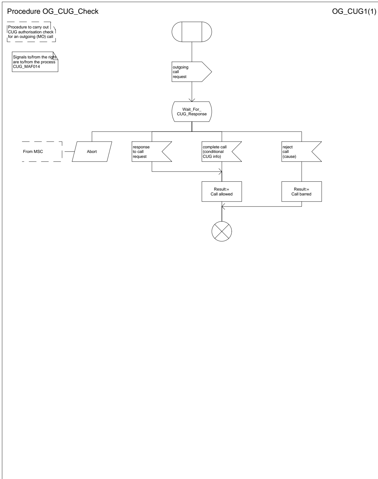
Figure 31: Procedure OG_CUG_Check
