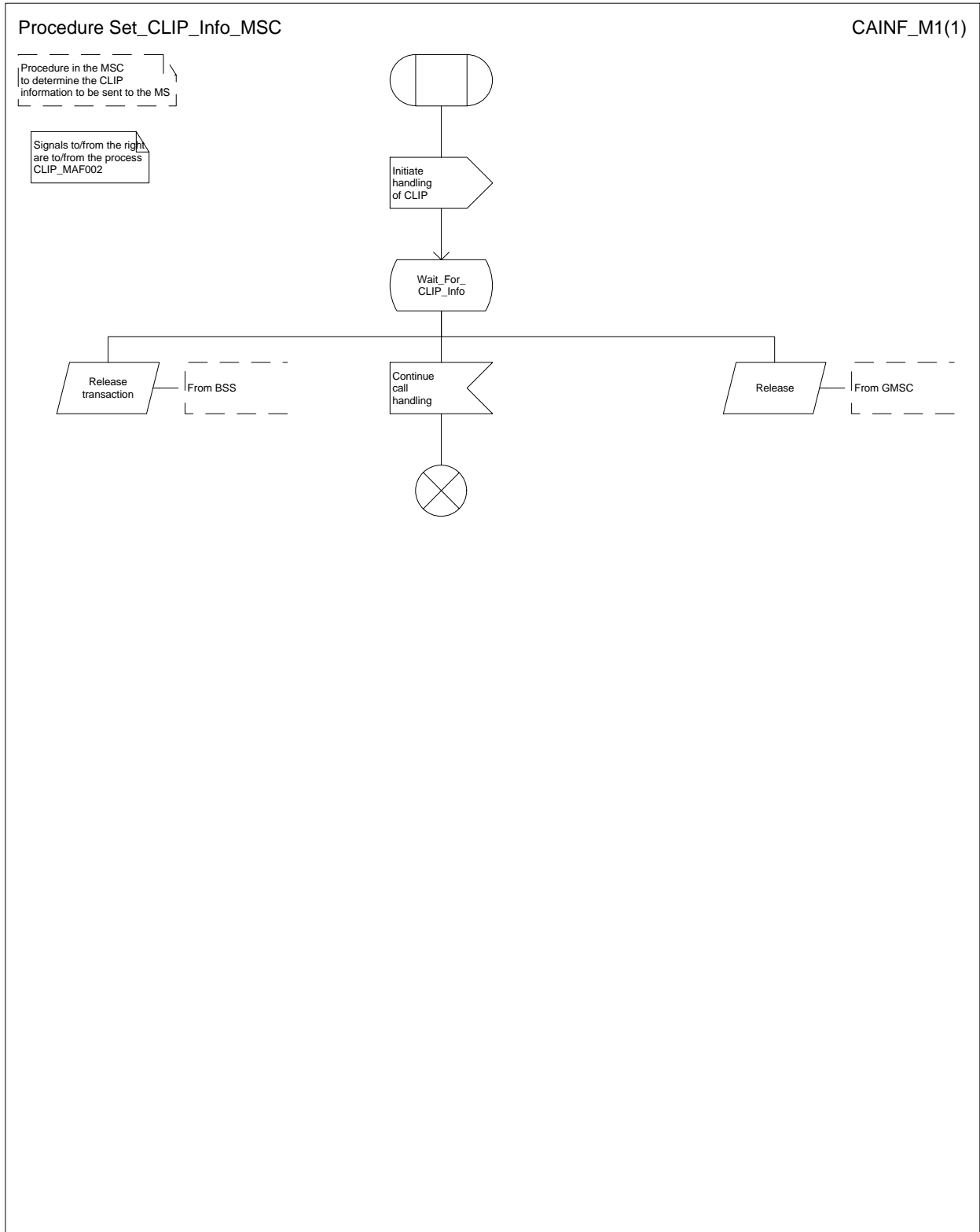
Figure 63: Procedure Set_CLIP_Info_MSC
