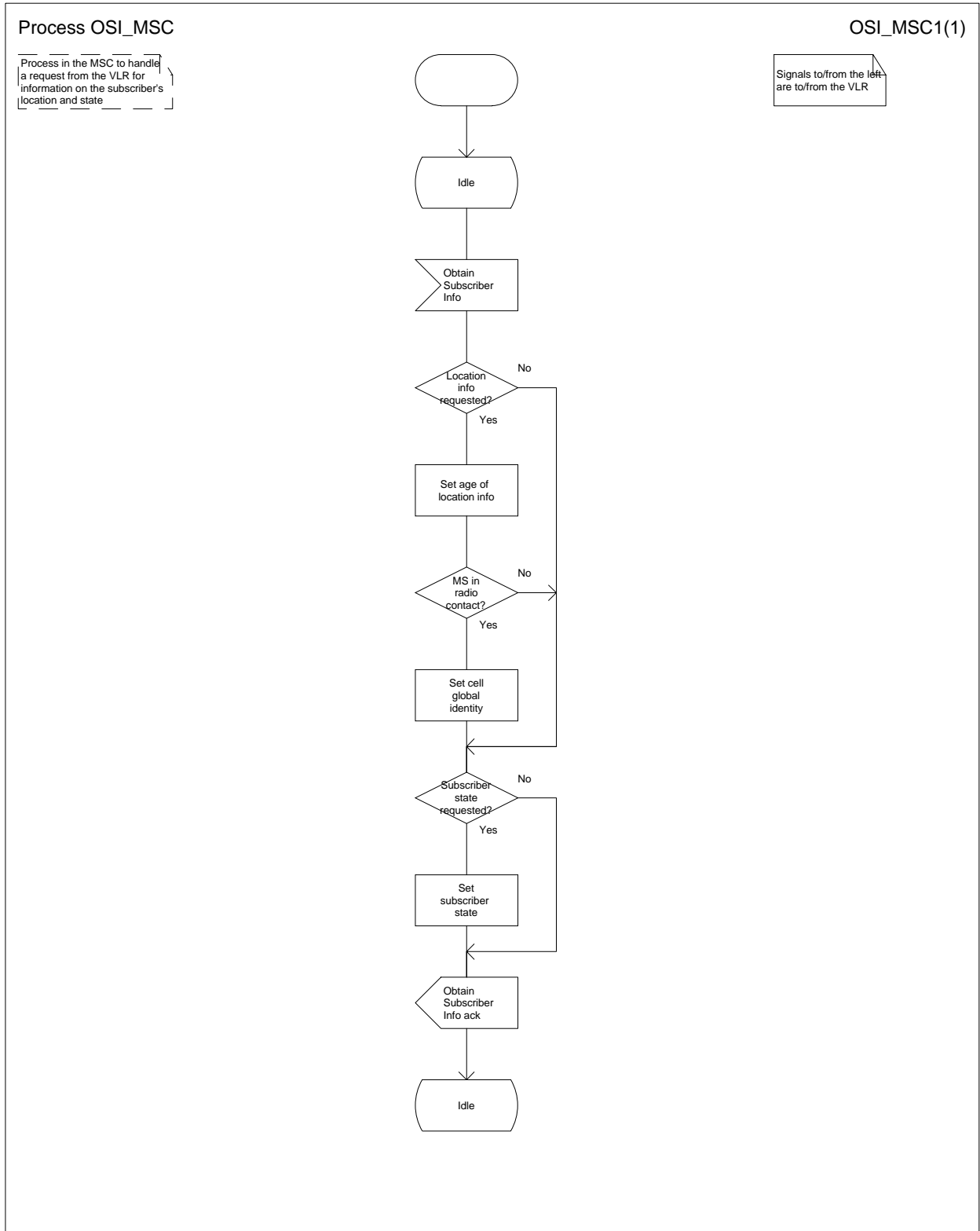
Figure 57: Process OSI_MSC
