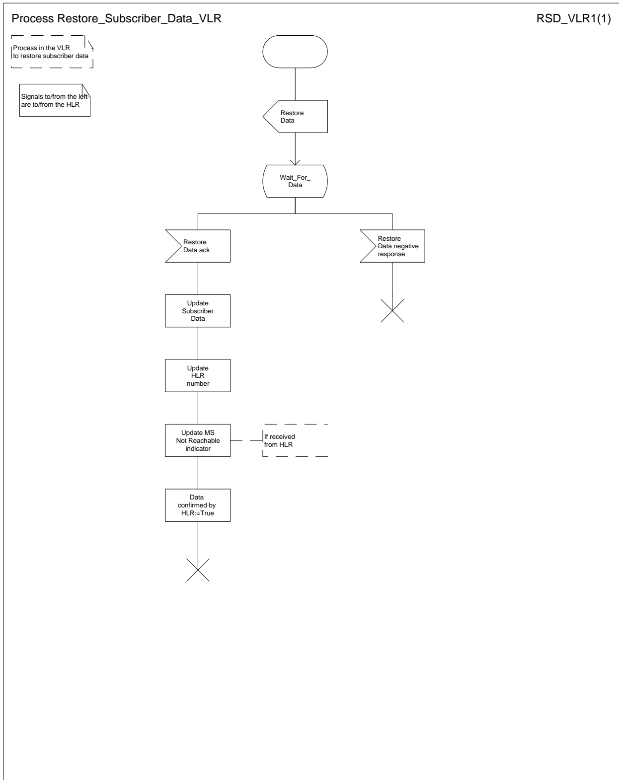
Figure 55: Process Restore_Subscriber_Data_VLR
