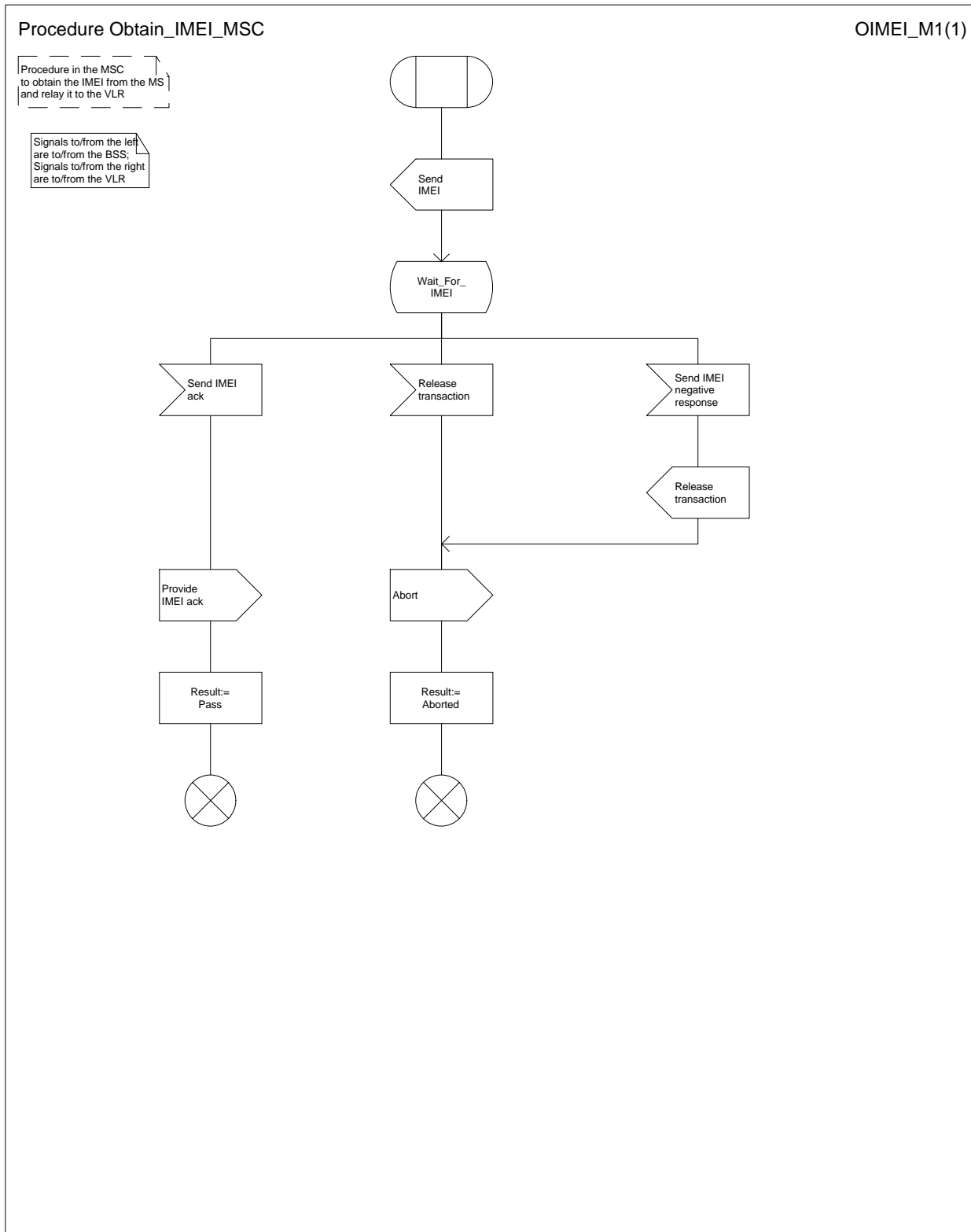
Figure 11: Procedure Obtain_IMEI_MSC
