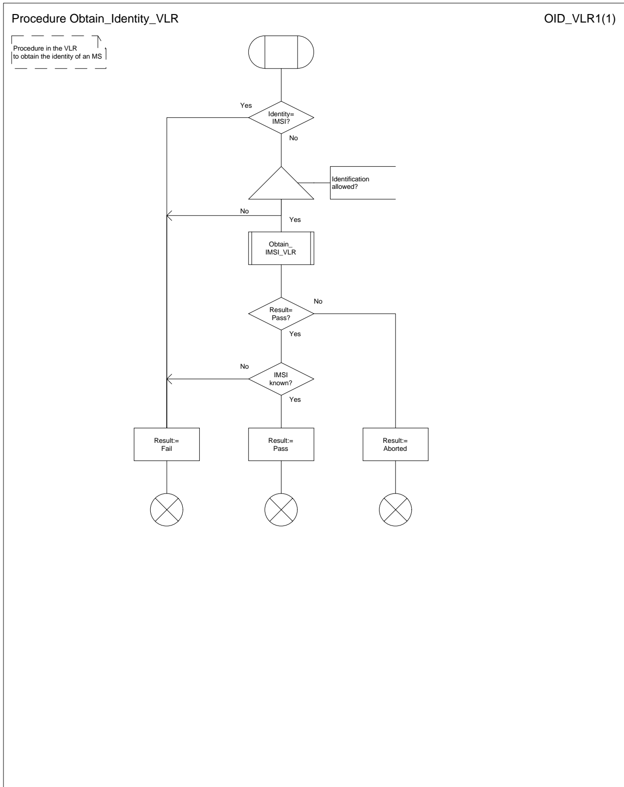
Figure 22: Procedure Obtain_Identity_VLR
