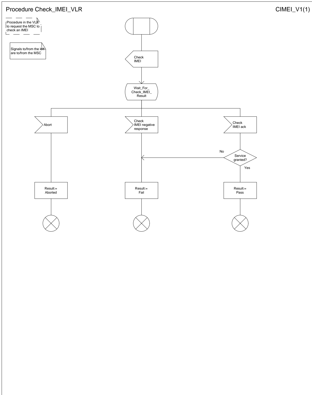
Figure 27: Procedure Check_IMEI_VLR
