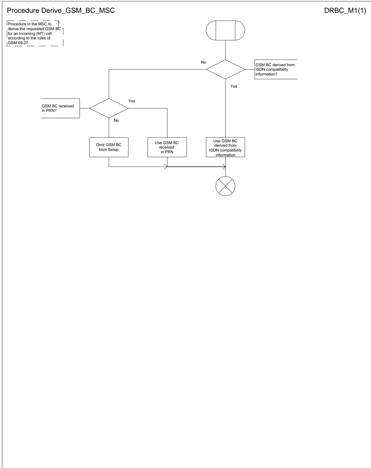
Figure 64: Derive_GSM_BC_MSC
