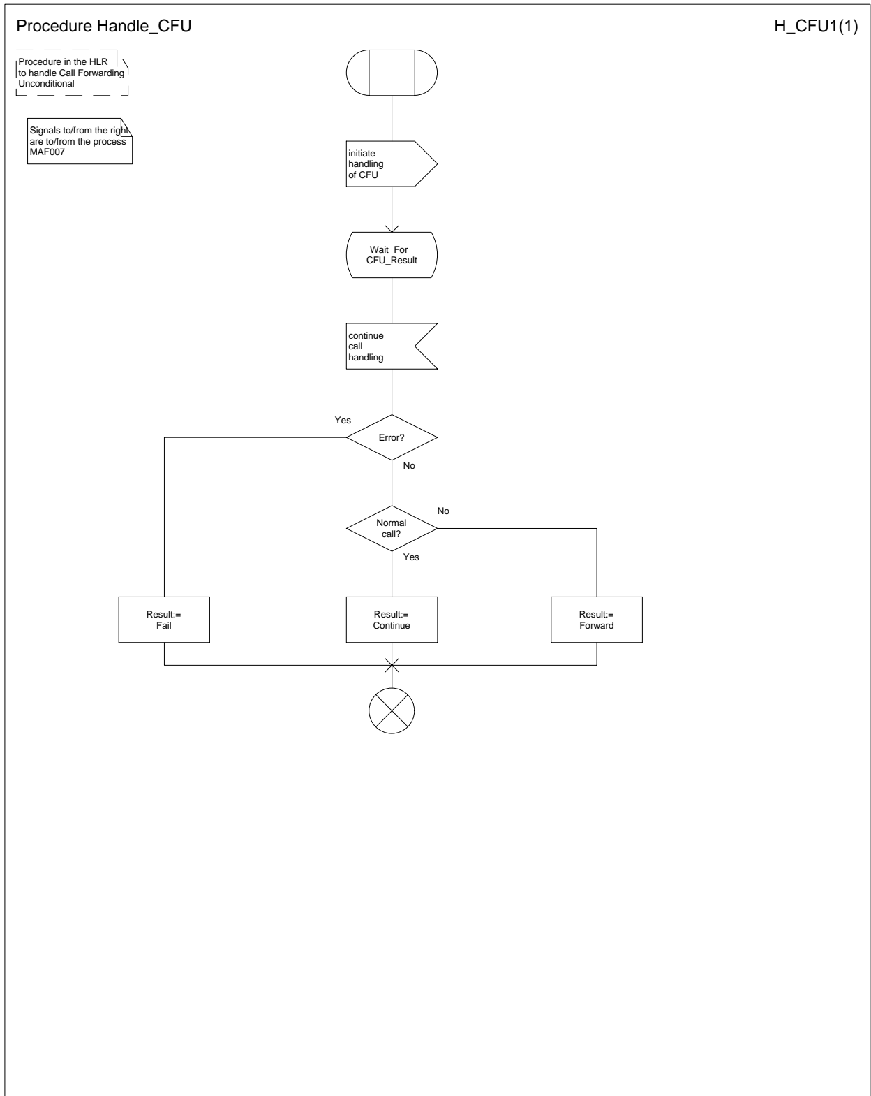
Figure 52: Procedure Handle_CFU
