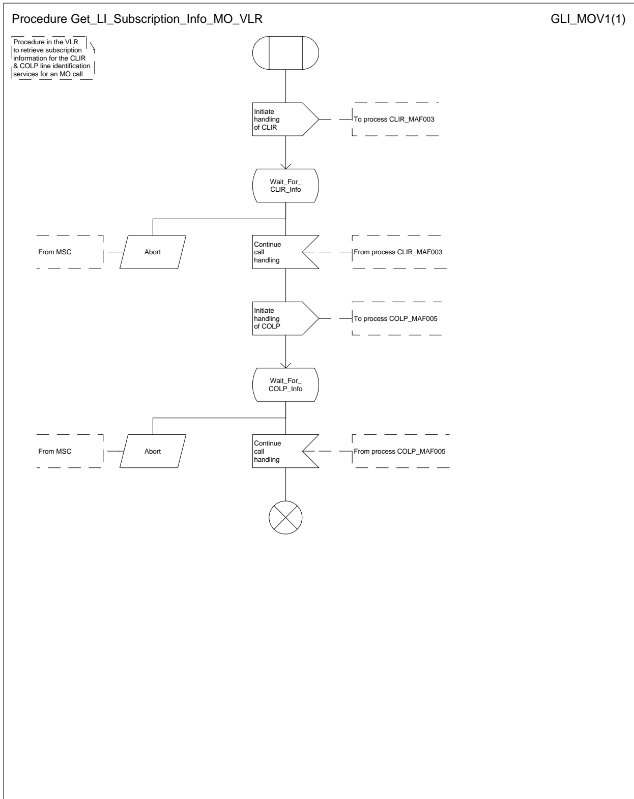
Figure 32: Procedure Get_LI_Subscription_Info_MO_VLR
