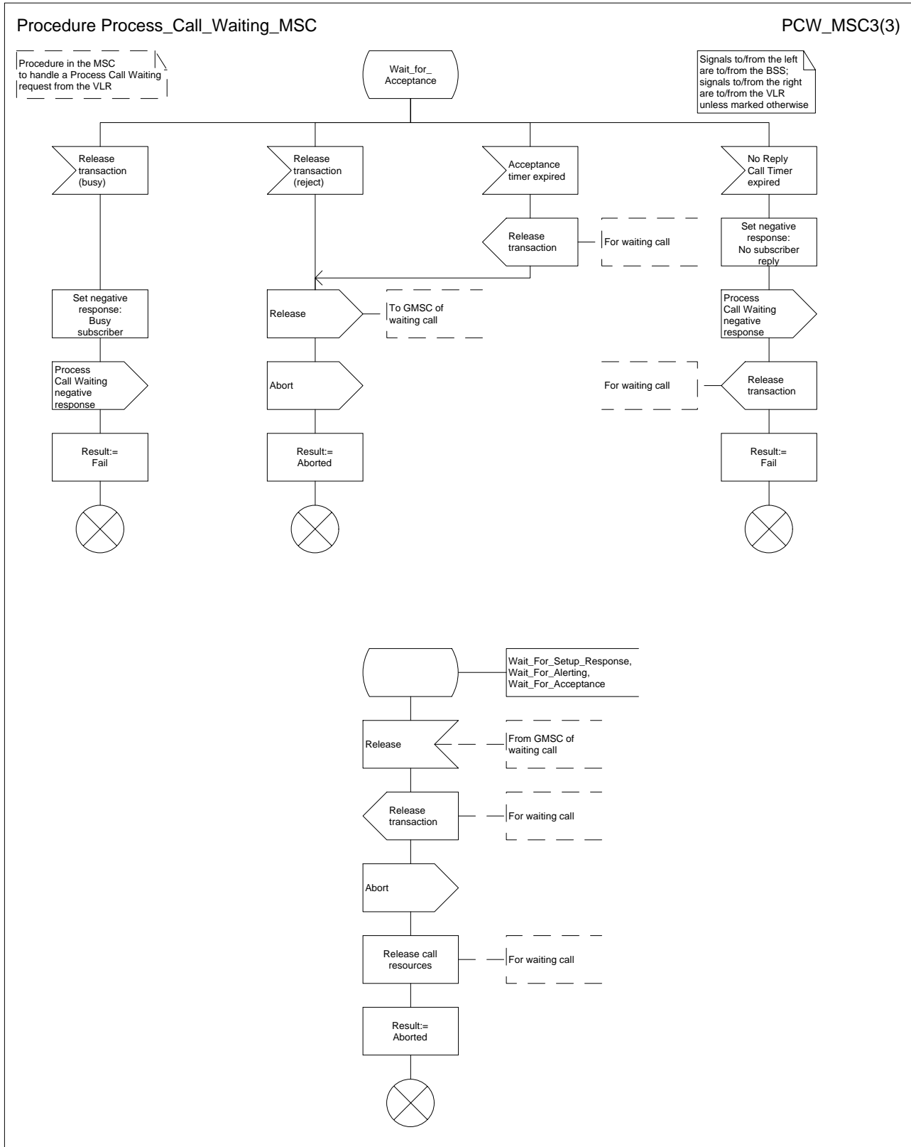
Figure 62c: Procedure Process_Call_Waiting_MSC(sheet 3)
