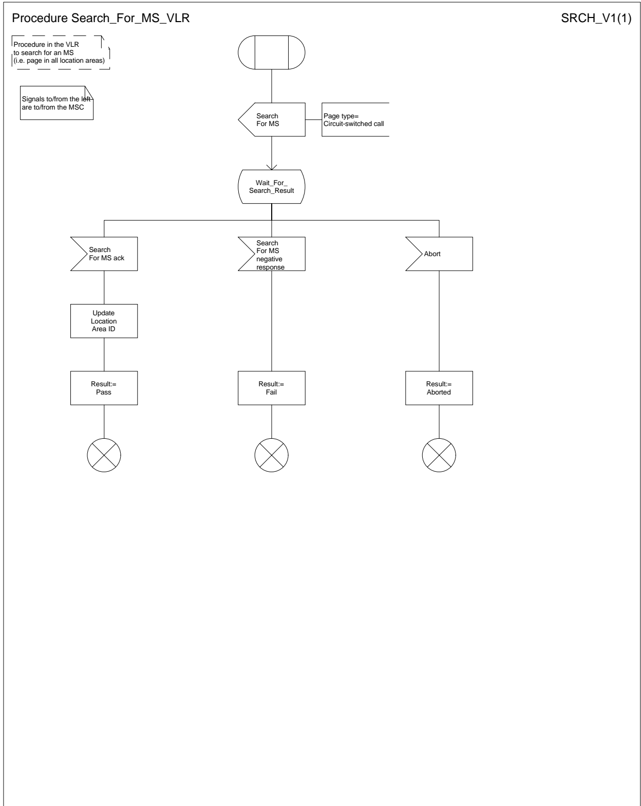
Figure 70: Procedure Search_For_MS_VLR
