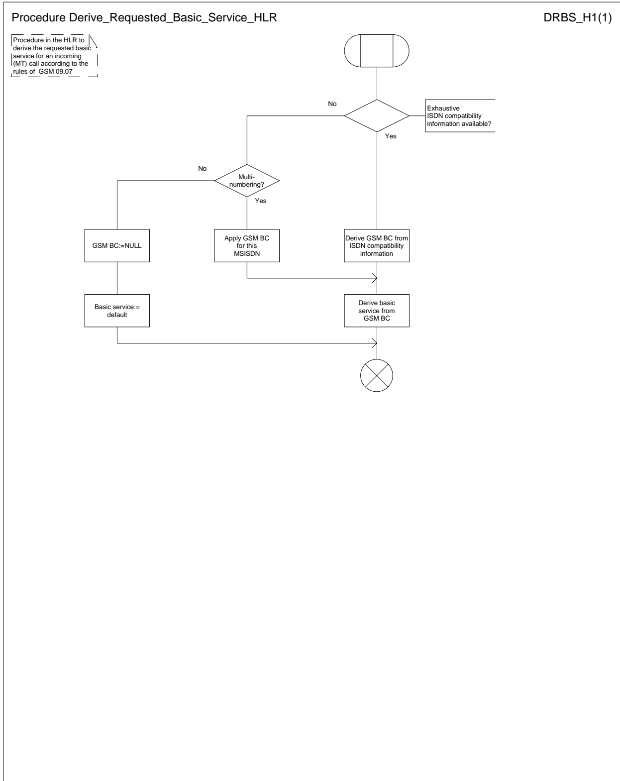
Figure 49: Procedure Derive_Requested_Basic_Service_HLR
