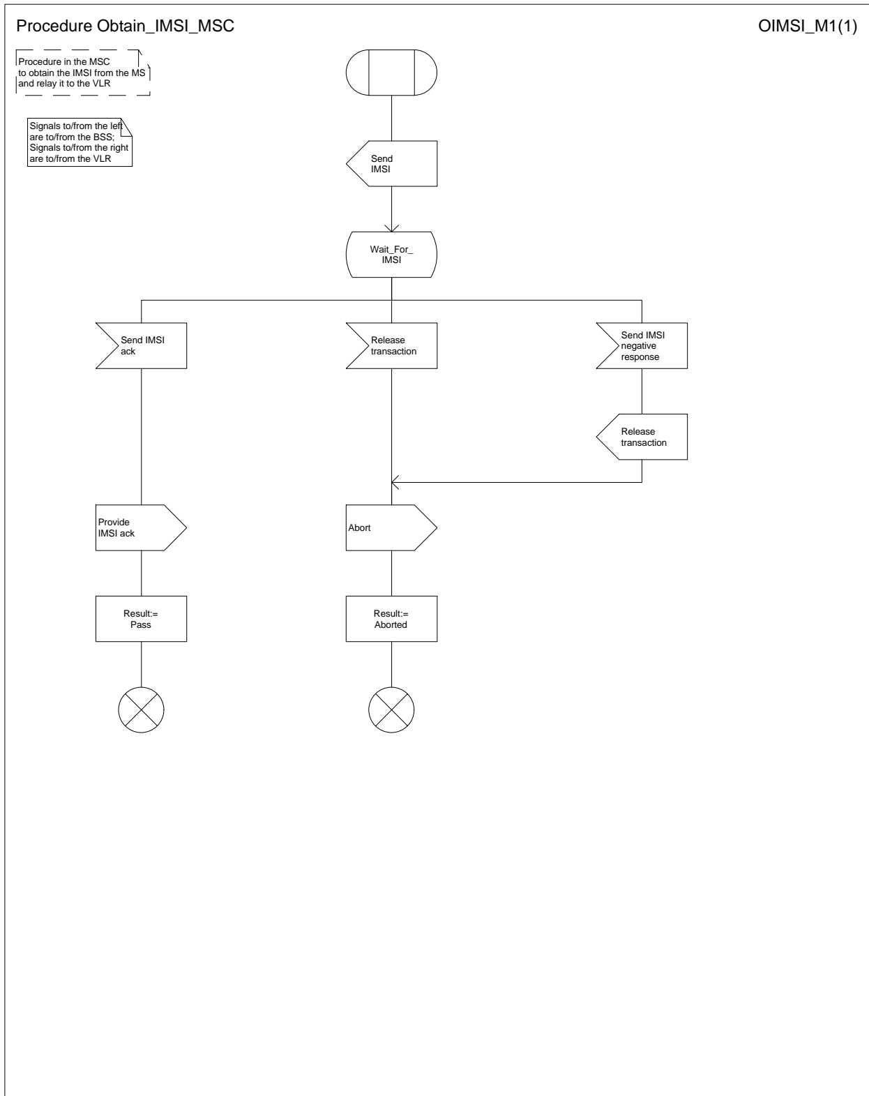
Figure 9: Procedure Obtain_IMSI_MSC
