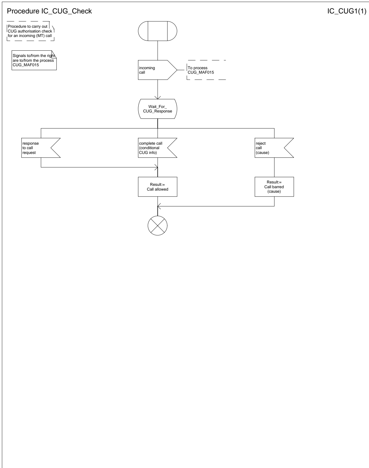
Figure 51: Procedure IC_CUG_Check
