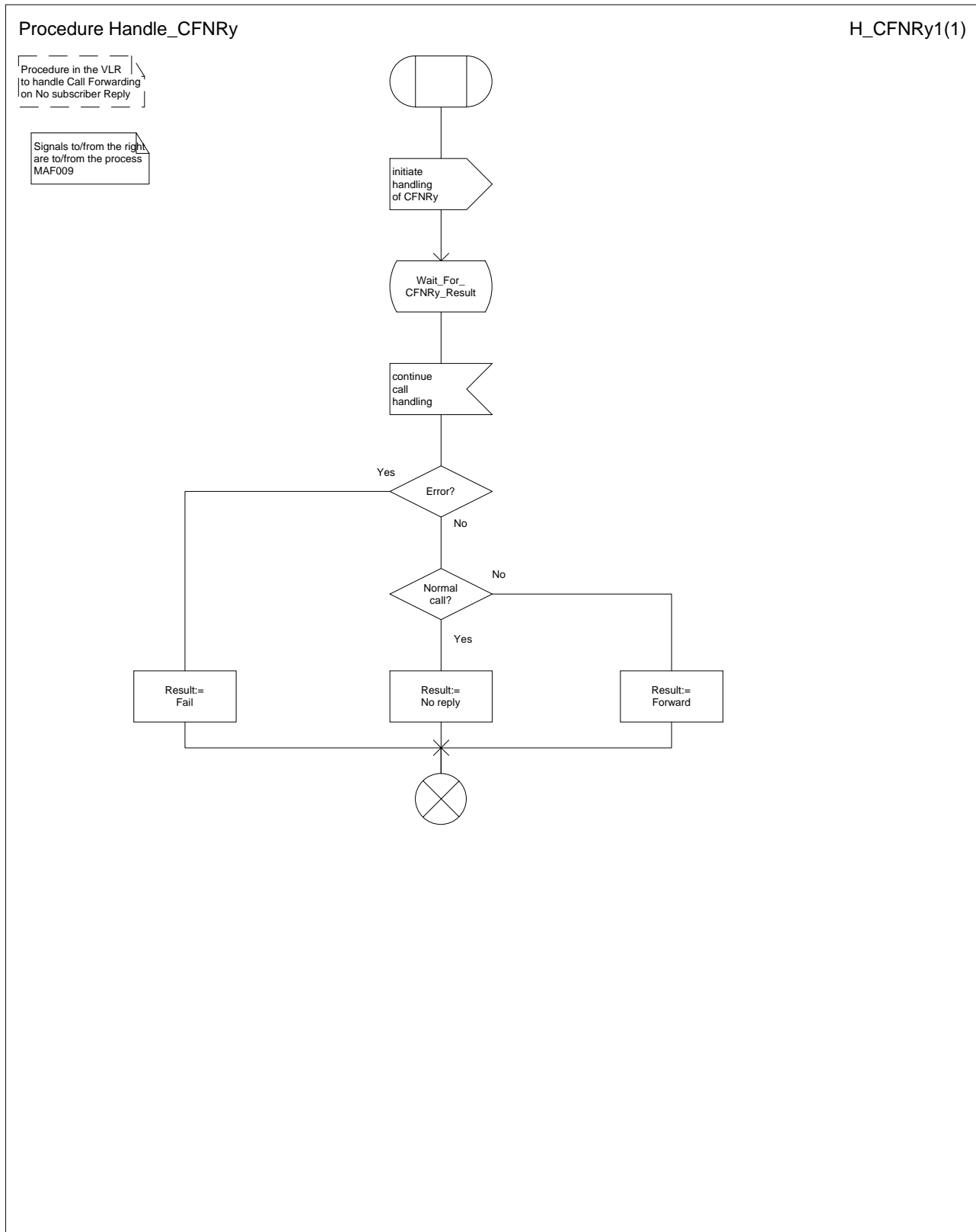
Figure 74: Procedure Handle_CFNRy
