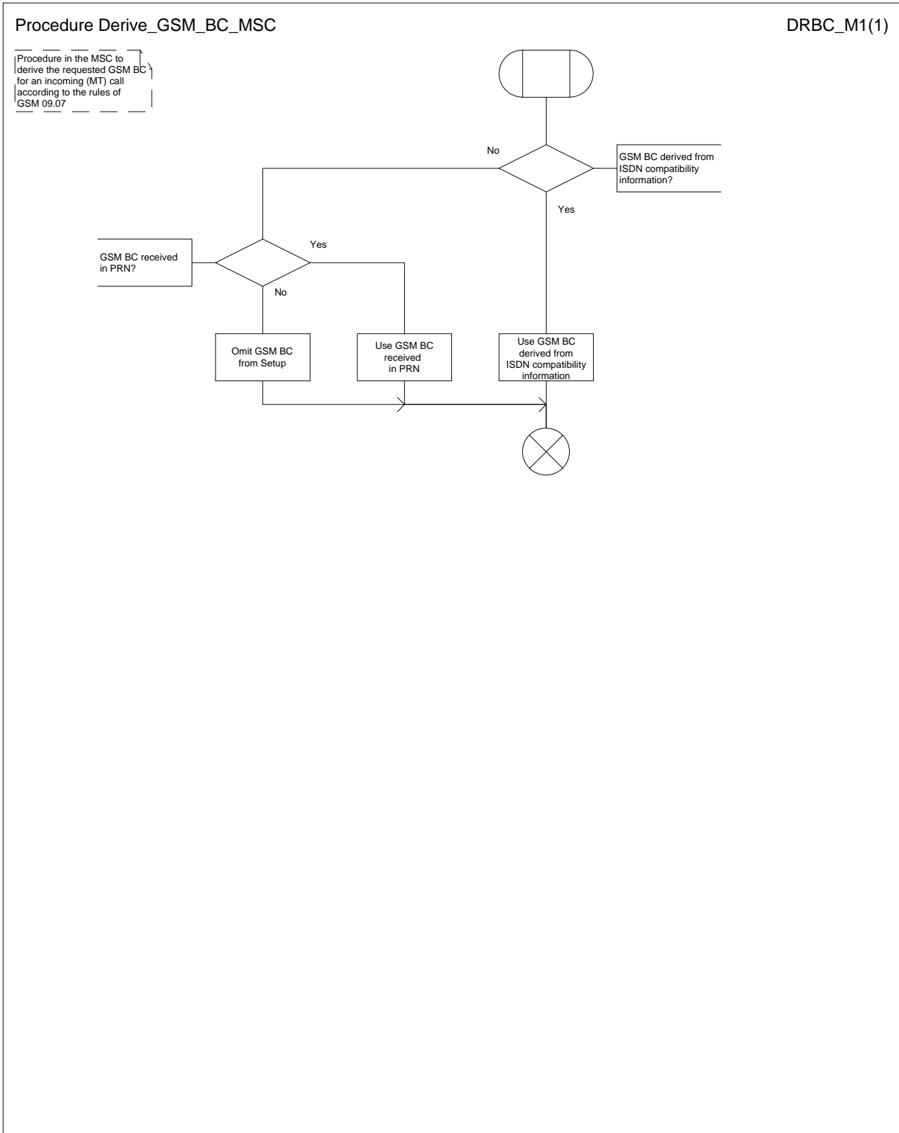
Figure 64: Derive_GSM_BC_MSC
