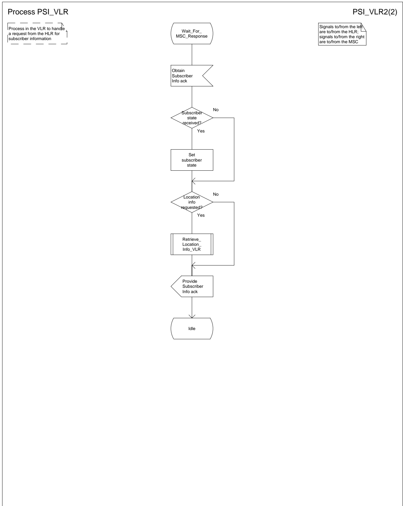
Figure 56b: Process PSI_VLR (sheet 2)
