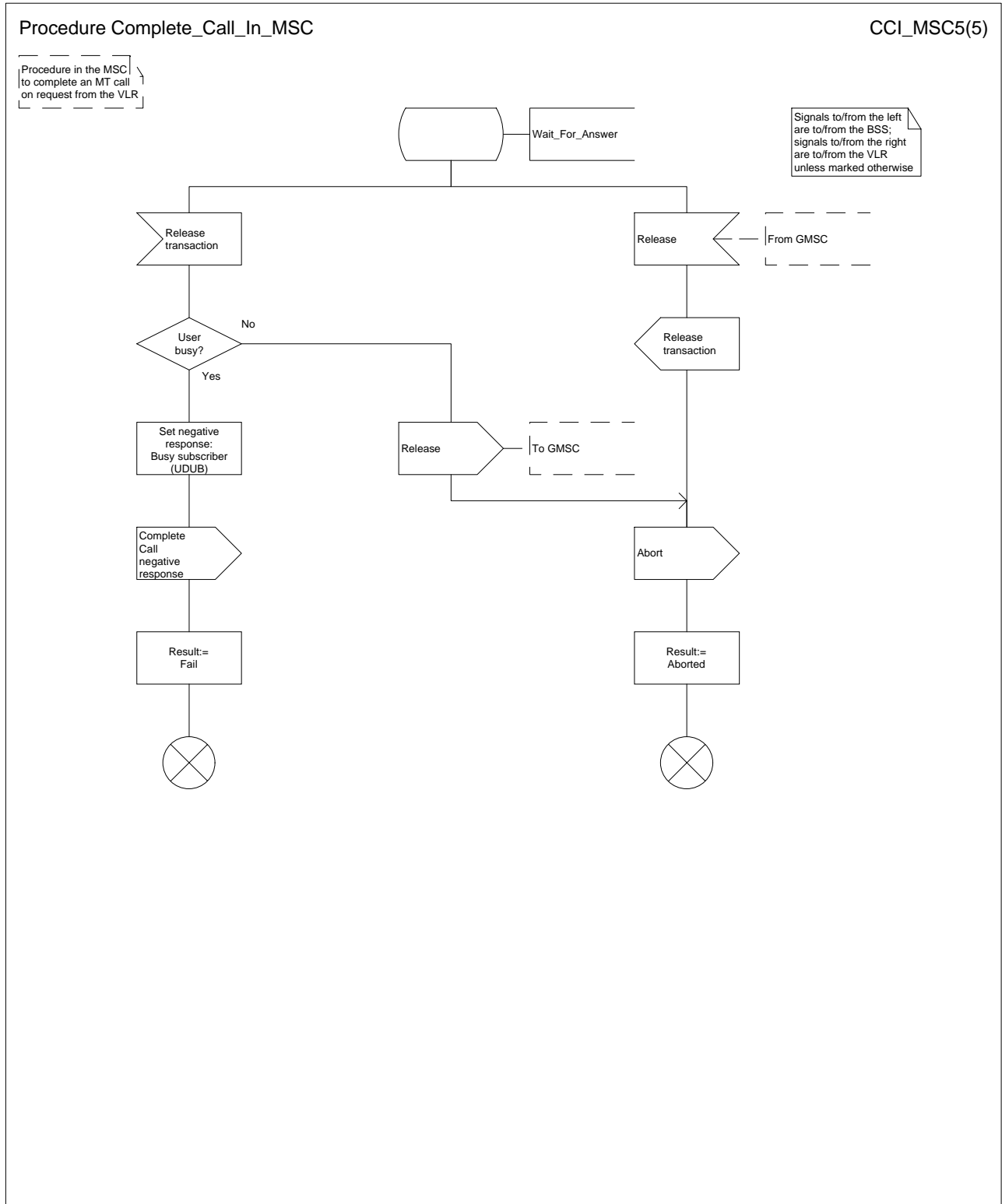
Figure 61e: Procedure Complete_Call_In_MSC (sheet 5)
