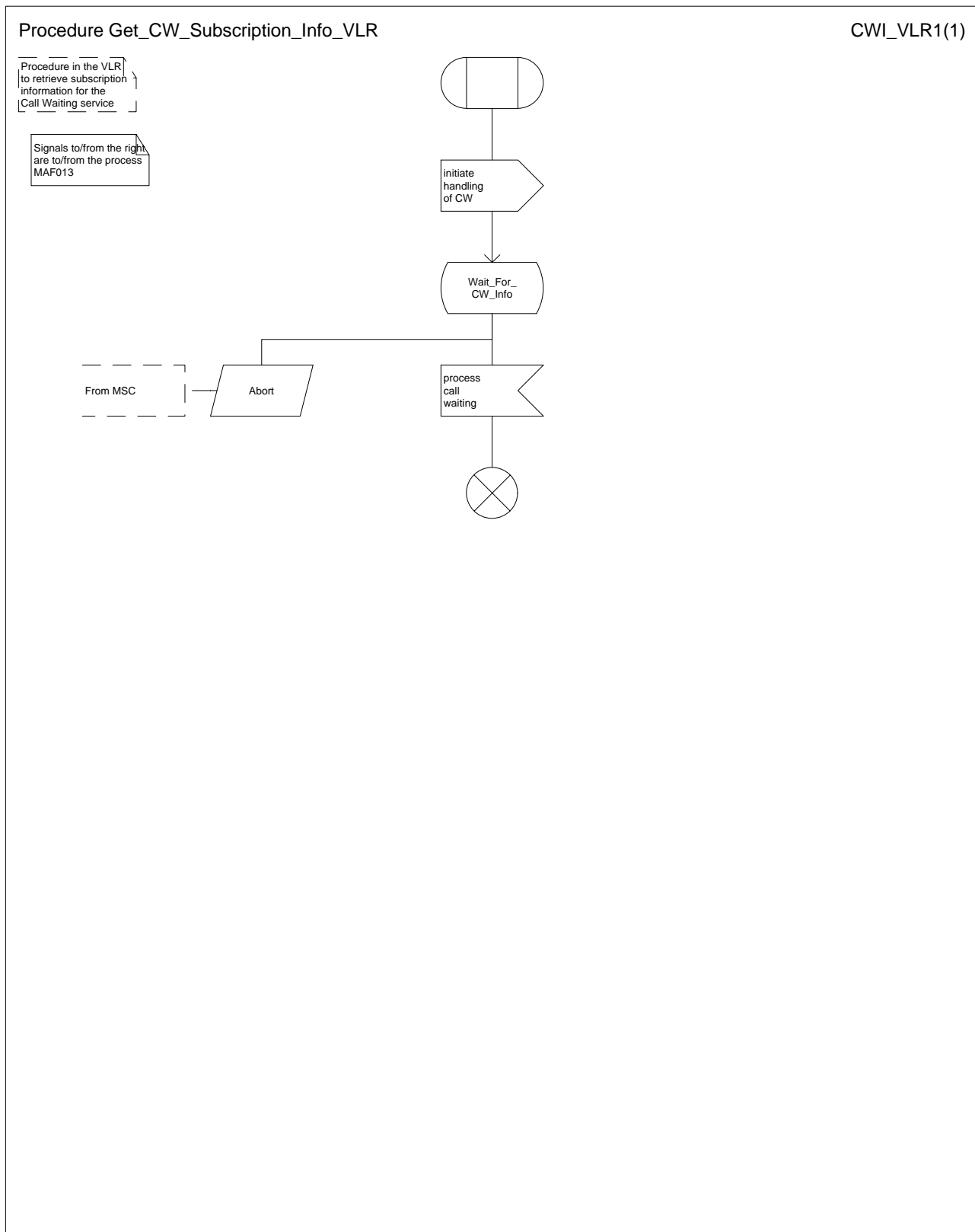
Figure 71: Procedure Get_CW_Subscription_Info_VLR
