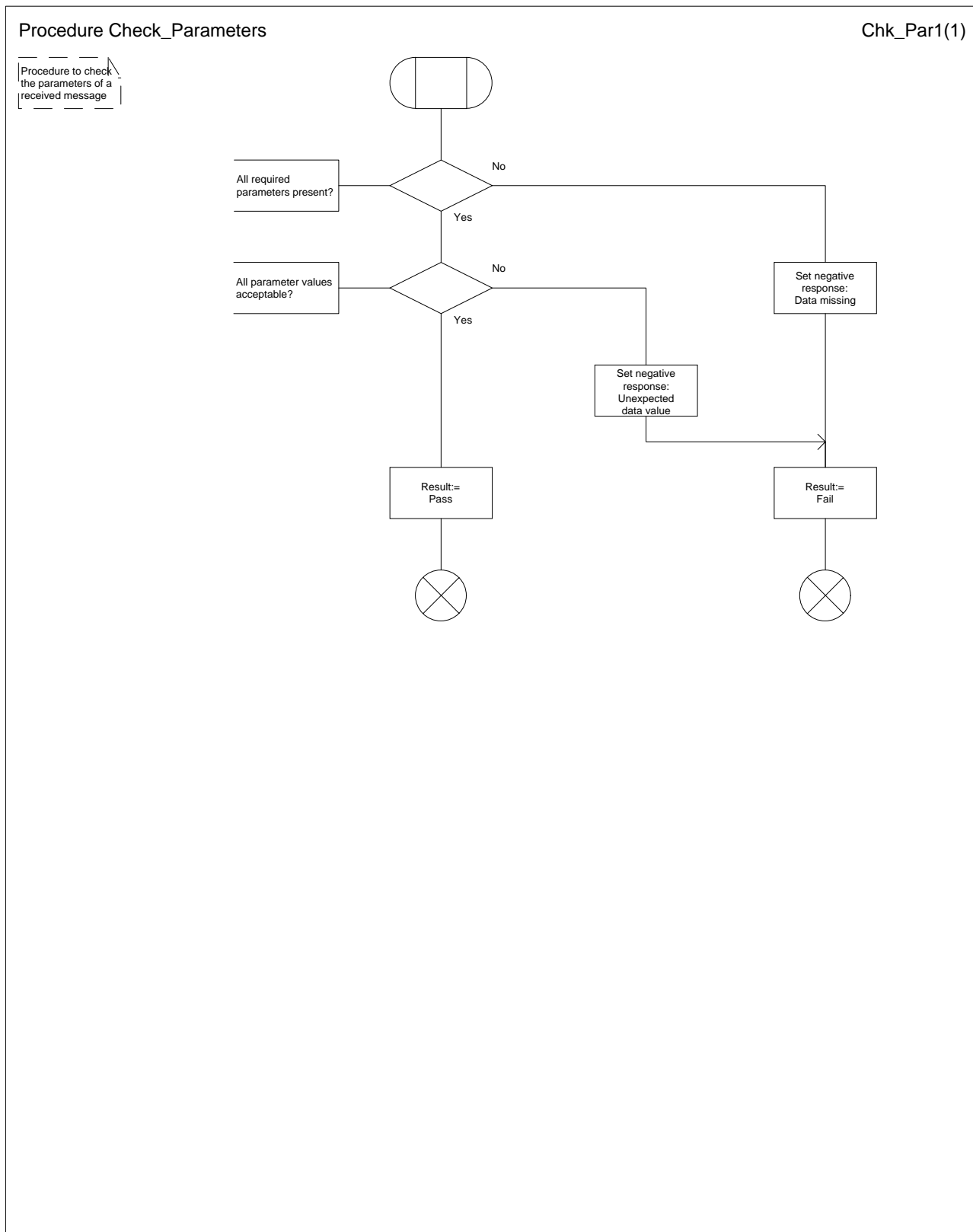
Figure 44: Procedure Check_Parameters
