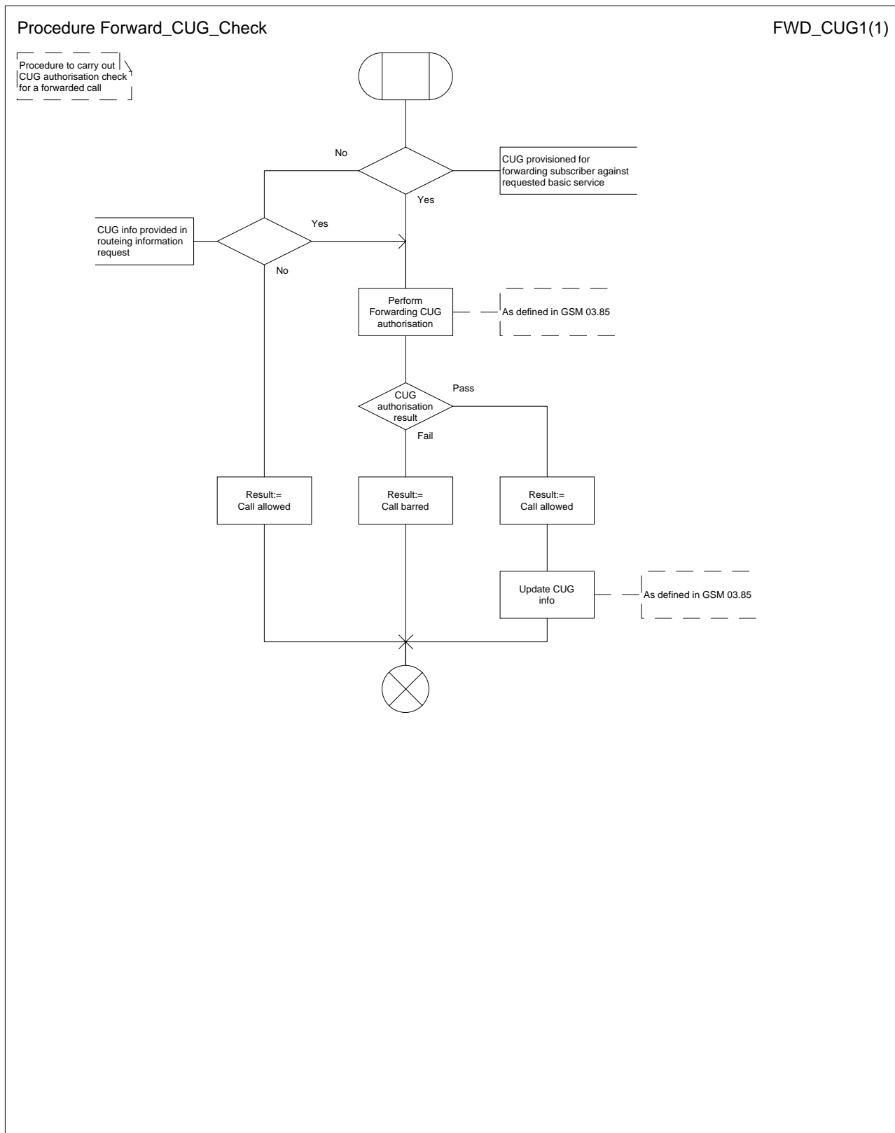
Figure 48: Procedure Forward_CUG_Check
