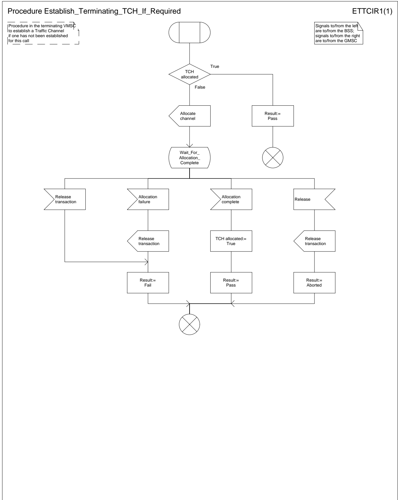
Figure 65: Procedure Establish_Terminating_TCH_If_Required
