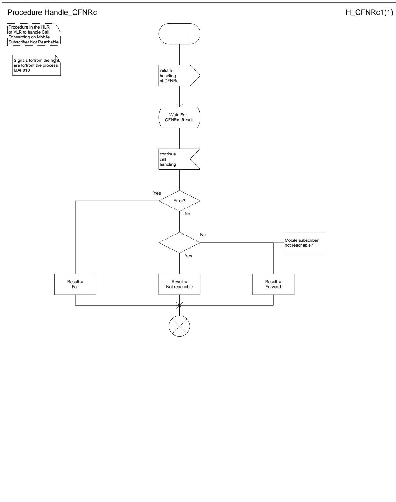
Figure 53: Procedure Handle_CFNRc
