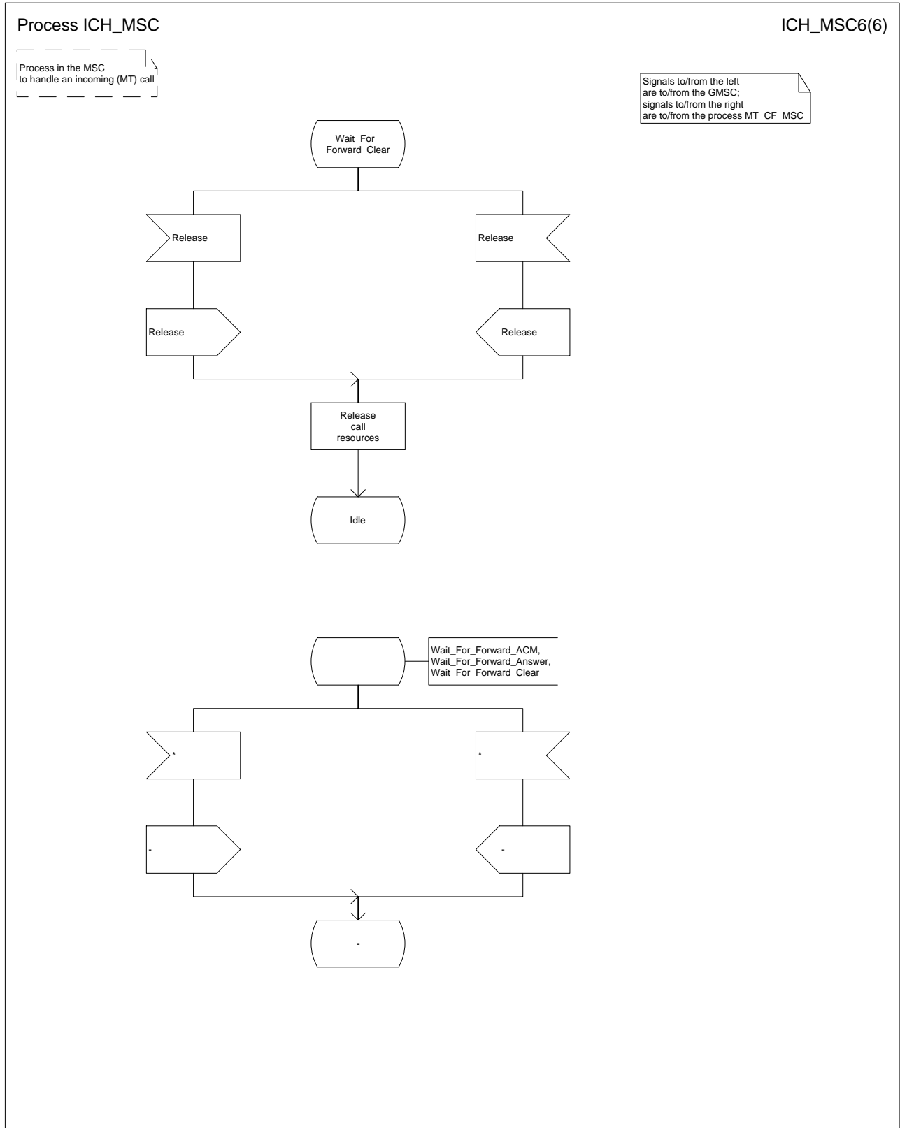
Figure 58f: Process ICH_MSC (sheet 6)
