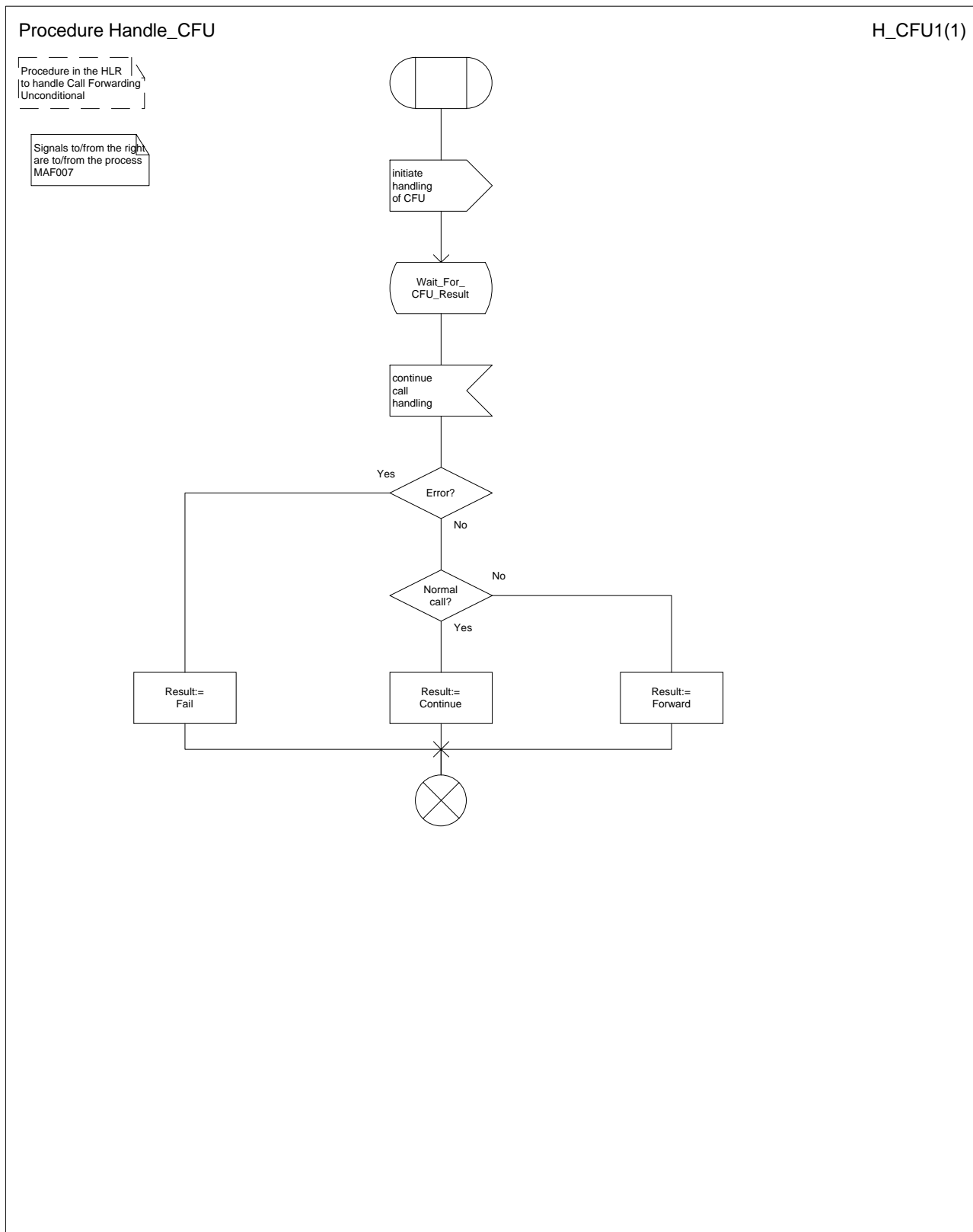
Figure 52: Procedure Handle_CFU
