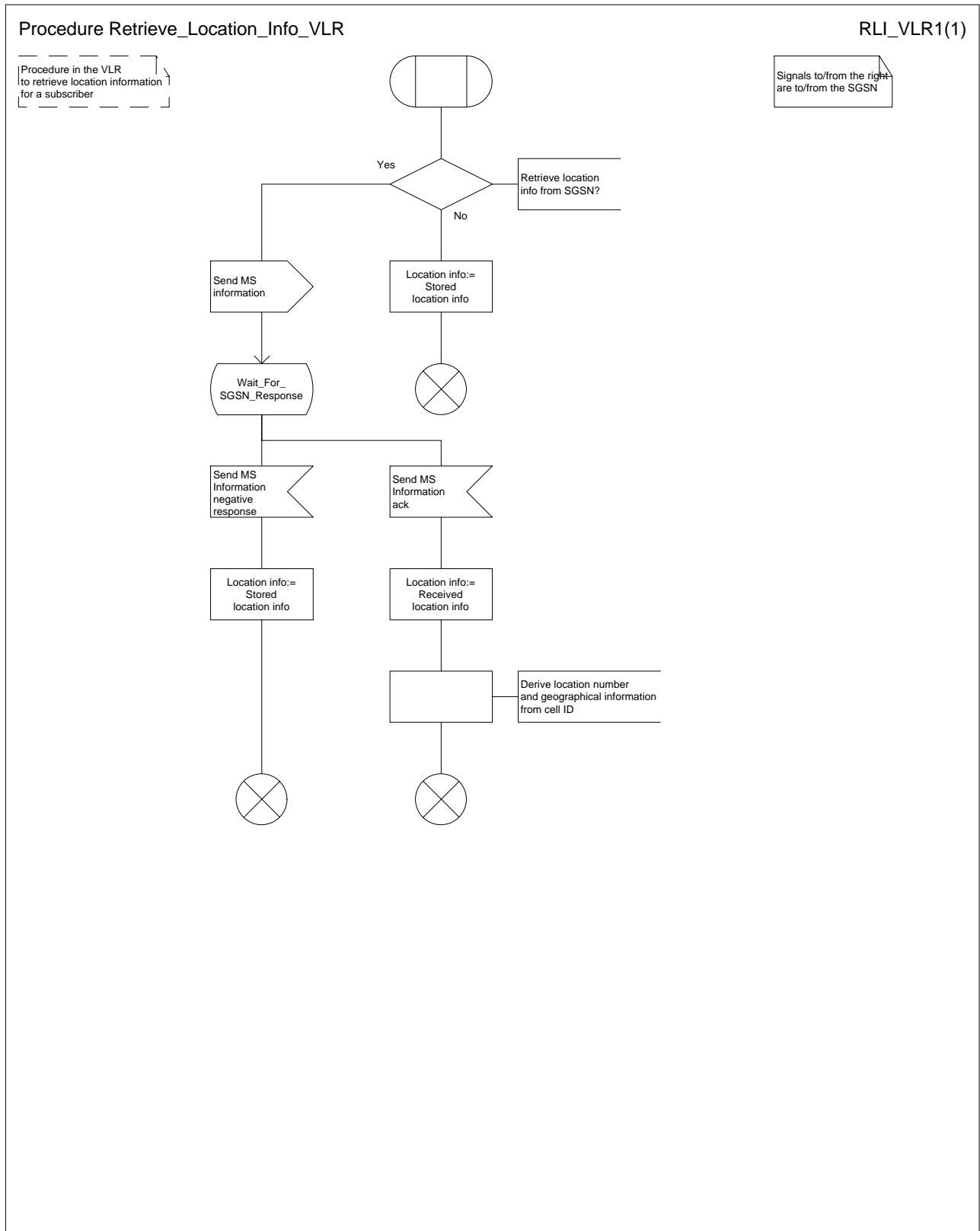
Figure 57: Procedure Retrieve_Location_Info_VLR
