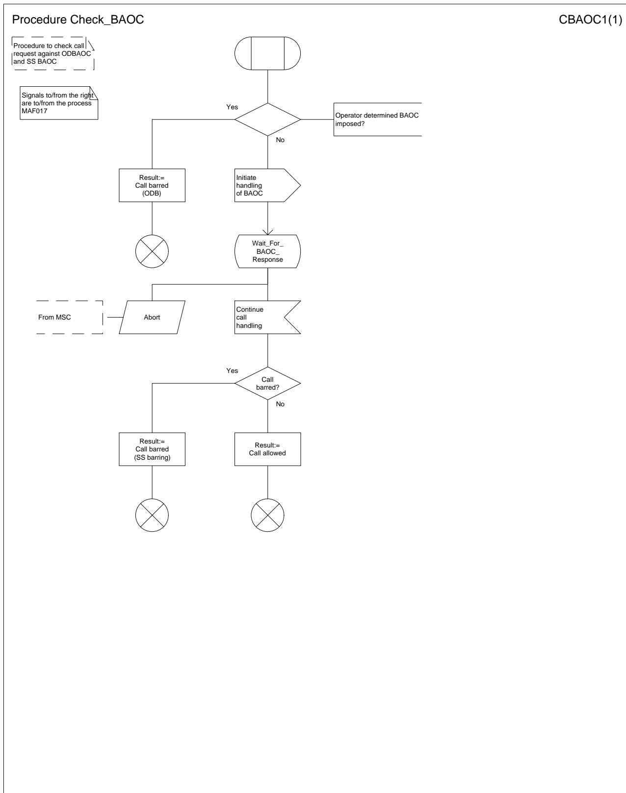
Figure 30: Procedure Check_BAOC
