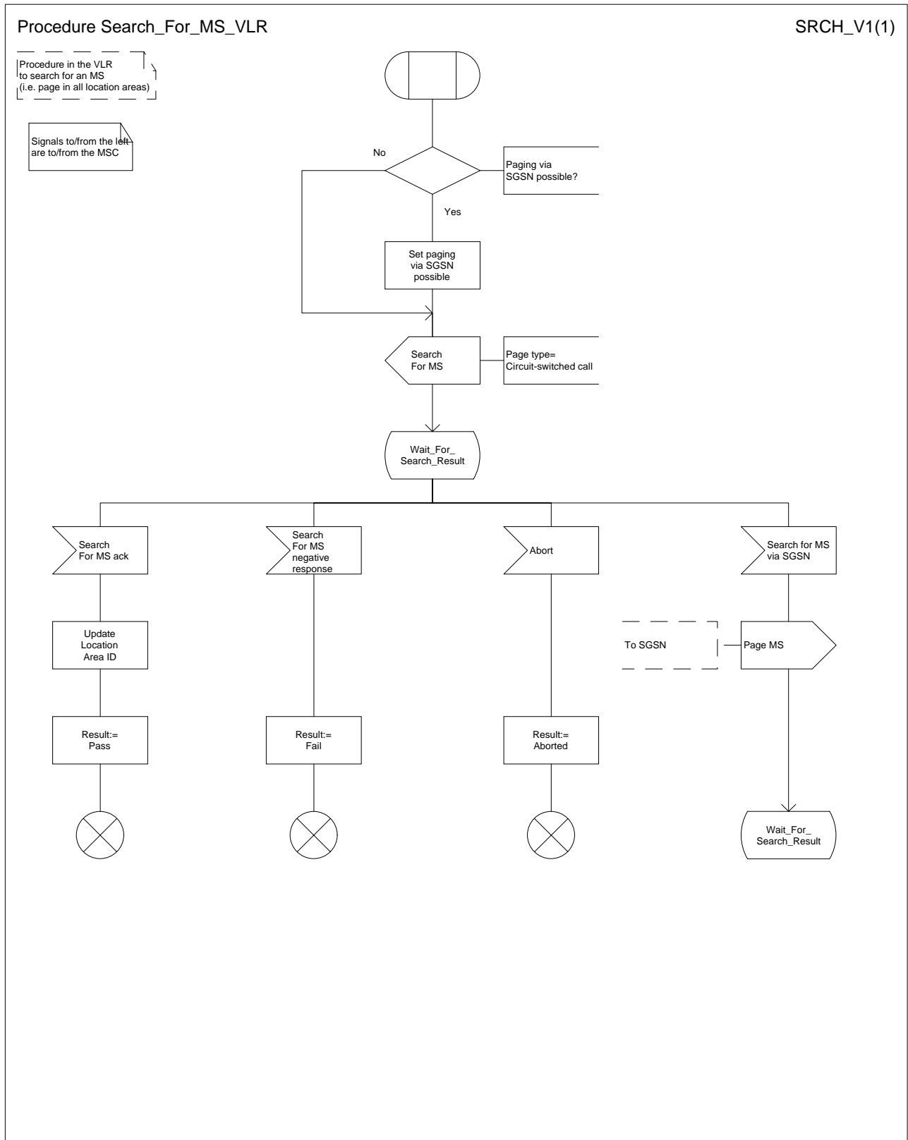
Figure 70: Procedure Search_For_MS_VLR
