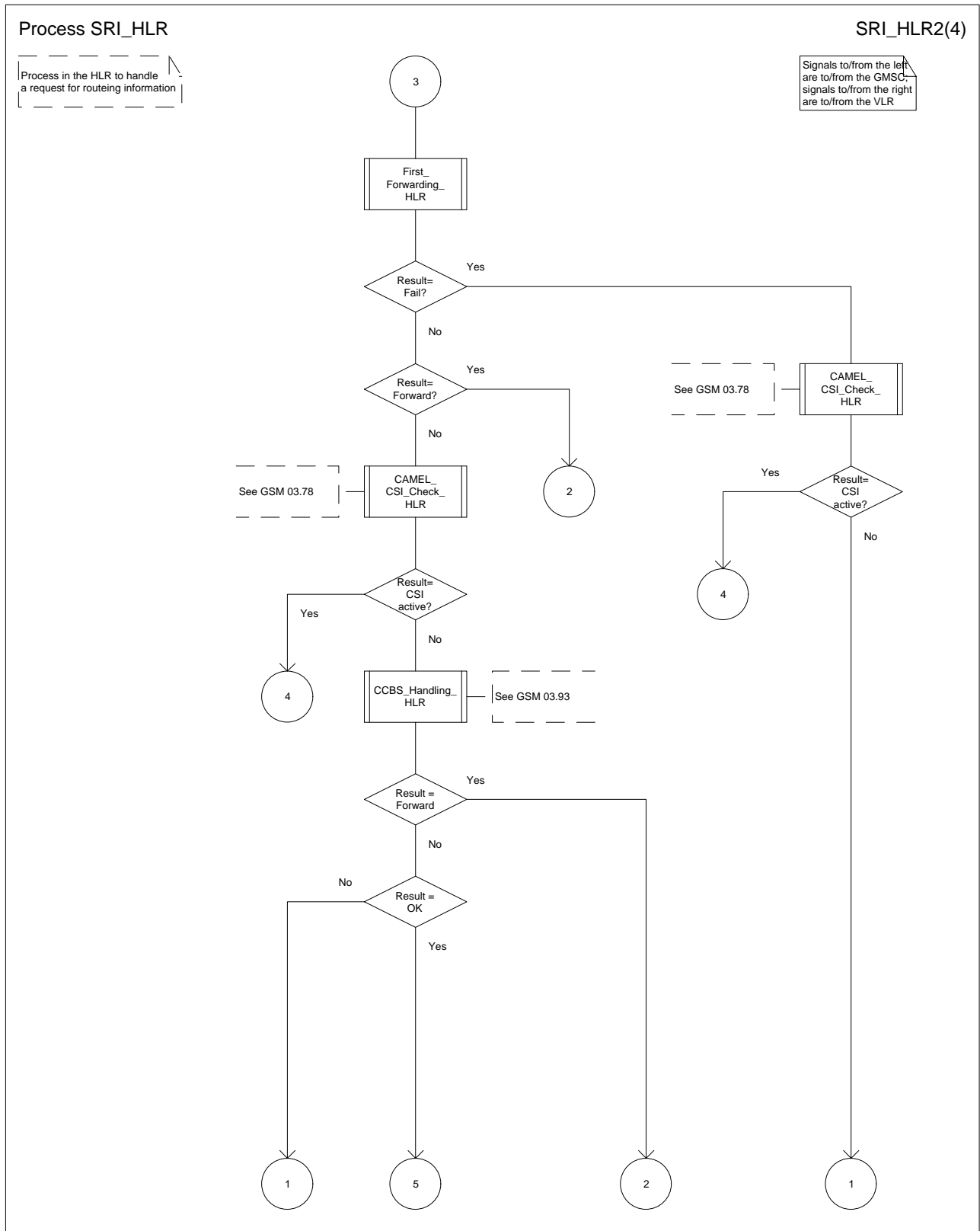
Figure 43b: Process SRI_HLR (sheet 2)
