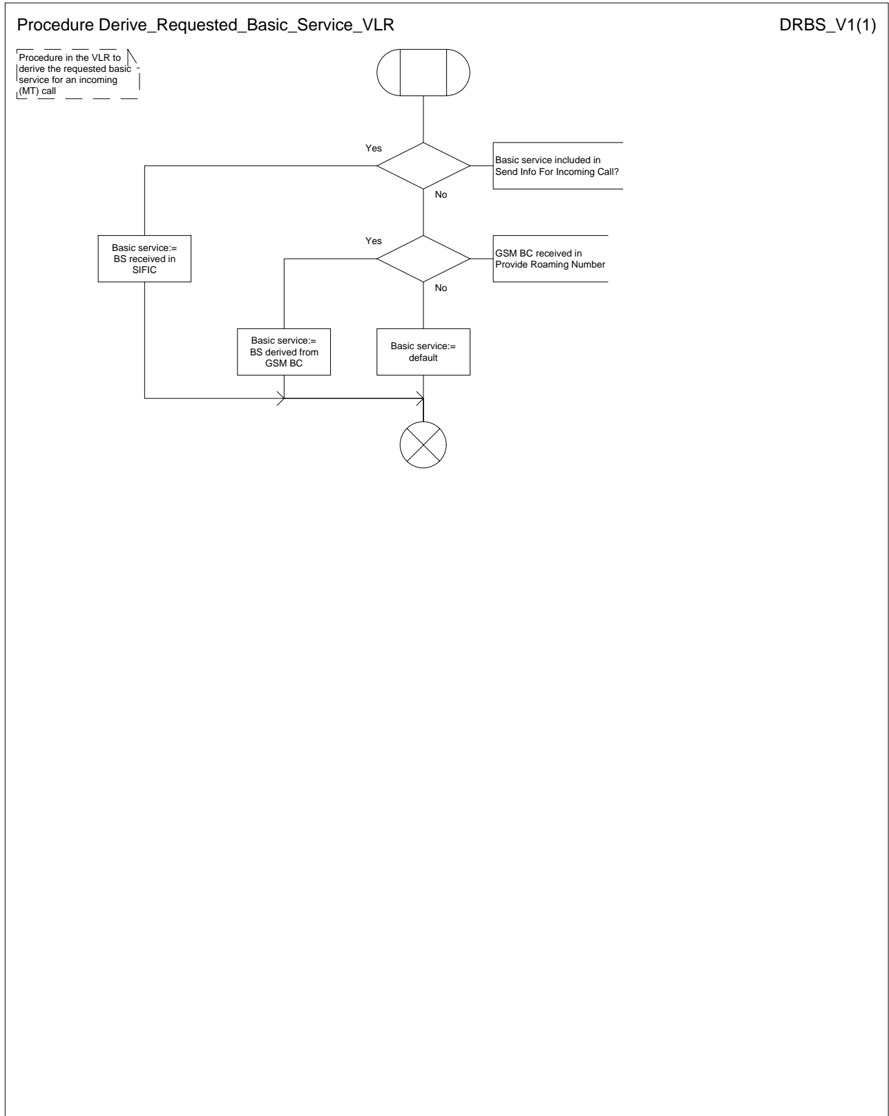
Figure 69: Procedure Derive_Requested_Basic_Service_VLR
