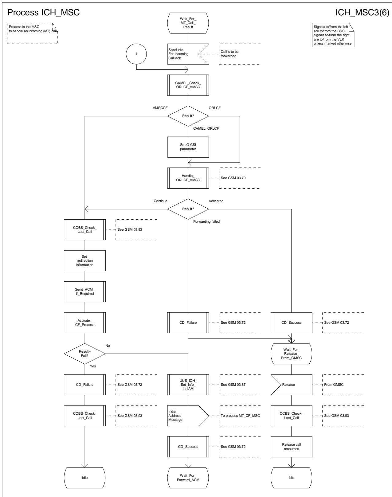
Figure 59c: Process ICH_MSC (sheet 3)
