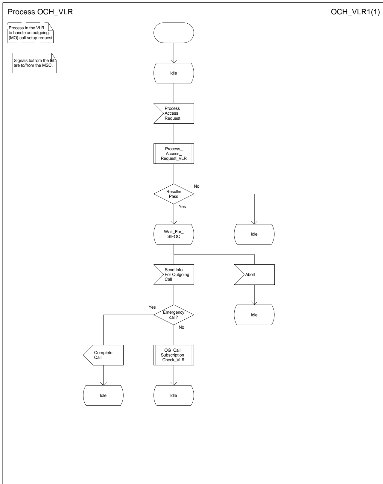
Figure 19: Process OCH_VLR
