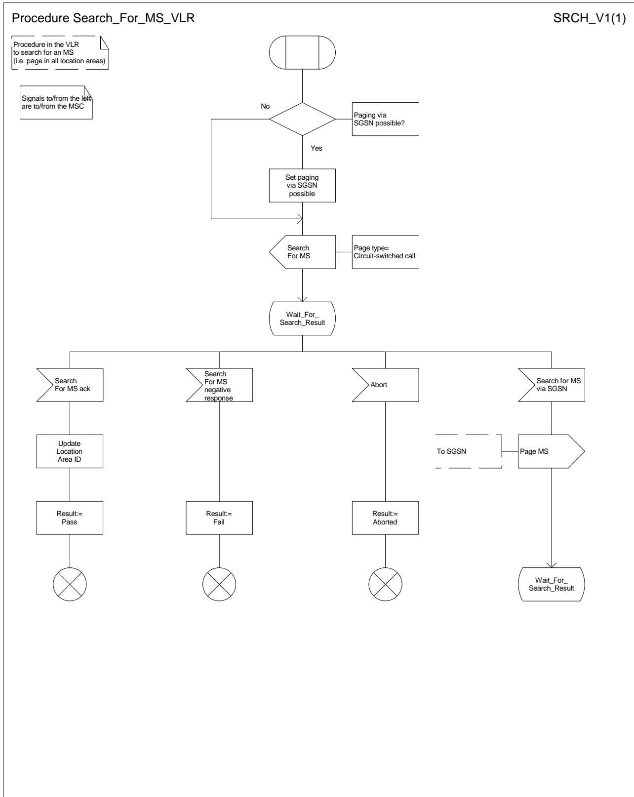
Figure 71: Procedure Search_For_MS_VLR
