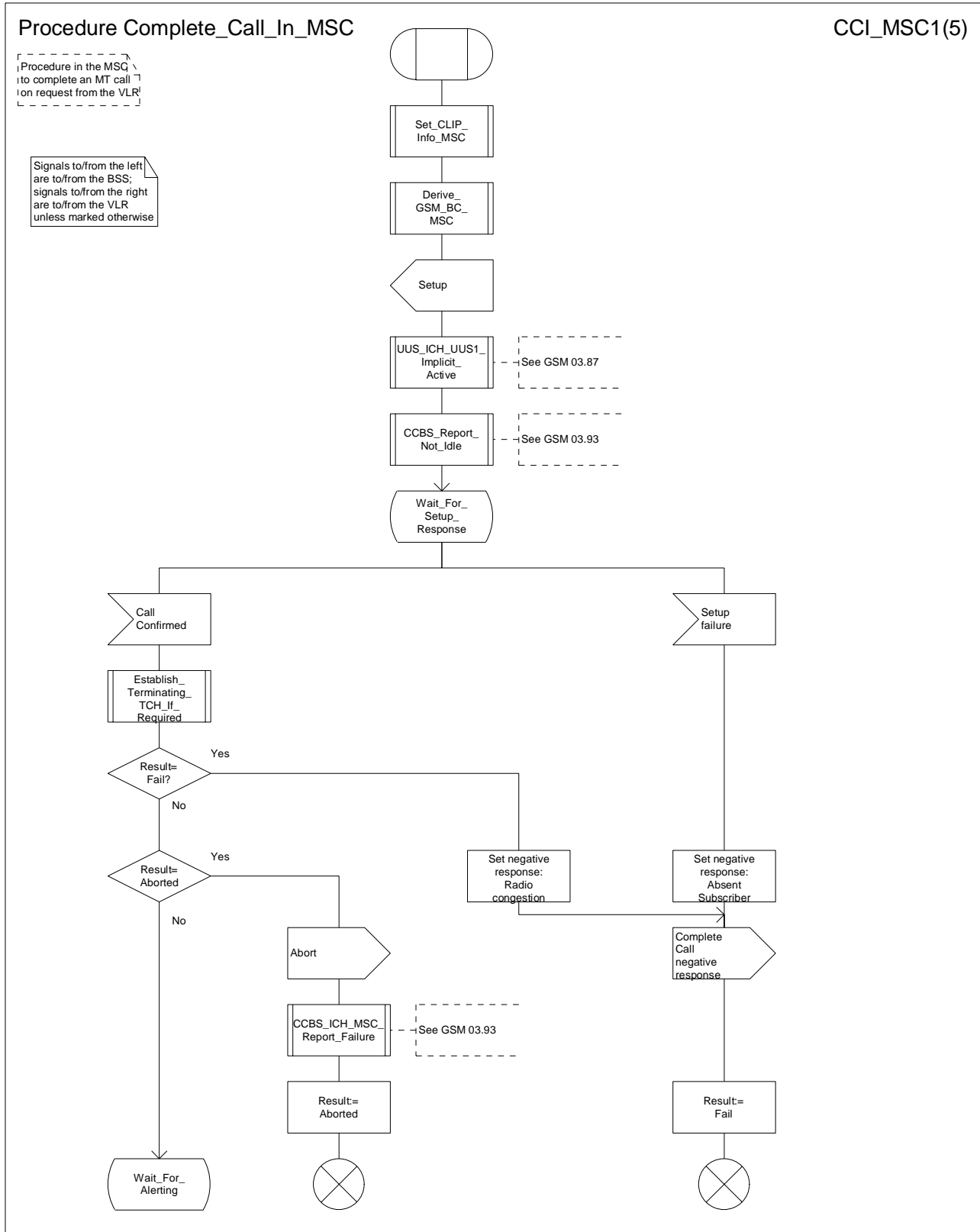
Figure 62a: Procedure Complete_Call_In_MSC (sheet 1)
