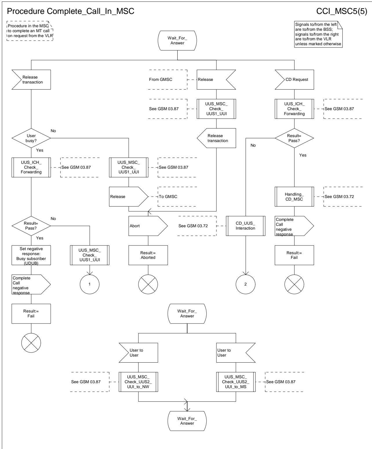
Figure 62e: Procedure Complete_Call_In_MSC (sheet 5)
