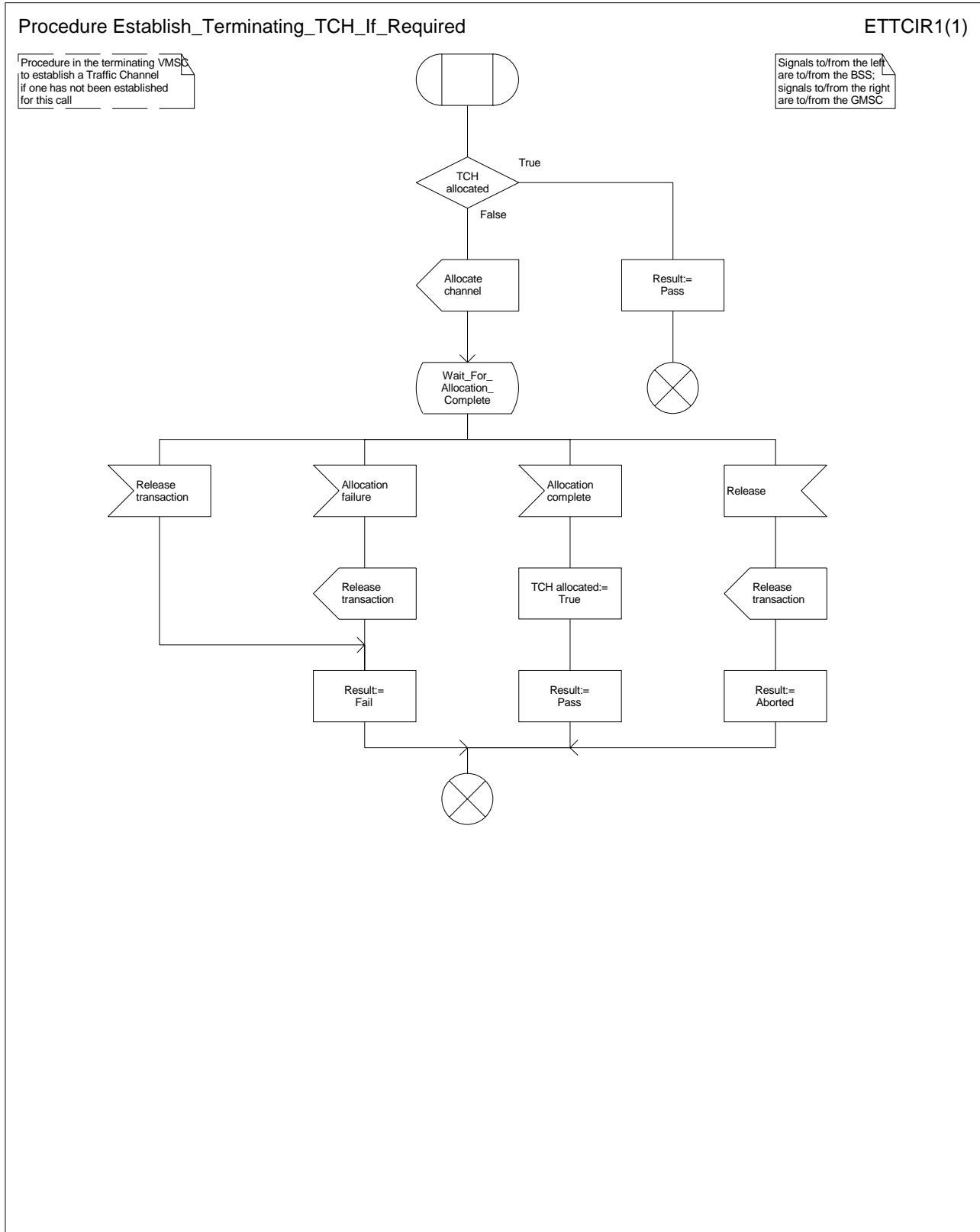
Figure 66: Procedure Establish_Terminating_TCH_If_Required
