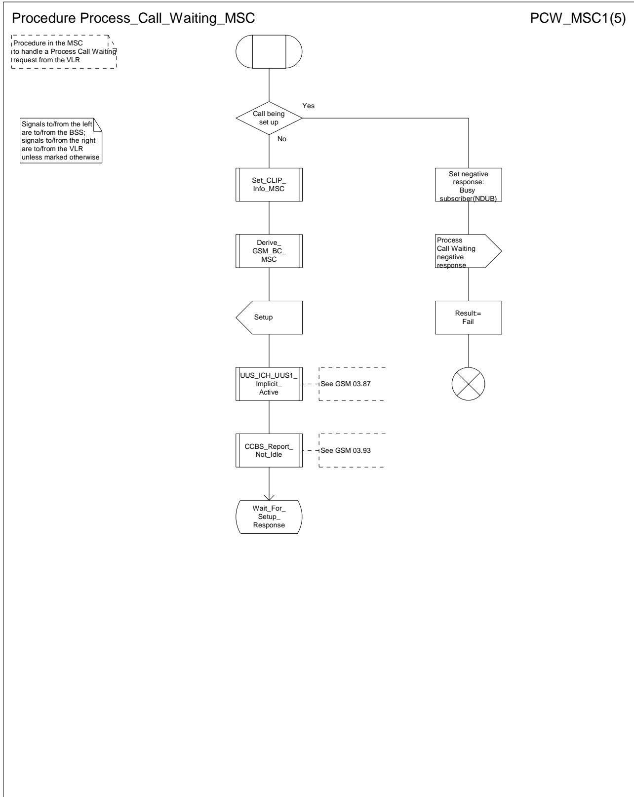
Figure 63a: Procedure Process_Call_Waiting_MSC (sheet 1)
