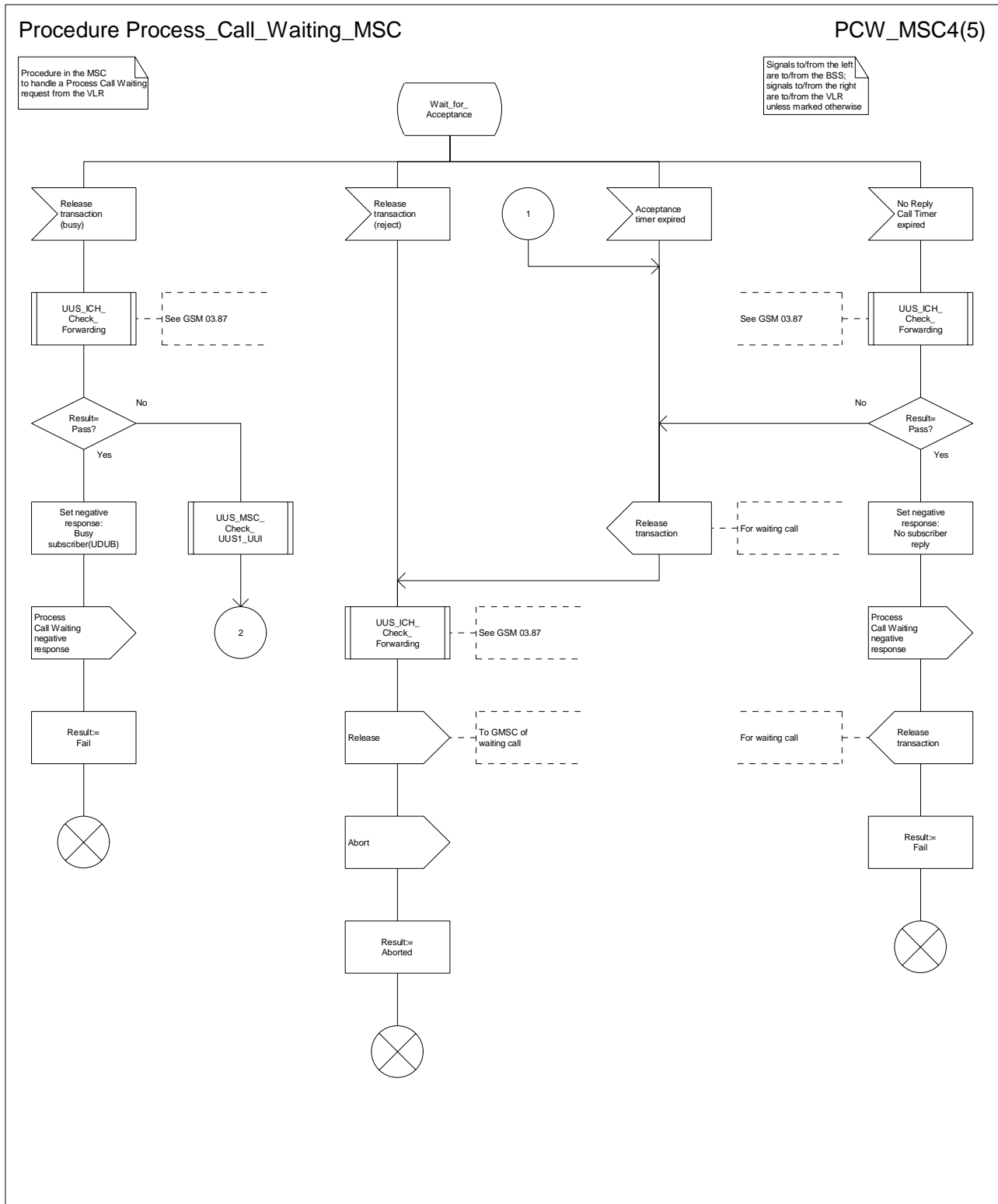
Figure 63d: Procedure Process_Call_Waiting_MSC(sheet 4)
