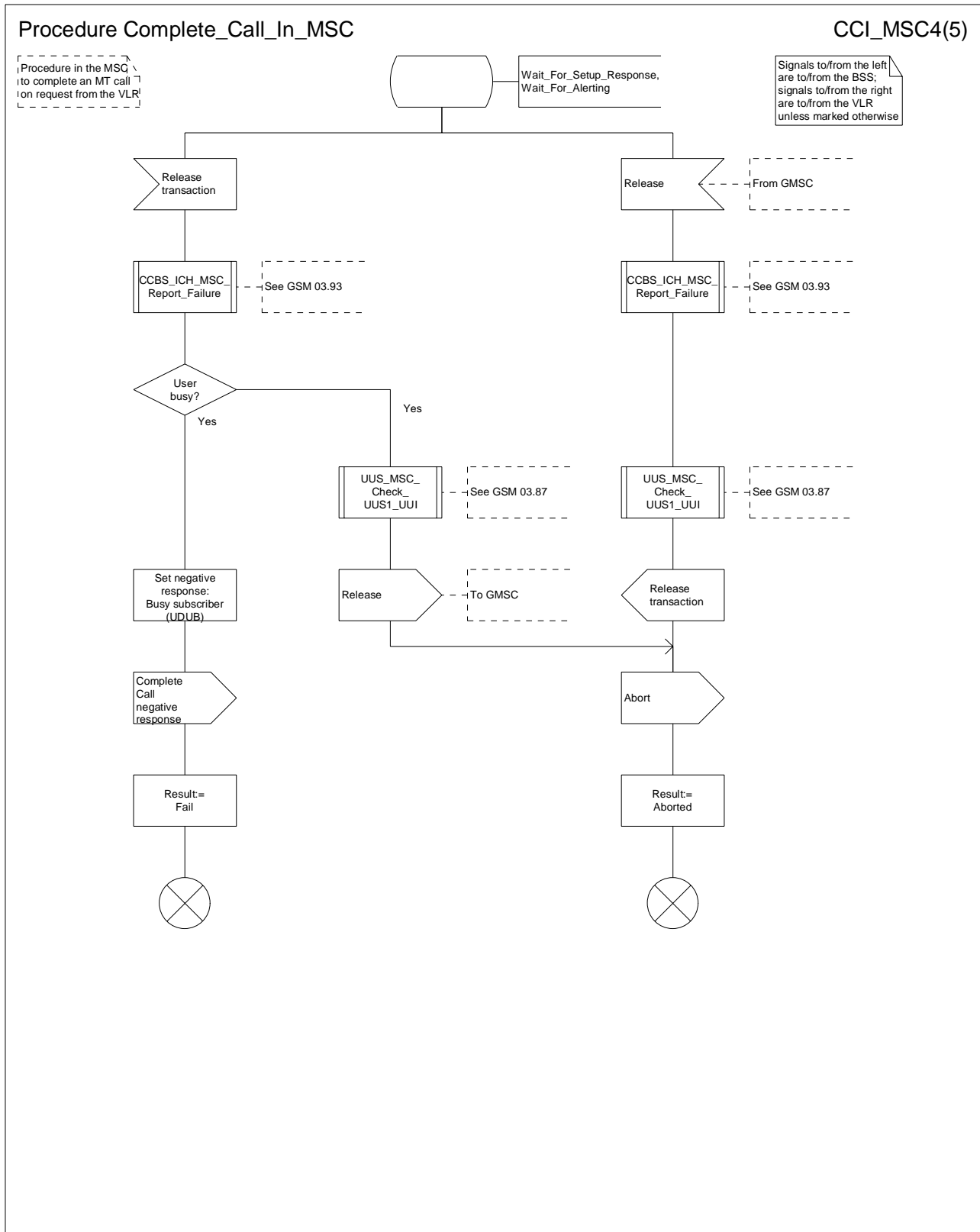
Figure 62d: Procedure Complete_Call_In_MSC (sheet 4)
