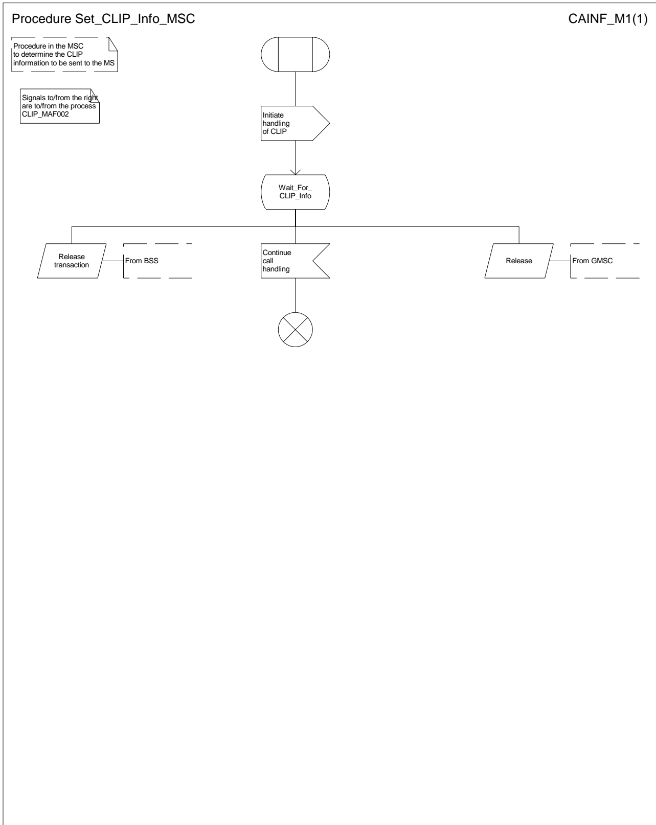
Figure 64: Procedure Set_CLIP_Info_MSC
