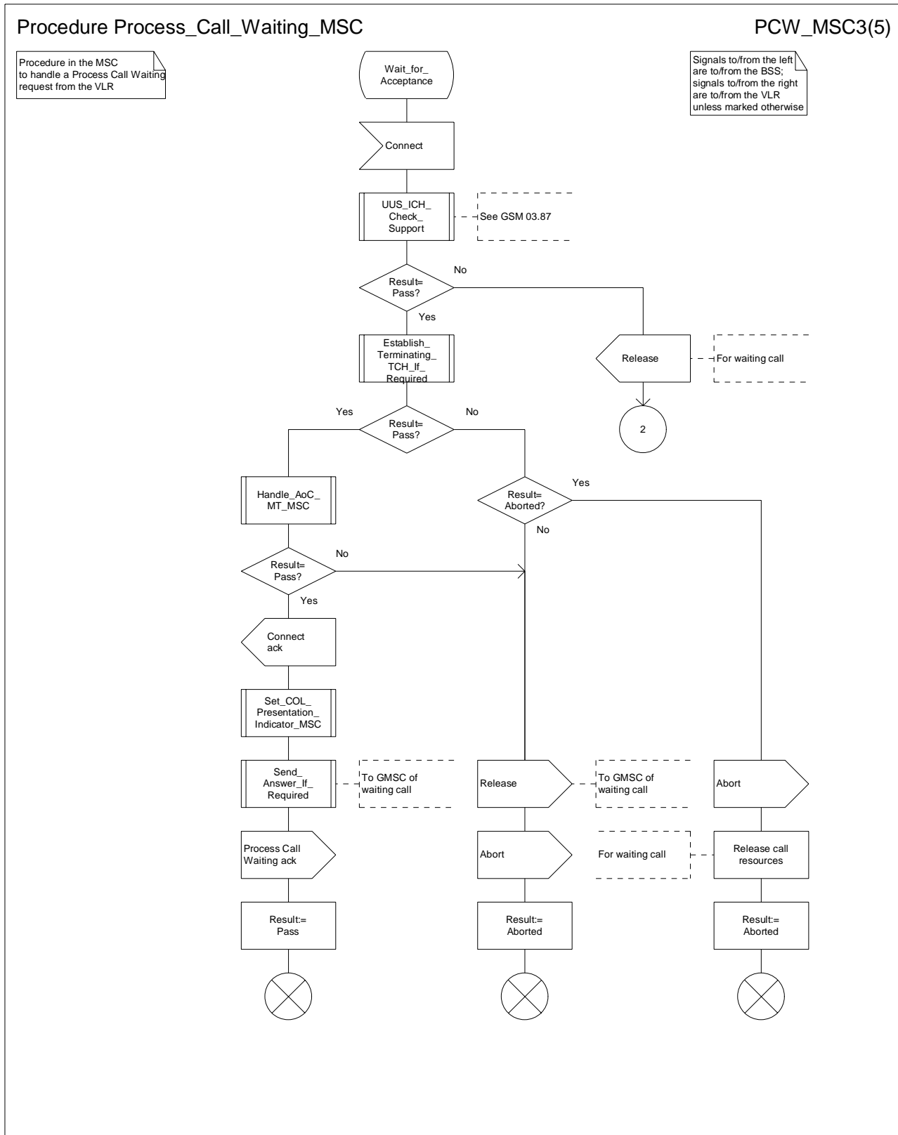
Figure 63c: Procedure Process_Call_Waiting_MSC(sheet 3)
