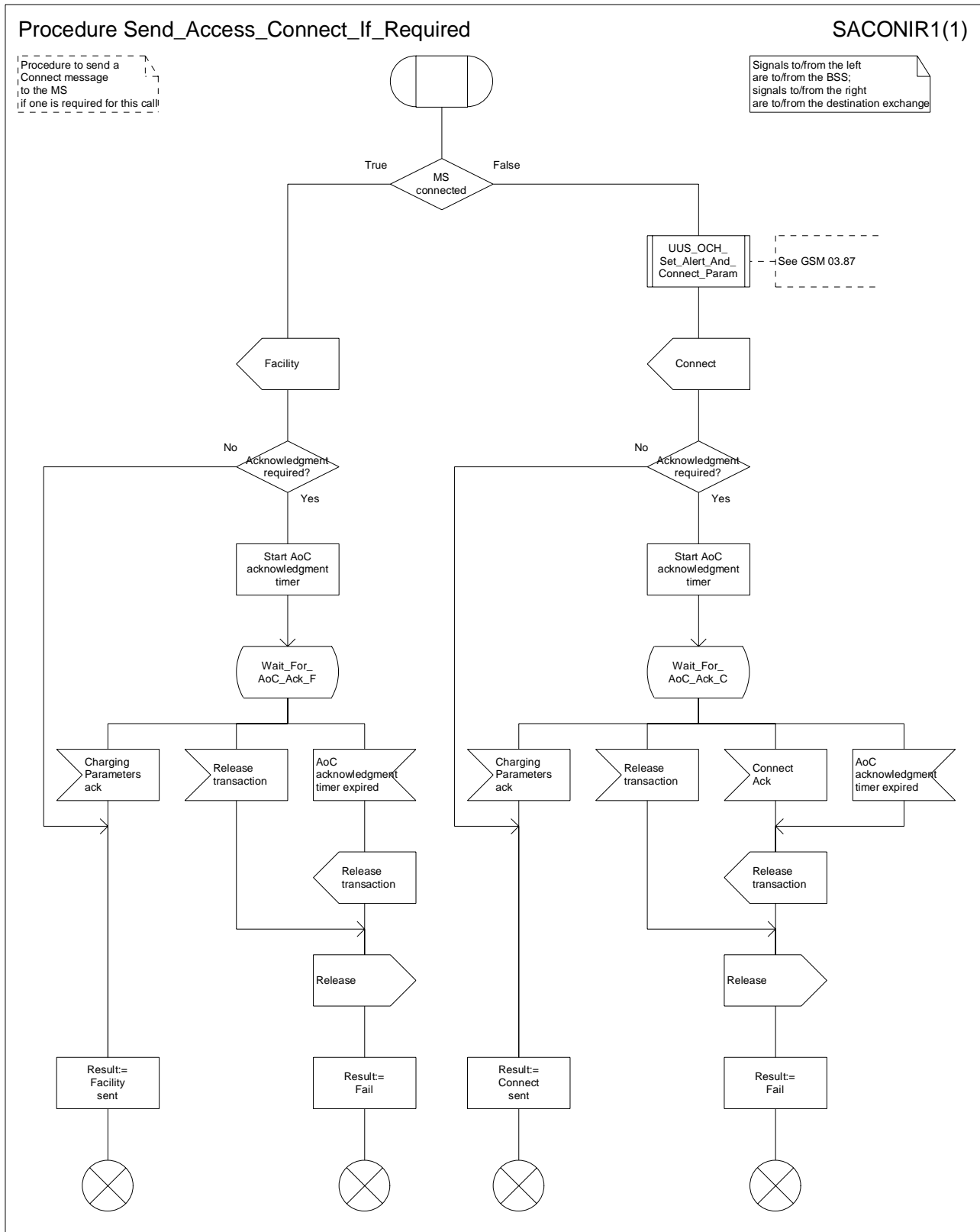
Figure 18: Procedure Send_Access_Connect_If_Required
