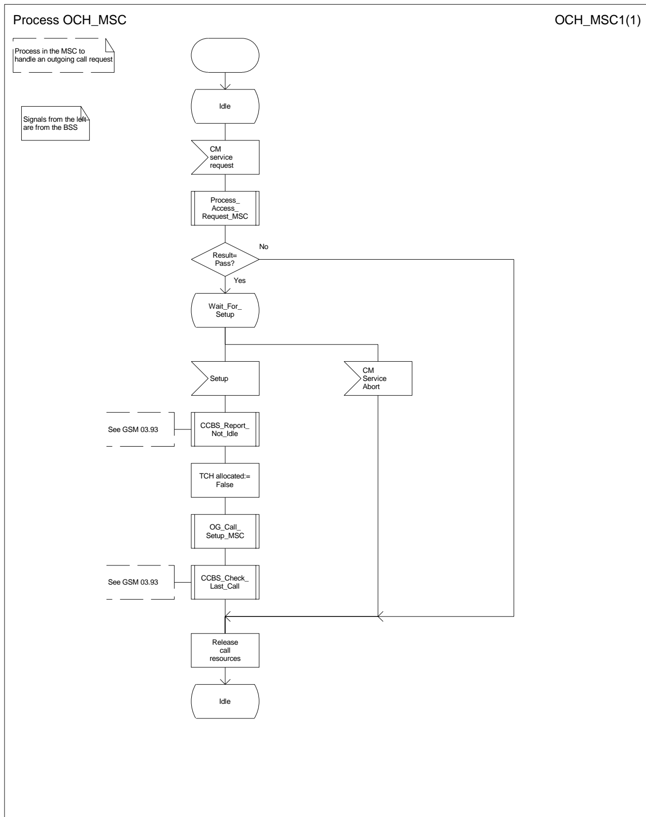
Figure 6: Process OCH_MSC
