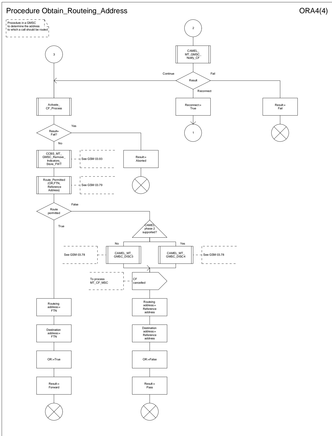
Figure 36d: Procedure Obtain_Routing_Address (sheet 4)
