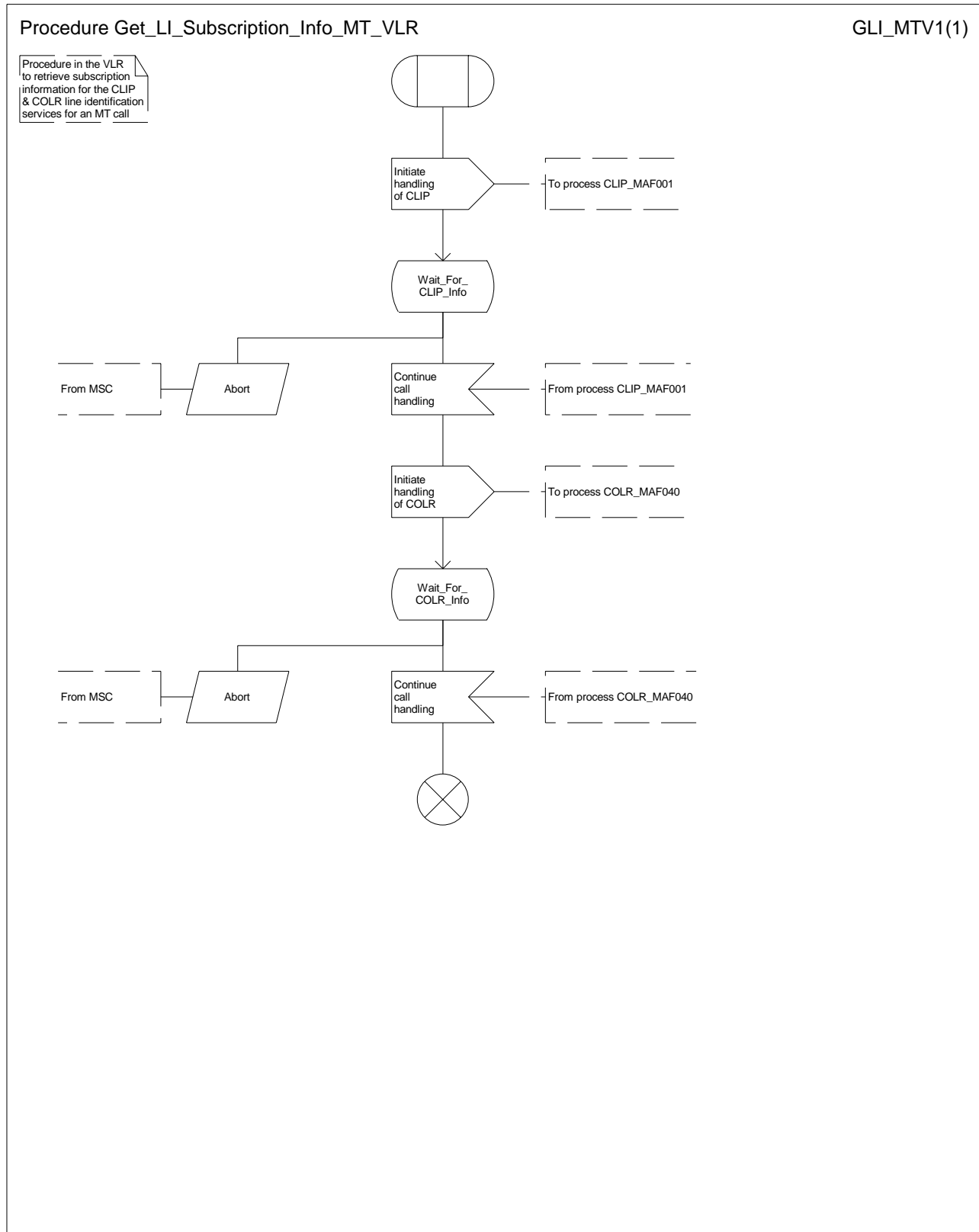
Figure 73: Procedure Get_LI_Subscription_Info_MT_VLR
