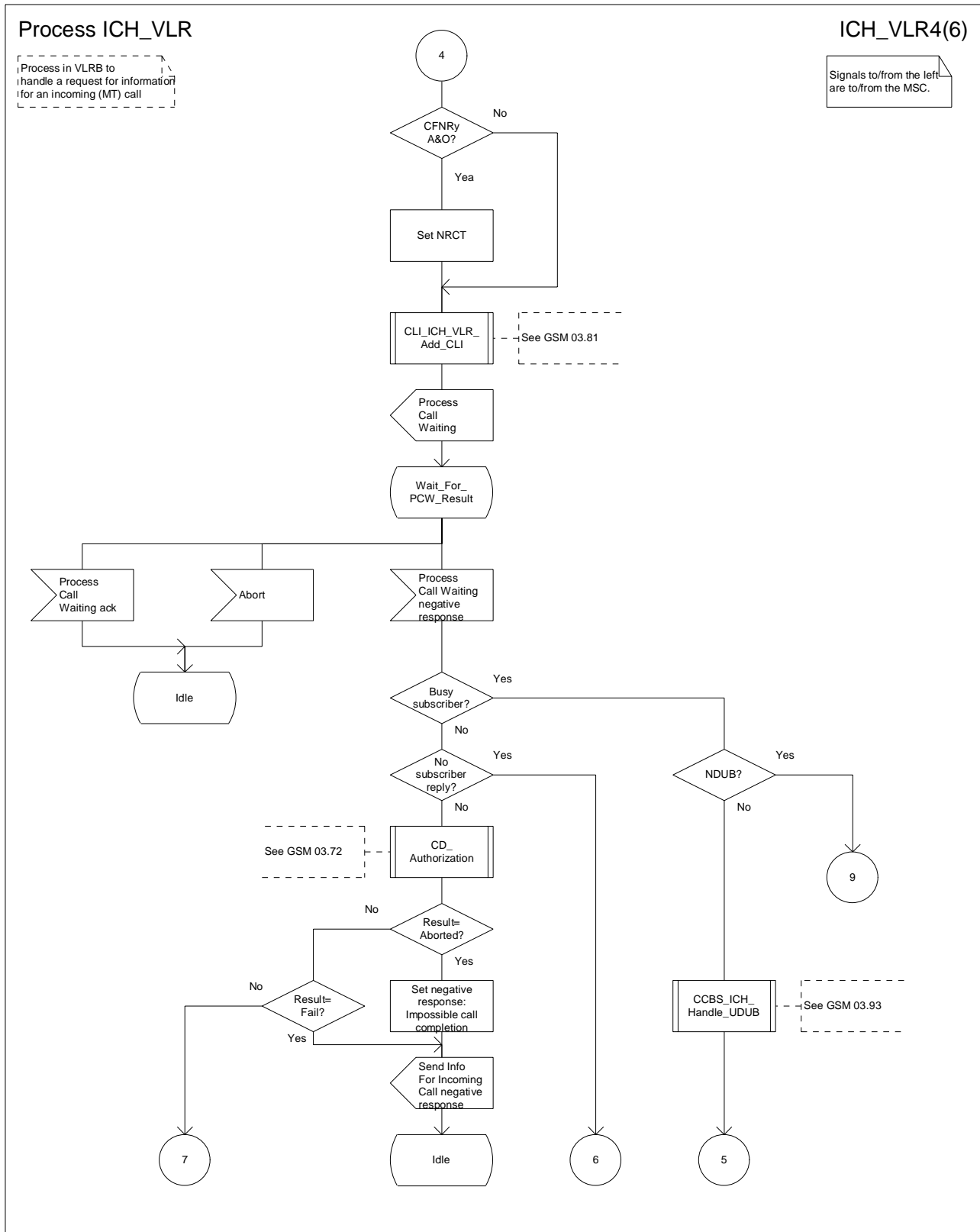
Figure 69d: Process ICH_VLR (sheet 4)
