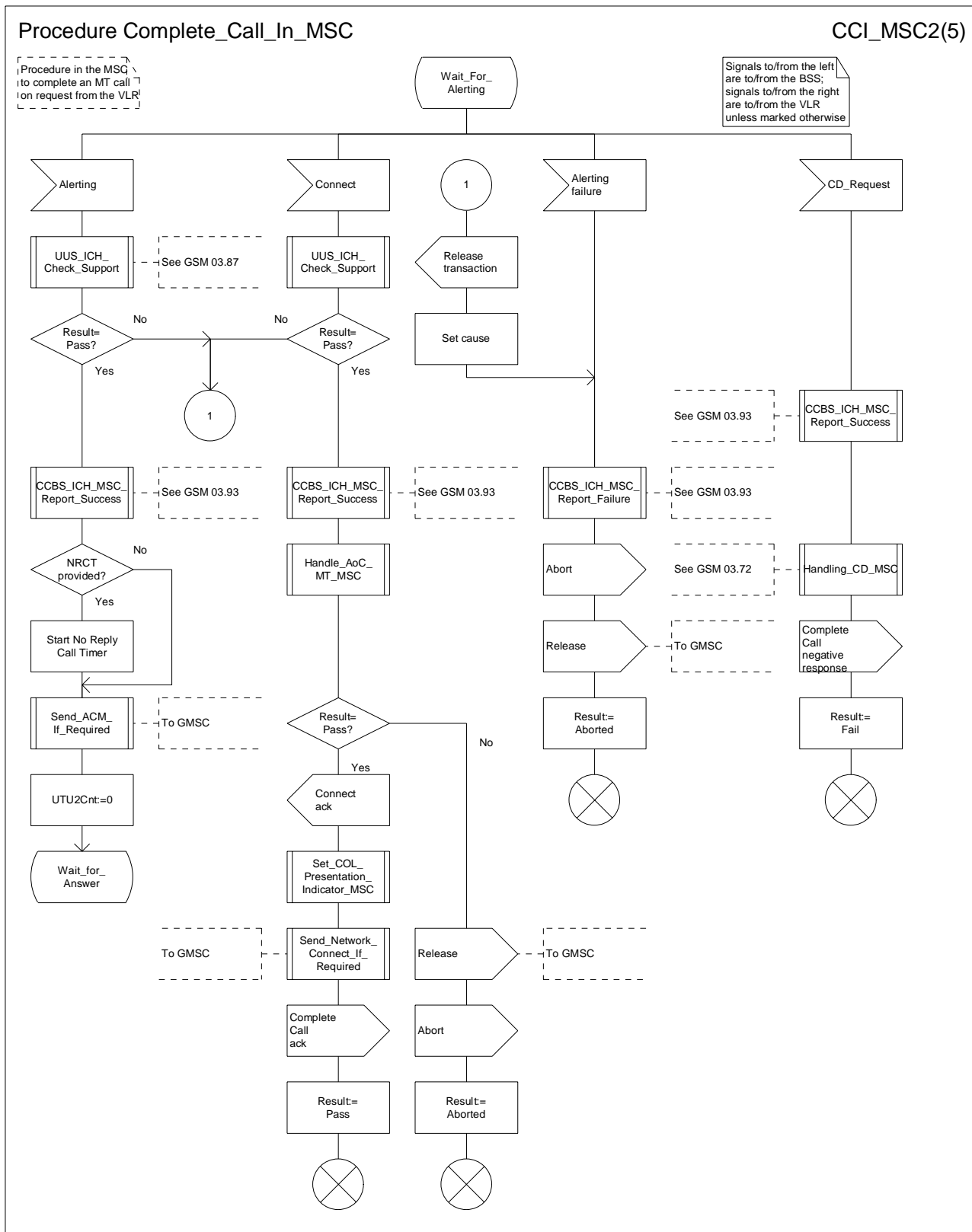
Figure 62b: Procedure Complete_Call_In_MSC (sheet 2)
