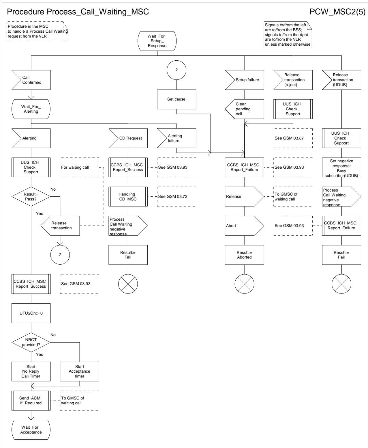
Figure 63b: Procedure Process_Call_Waiting_MSC (sheet 2)
