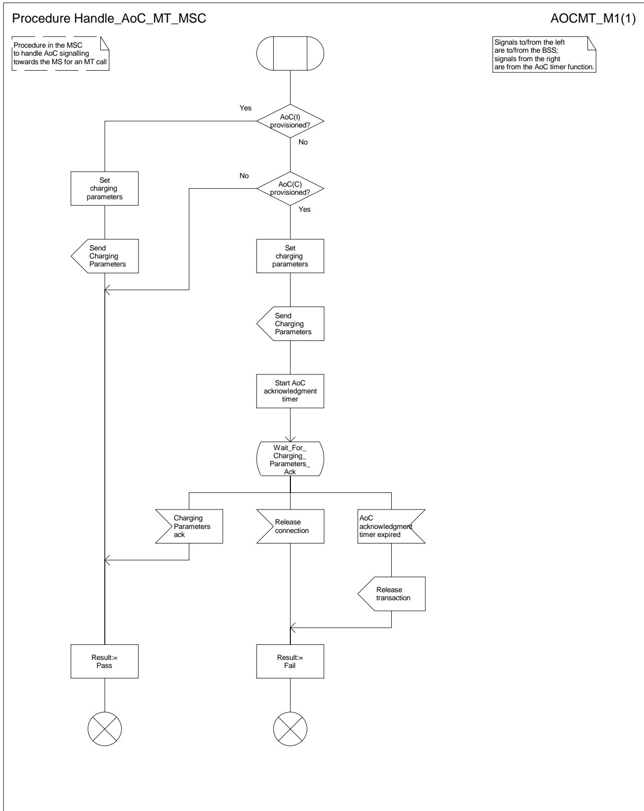
Figure 67: Procedure Handle_AoC_MT_MSC
