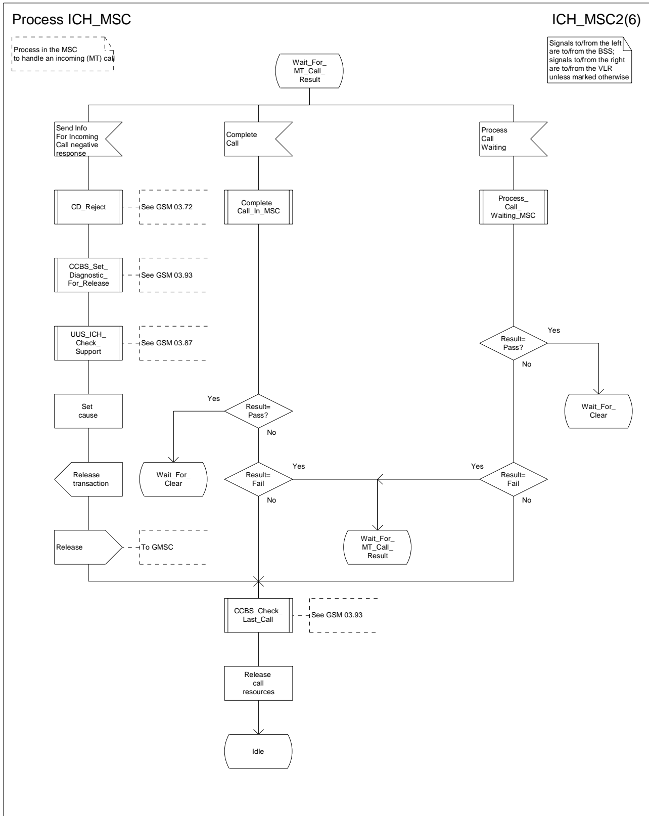
Figure 59b: Process ICH_MSC (sheet 2)
