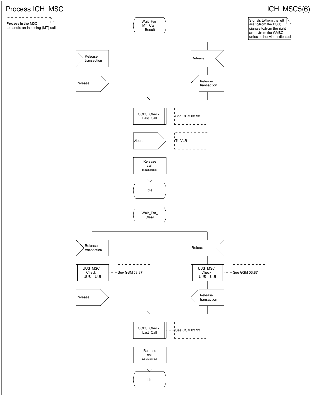
Figure 59e: Process ICH_MSC (sheet 5)
