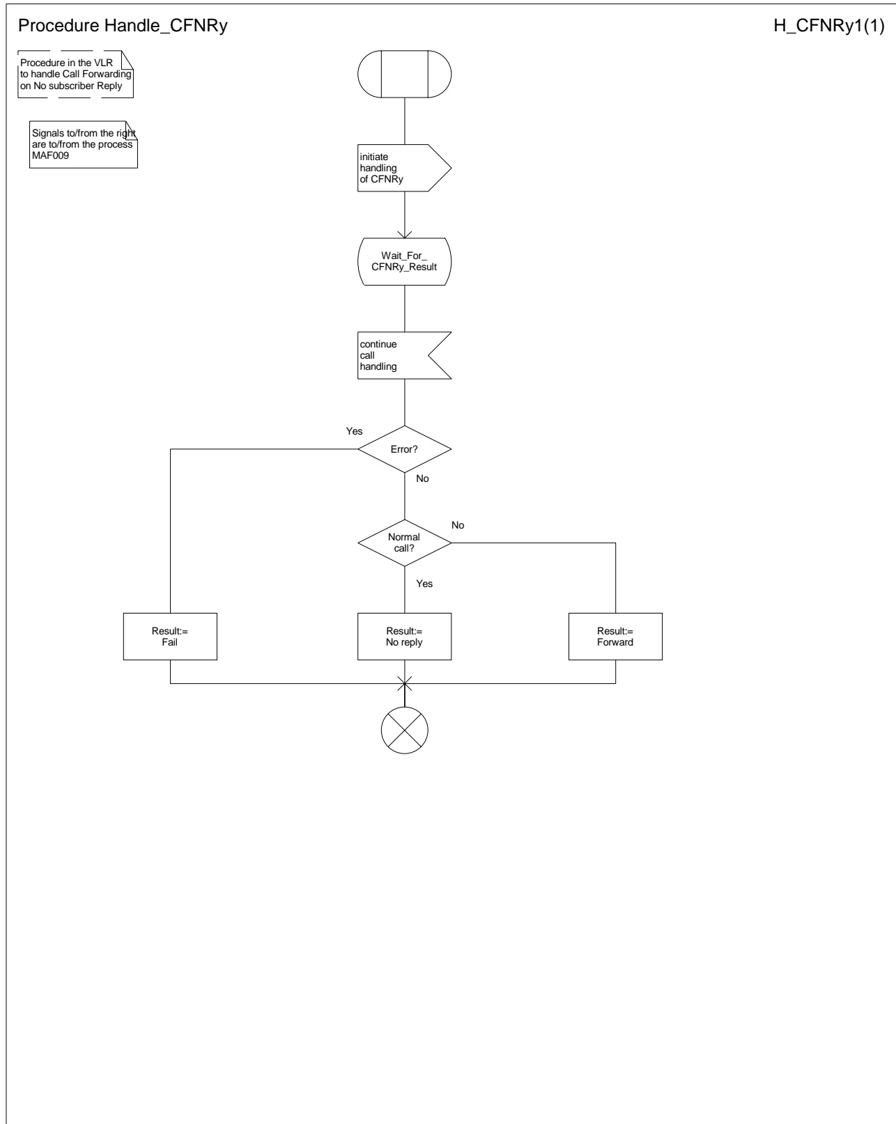
Figure 75: Procedure Handle_CFNRy
