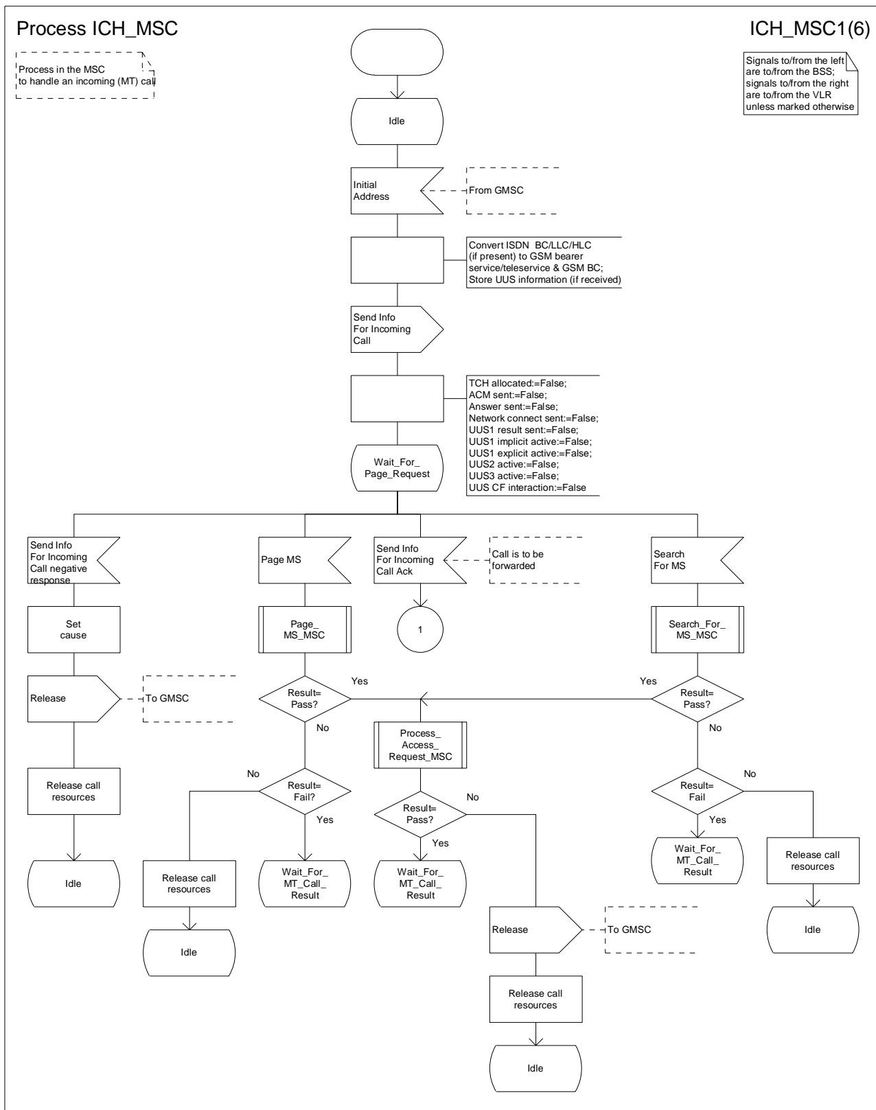
Figure 59a: Process ICH_MSC (sheet 1)
