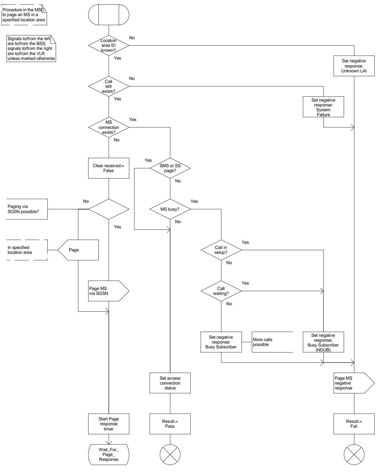
Figure 60a: Procedure Page_MS_MSC (sheet 1)
