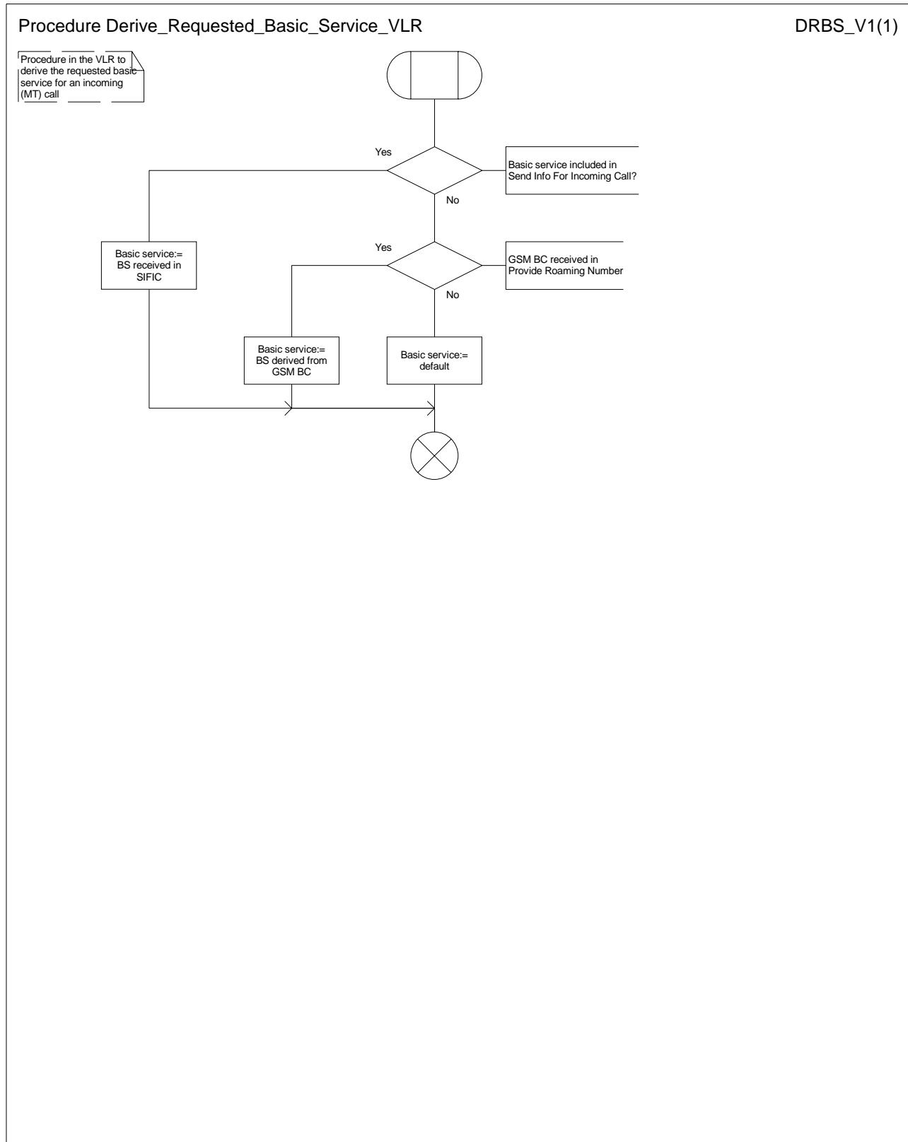
Figure 70: Procedure Derive_Requested_Basic_Service_VLR
