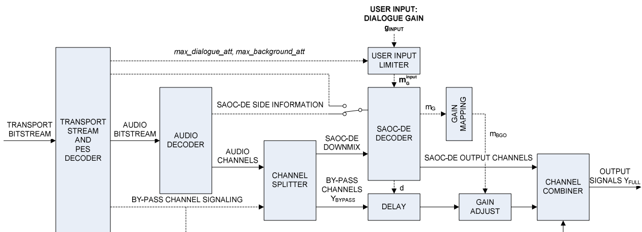
Figure E.6: Multichannel service with Dialogue Enhancement
