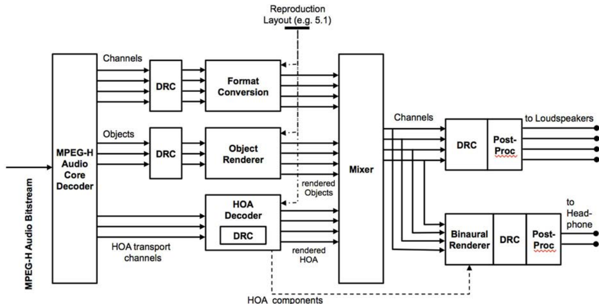
Figure 5: Top level block diagram of the MPEG-H Audio decoder
