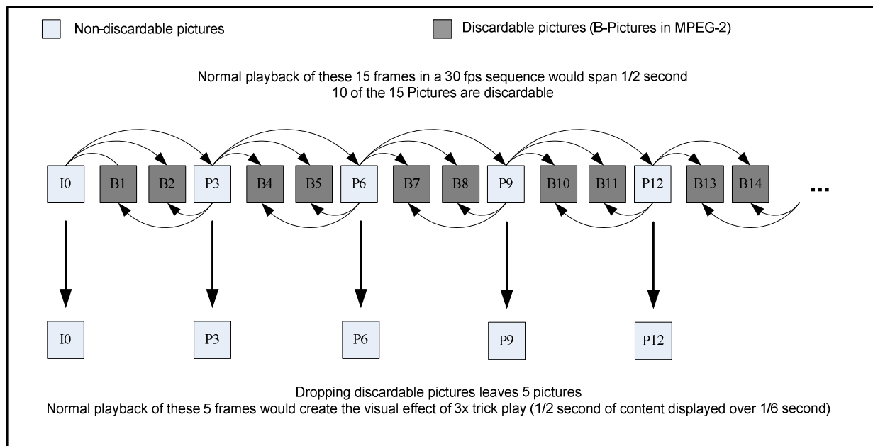
Figure F.1: Example of achieving a 3x trickplay mode from a common MPEG-2 GOP structure (IBBP)
