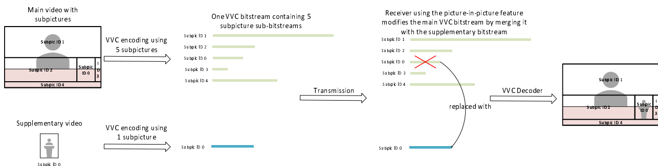
Figure M.6: VVC subpictures for picture-in-picture service
