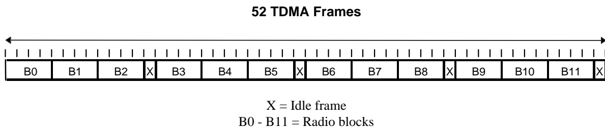
Figure 2a: 52- multiframe for PDCHs
