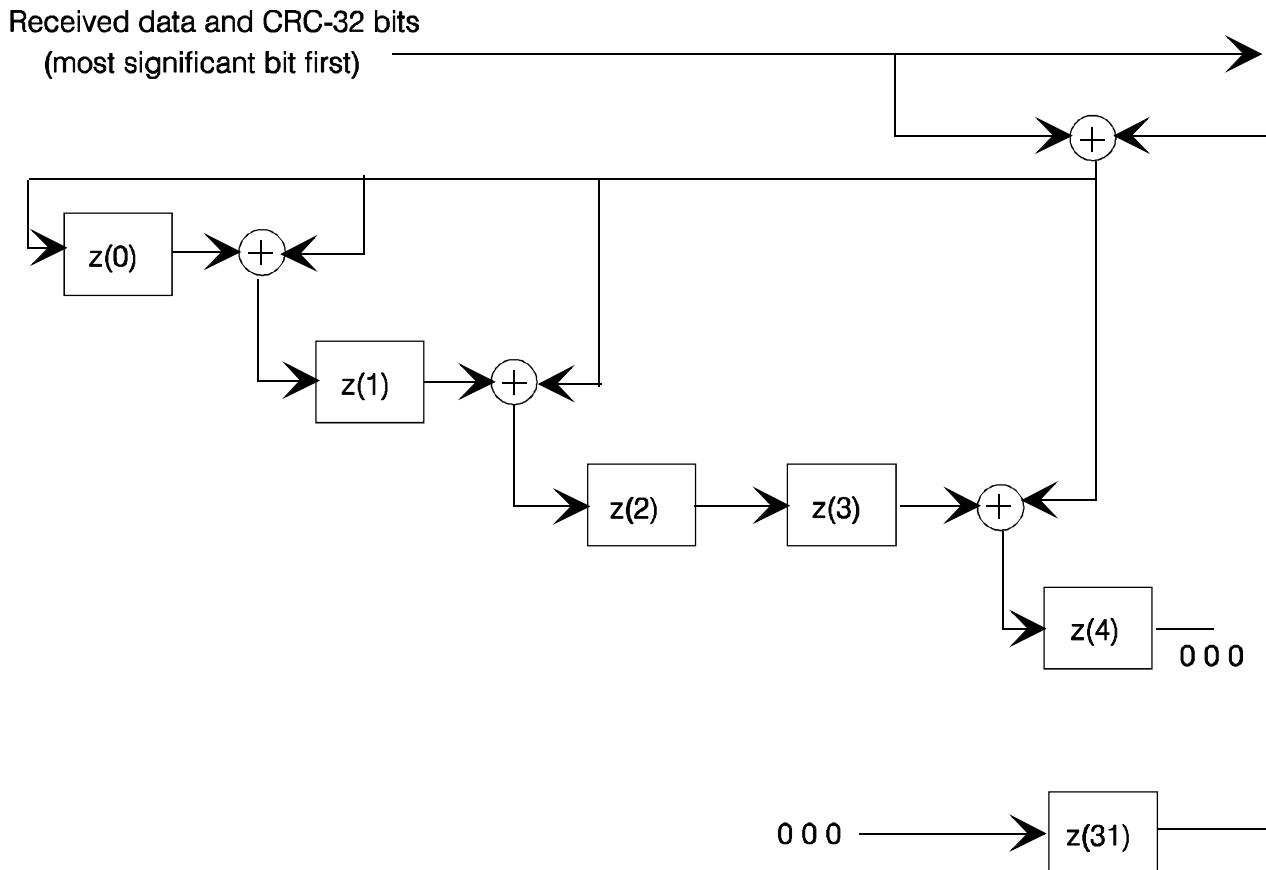
Figure A.1: 32-bit CRC decoder model
