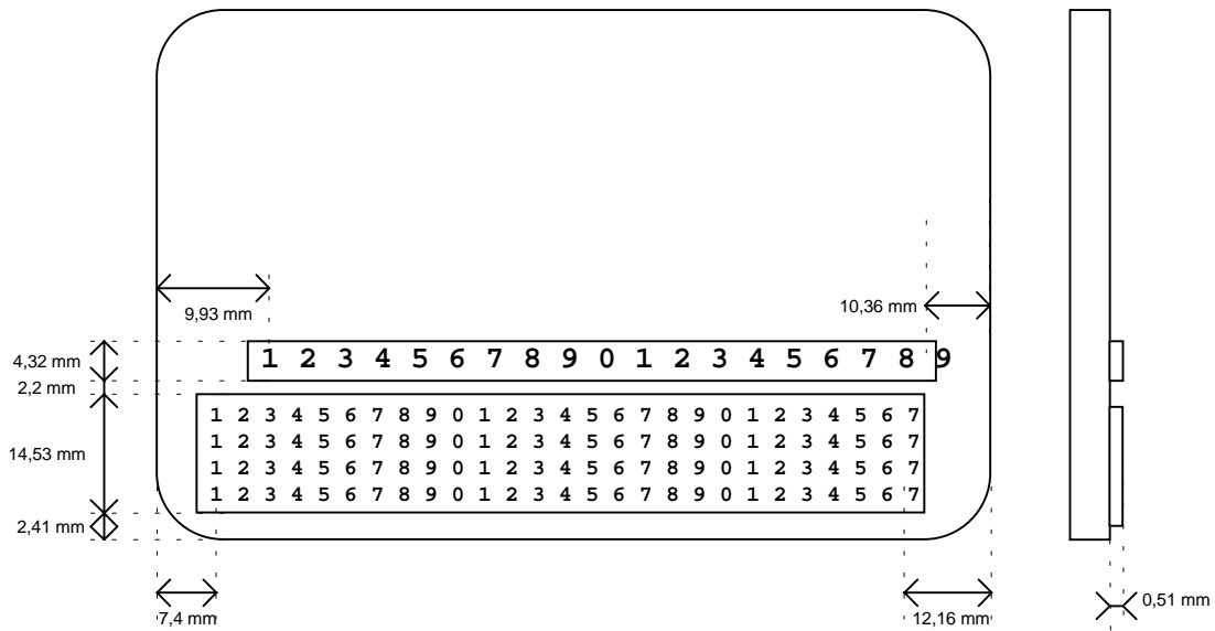
Figure 2: Dimensions of the IC card
