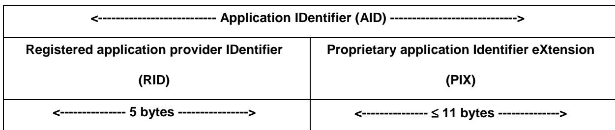
Figure 4.1: AID structure
