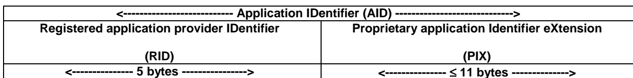
Figure 4.1: AID structure
