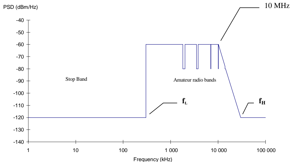
Figure 9: Maximum allowable PSD (Mask M1)
