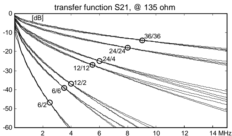
Figure 14: Transmission gain (in 135\ \Omega ) of the test-loops for various payload bit-rates
