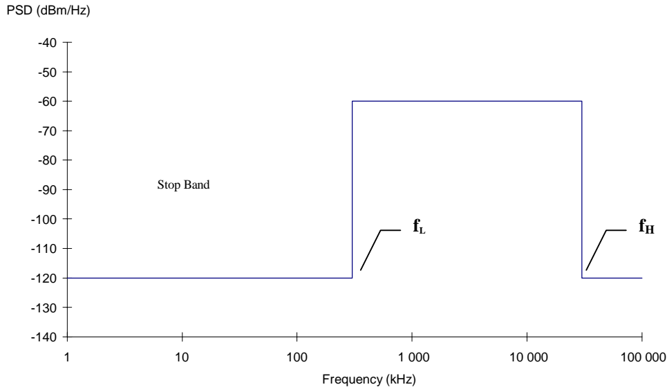
Figure 10: Maximum allowable PSD (Mask M2)
