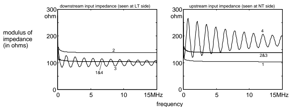
Figure 13: Calculated variation of input impedance, at a normalized loop length of 1 500 m
