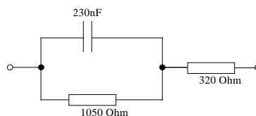
Figure B.3: Z_M compromise reference impedance used by British Telecommunications plc (voice terminals)
