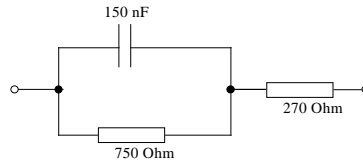
Figure B.1: Z_M compromise reference impedance (European harmonized - non voice terminals)
