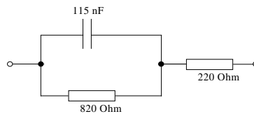
Figure B.2: Z_M compromise reference impedance used by Deutsche Telekom AG (voice terminals)
