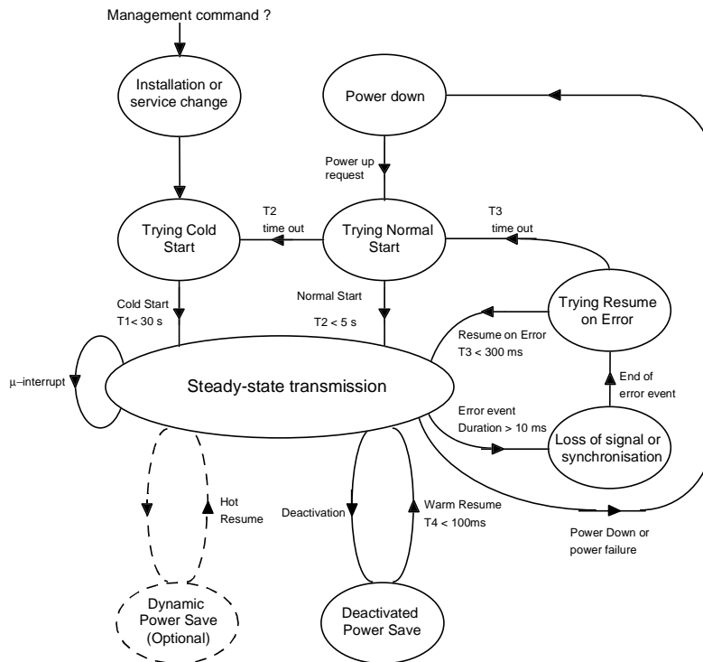
Figure 22: State and timing diagram
