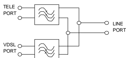
Figure 23: Structure of the VDSL splitter filter
