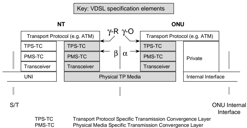
Figure 4: VDSL reference model
