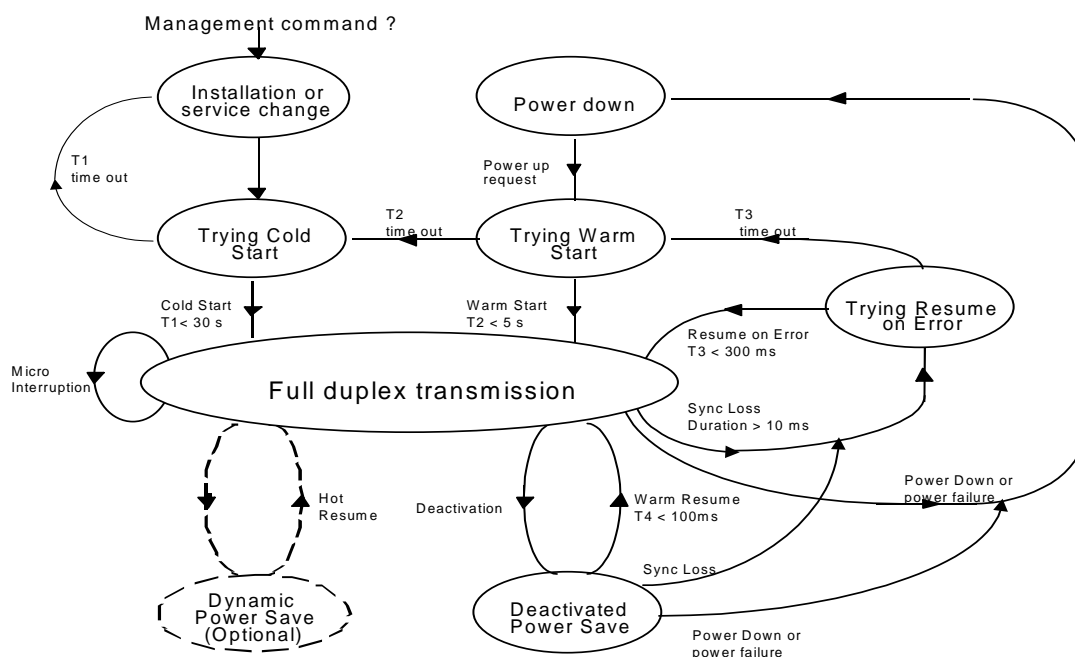
Figure 19: State and timing diagram
