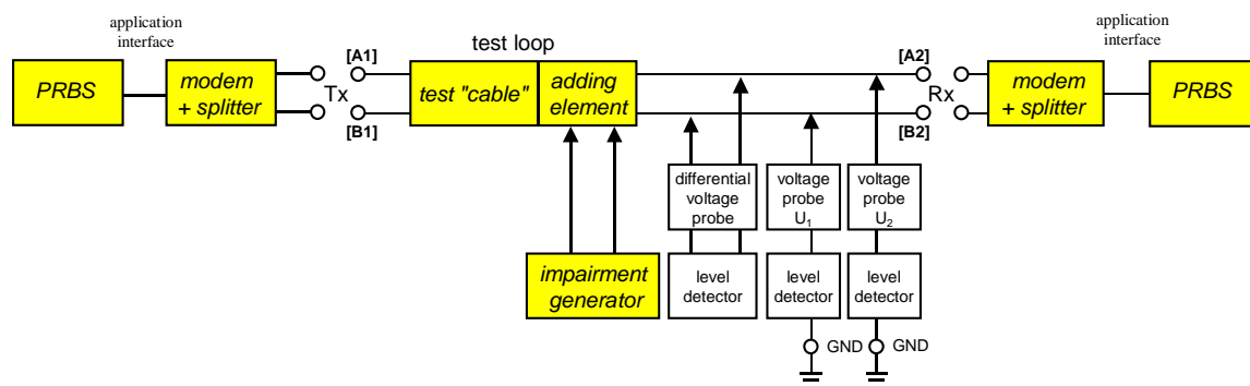
Figure 12: Functional description of the set-up of the performance tests
