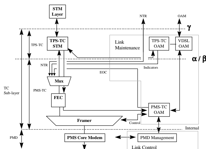
Figure 20: VDSL functional reference model applied to SDH
