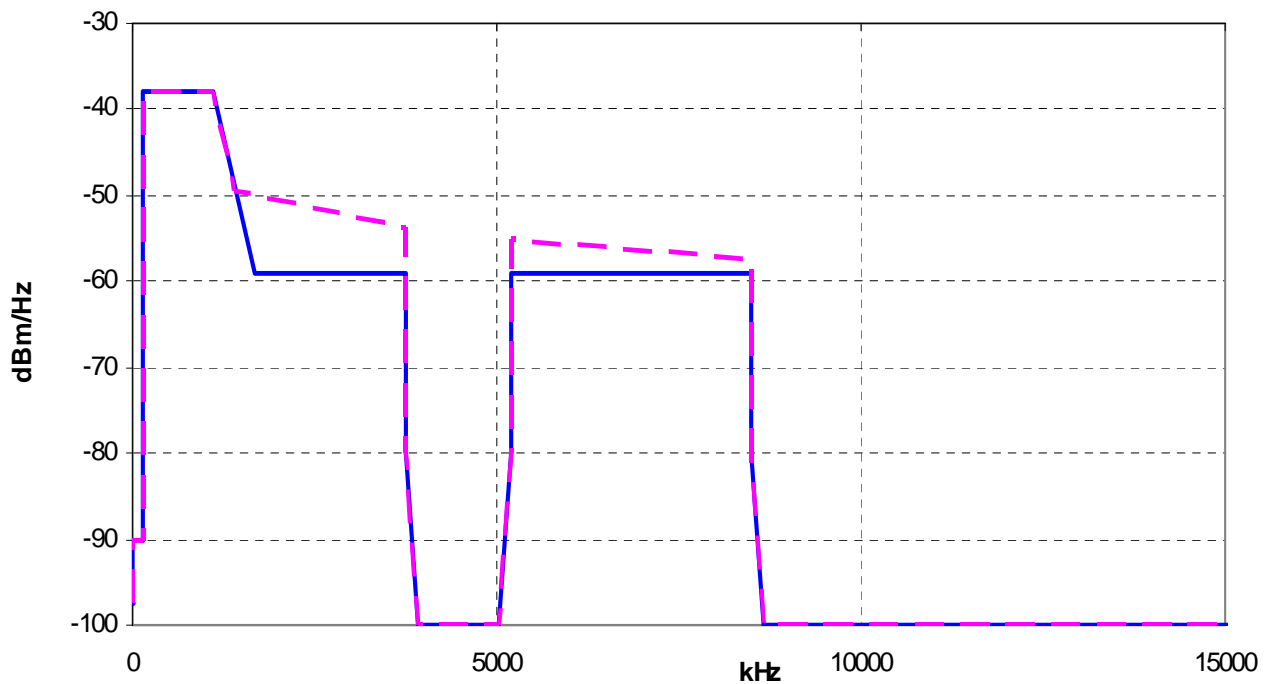
Figure D.8: Regional-specific Pex.P2.M1 (solid line) and Pex.P2.M2 (dashed line)
