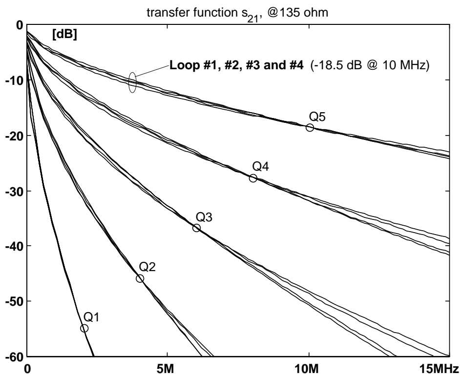
Figure 15: Typical transfer function (in 135 \Omega ) of the test loops when normalized in electrical length
