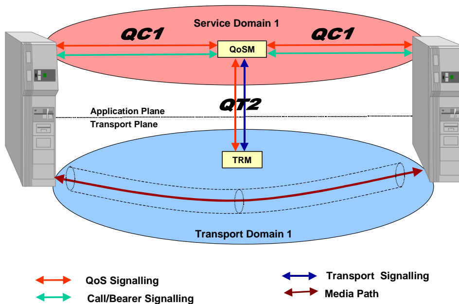
Figure 15: One Service Domain/One Transport Domain
