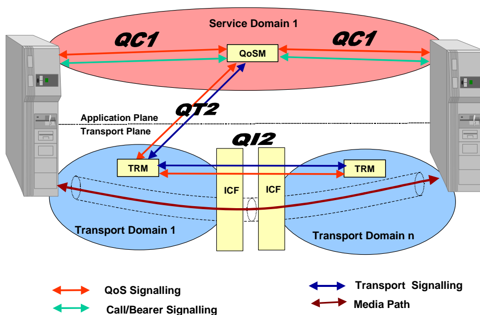
Figure 17: One Service Domain/Multiple Transport Domains - Case II
