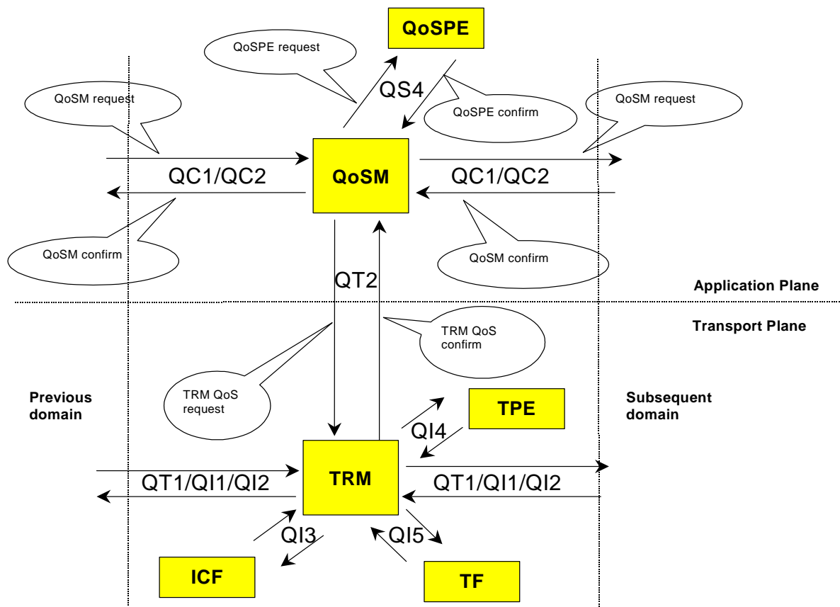
Figure 8: Model of QoS information flows.
