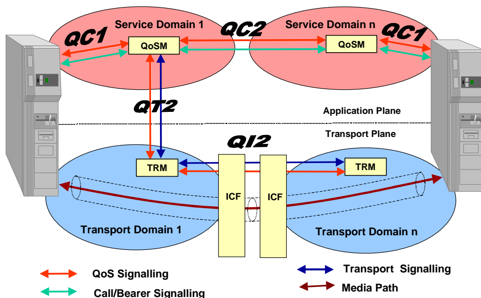
Figure 18: Multiple Service Domains/Multiple Transport Domains - Case I
