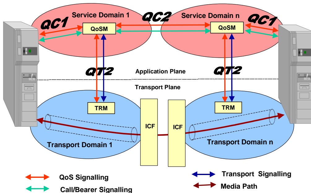
Figure 19: Multiple Service Domains/Multiple Transport Domains - Case II
