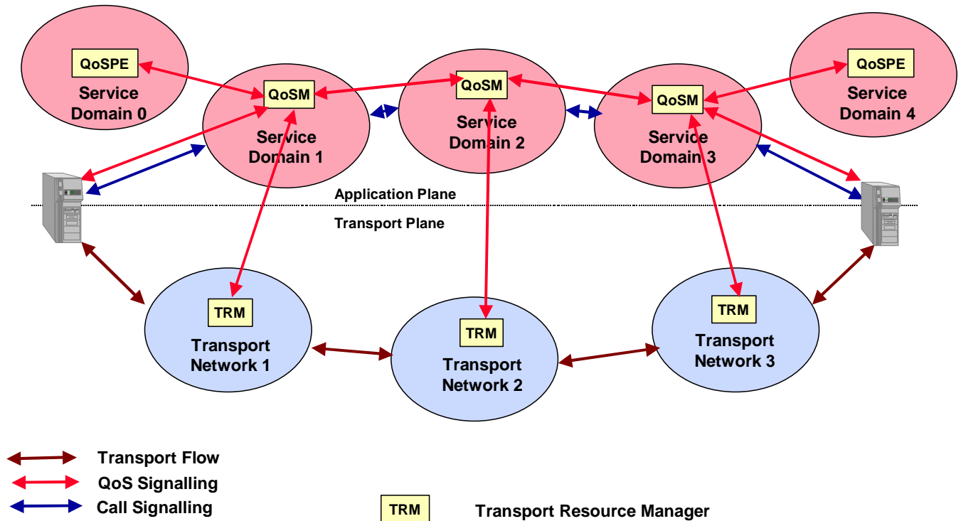
Figure 20: Multiple Service Domains/Multiple Transport Domains - Roaming
