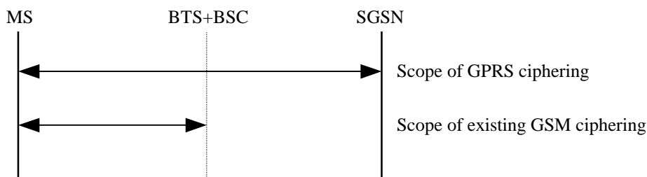
Figure 25: Scope of GPRS Cipherng
