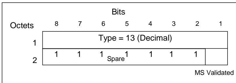
Figure 18: MS Validated information element
