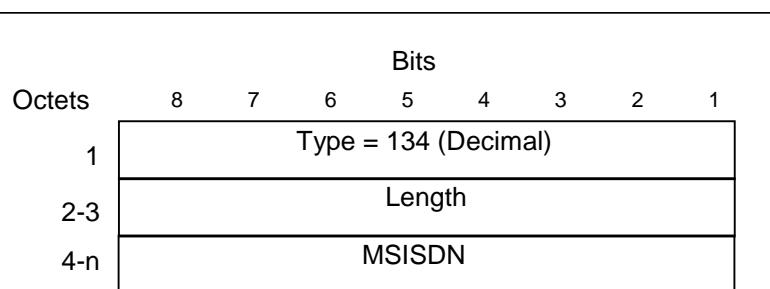
Figure 34: MSISDN information element
