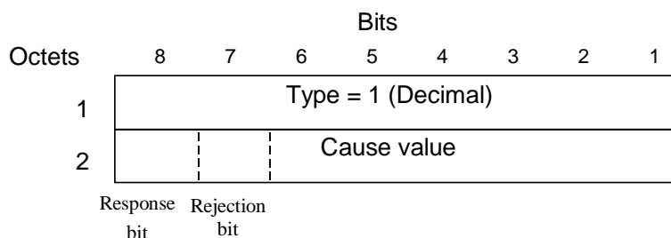
Figure 8: Cause information element
