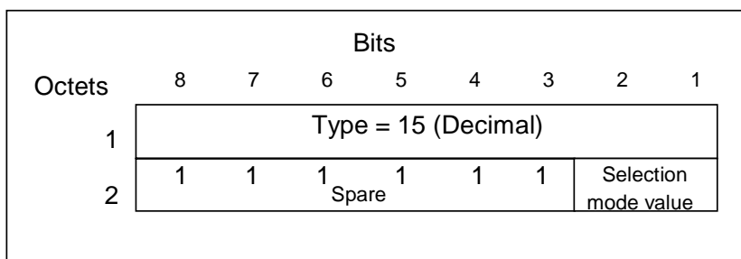
Figure 20: Selection mode information element
