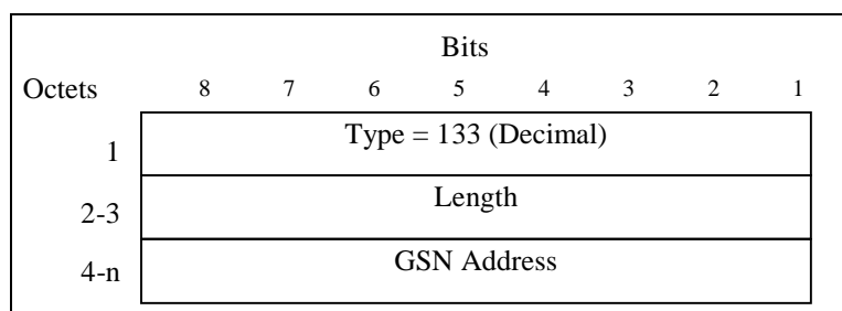
Figure 33: GSN Address information element
