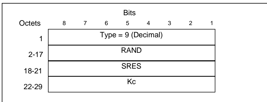
Figure 15: Authentication Triplet information element
