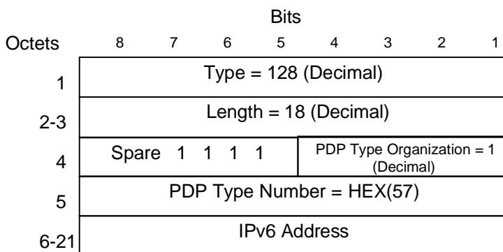
Figure 27: End User Address information element for IPv6
