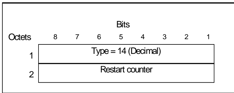
Figure 19: Restart counter information element
