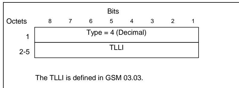
Figure 11: TLLI information element
