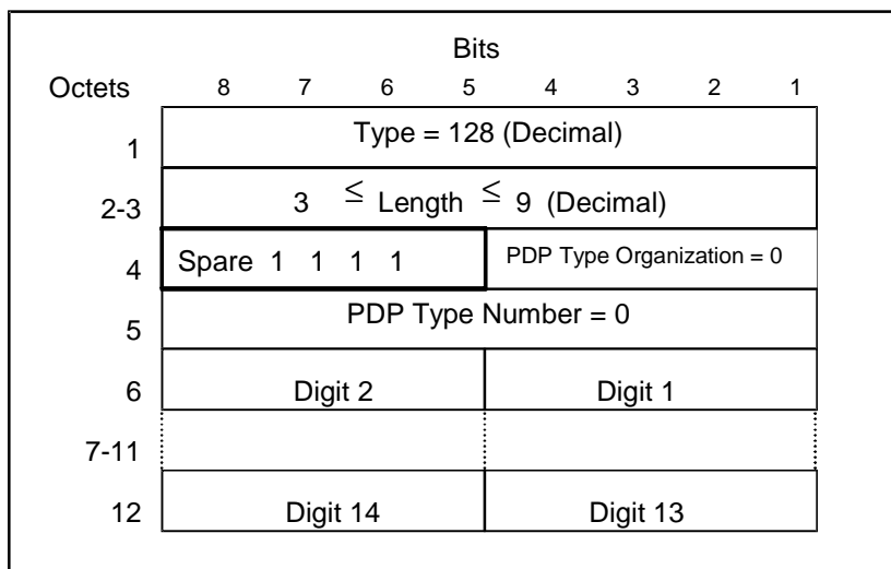
Figure 28: End User Address information element for X.25
