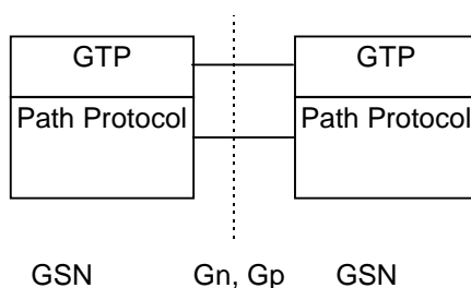
Figure 4: Signalling Plane - Protocol stack
