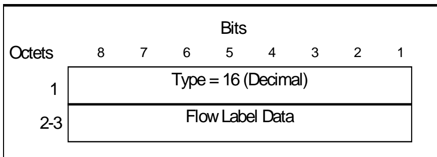
Figure 21: Flow Label Data information element
