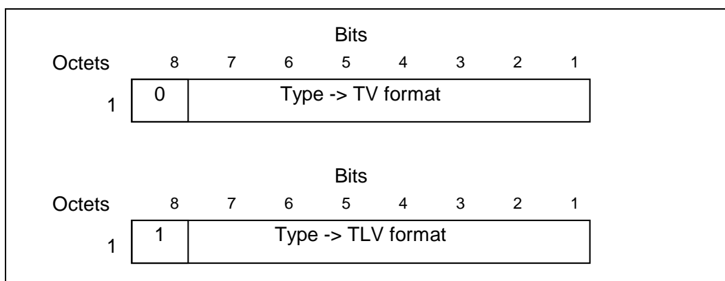
Figure 7: Type field for TV and TLV format
