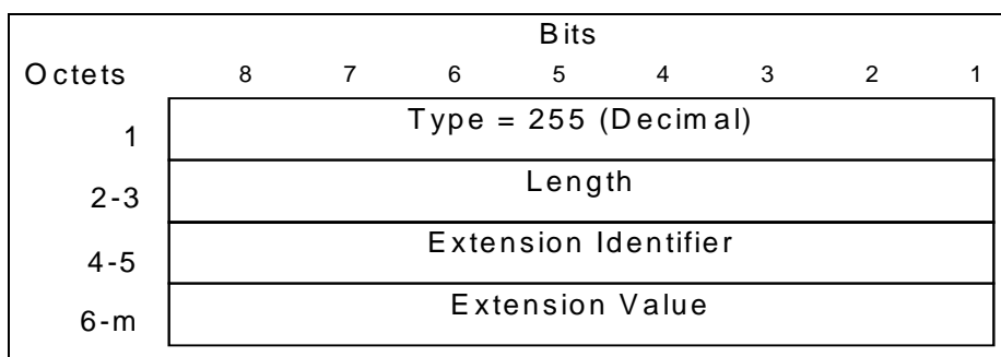
Figure 35: Private Extension information element
