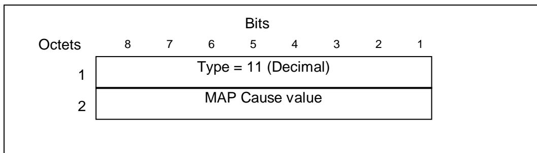
Figure 16: MAP Cause information element
