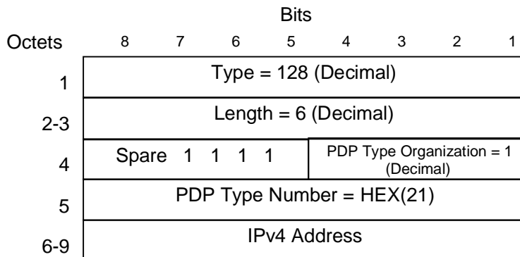
Figure 26: End User Address information element for IPv4
