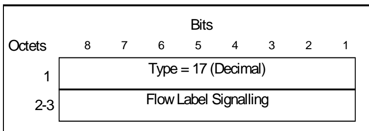
Figure 22: Flow Label Signalling information element
