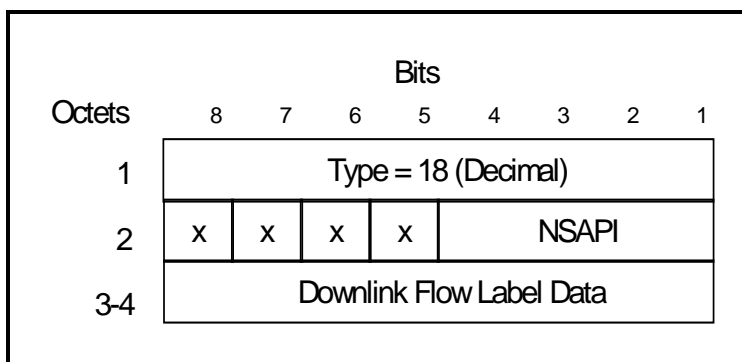
Figure 23: Flow Label Data II information element
