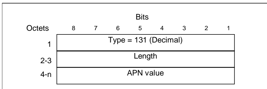
Figure 31: Access Point Name information element
