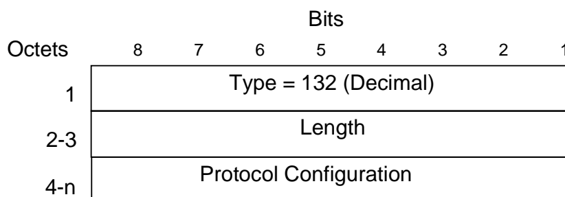
Figure 32: Protocol Configuration Options information element
