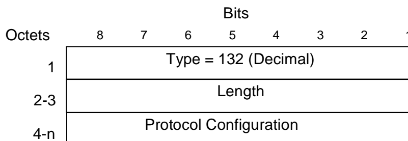
Figure 32: Protocol Configuration Options information element
