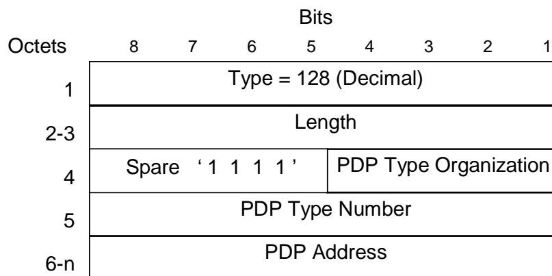
Figure 25: End User Address information element
