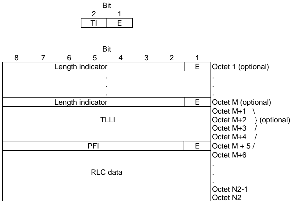
Figure 11: Uplink EGPRS RLC data block
