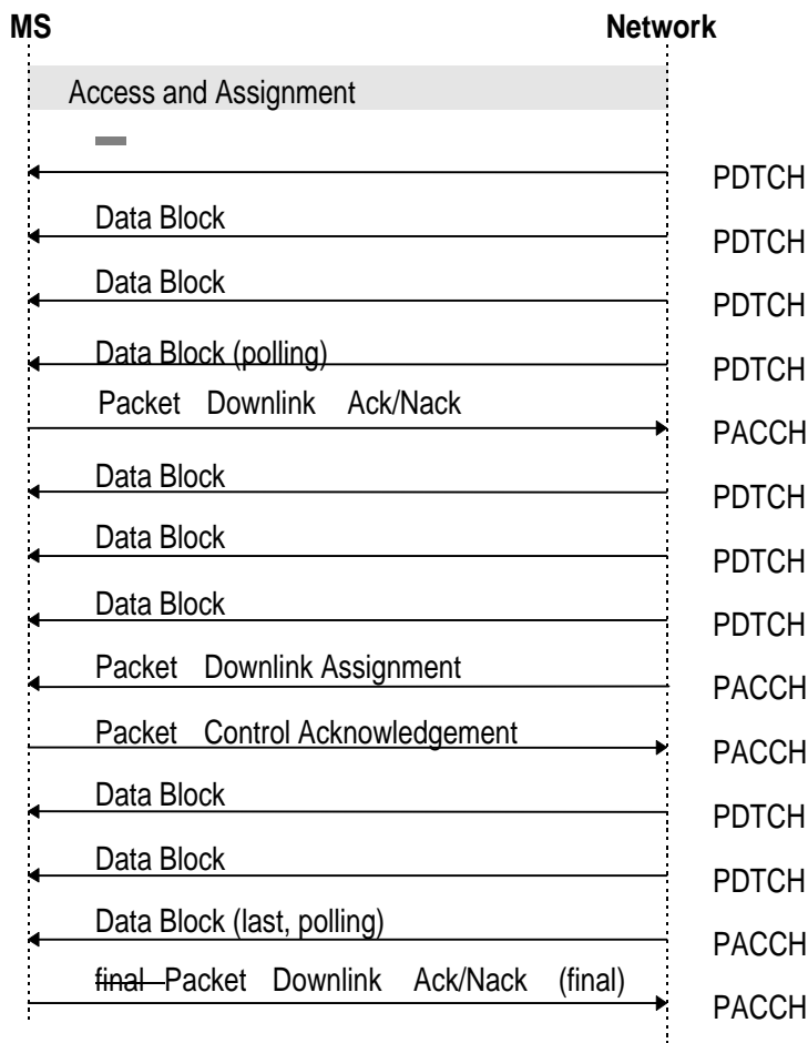
Figure 13: An example of downlink data transfer
