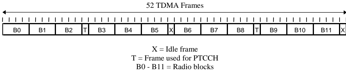
Figure 2: Multiframe structure for PDCH
