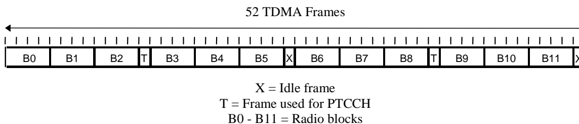
Figure 2: Multiframe structure for PDCH
