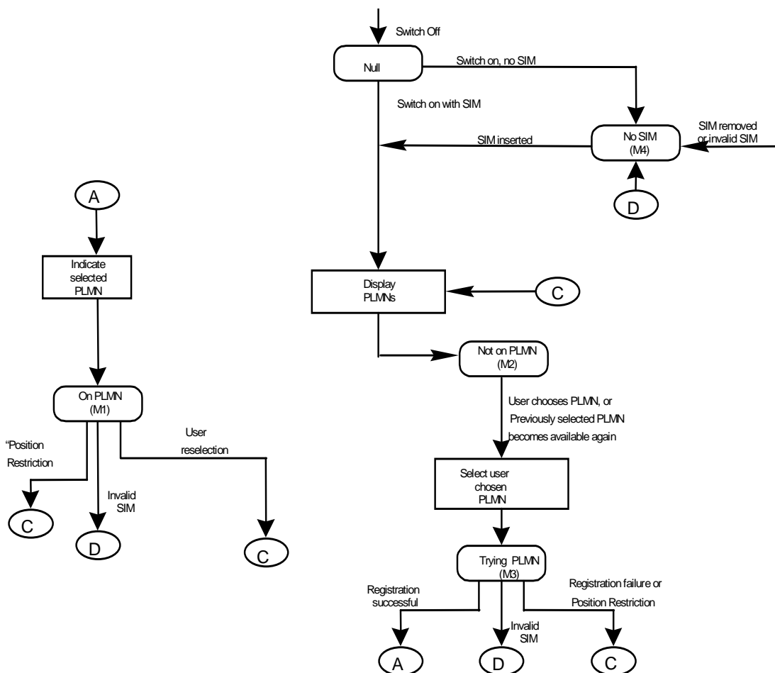
Figure 6.4: PLMN selection state diagram (manual mode)
