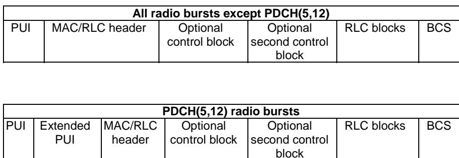
Figure 4: Radio burst structures for data transfer for GMPRS-1
