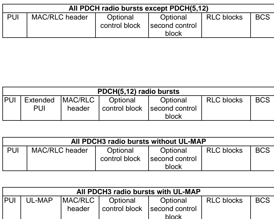
Figure 4: Radio burst structures for data transfer for GMR-1 3G
