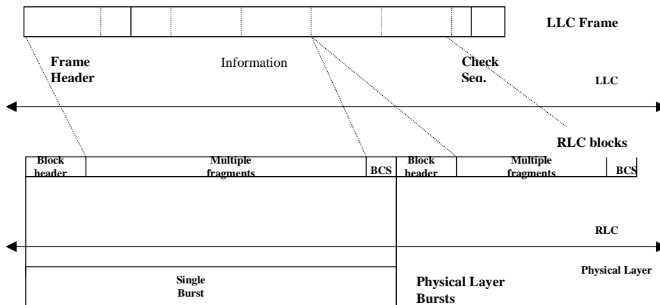
Figure 6: Transmission and reception data flow for GMR-1 3G
